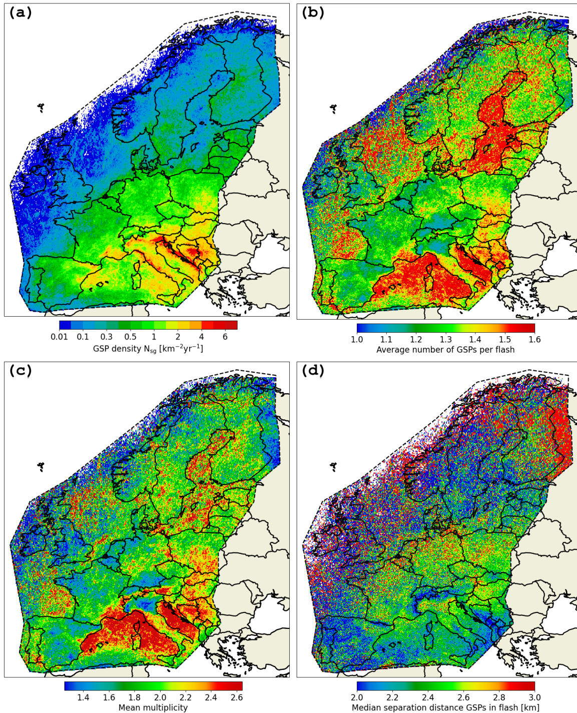
Figure 2: Spatial distribution of the (a) mean annual ground strike point density N_{SG} [ \text{km}^{-2} \text{yr}^{-1} ], (b) average number of GSPs per flash (GSPF), (c) mean multiplicity, and (d) median separation distance amongst GSPs in a flash.
