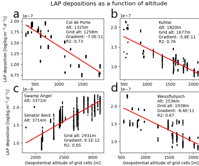
Figure 9. Local gradient of the total LAP climatological deposition rate with elevation and associated linear regression at (a) Col de Porte, (b) Kūhtai, (c) Swamp Angel and Senator Beck, and (d) Weissfluhjoch. Note that the axes are not identical between the plots. The gradients have the units \text{kg m}^{-2} \text{d}^{-1} .
