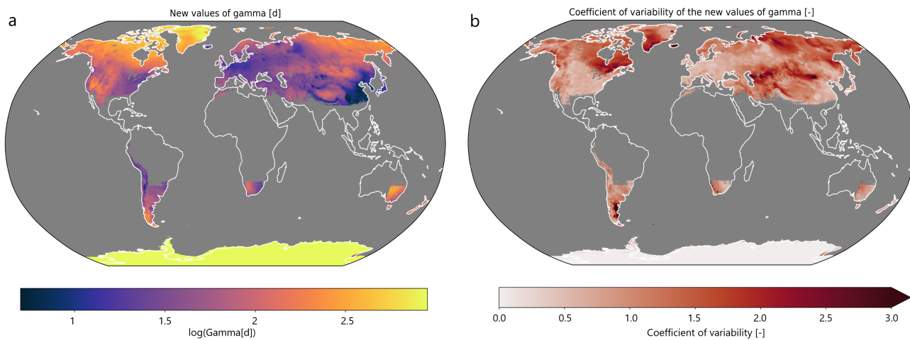
Figure 13. Global maps showing (a) the optimal value of \gamma derived from Eq. 10 and (b) the coefficient of variability of \gamma associated with the inter-annual variability of LAP deposition on snow.
