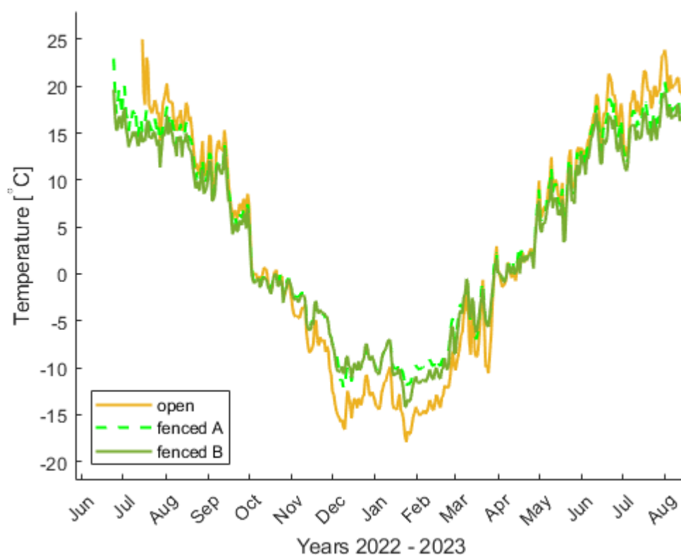
Figure 13: Daily ground surface temperature from the loggers placed in Udleg. Note that GST are measured at fenced plot A and B from 24. June 2022, while the open plot was added on the 15. July 2022. The GST evolution of the individual loggers is presented in Fig. B2.
