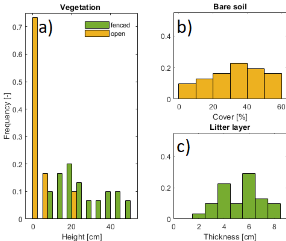
185 Figure 3: Observations from the vegetation survey in the Terelj site on 17. August 2023 (n=30 in each plot). a) Distribution of vegetation height in the open (median = 3cm) and fenced plot (median = 20 cm). b) Distribution of bare soil fraction at the open plot (median = 30%). c) The thickness of intact litter layers covering the ground surface at the fenced plot (median = 6 cm). For readability, the bars in a) are plotted next to each other within each 5 cm interval.
