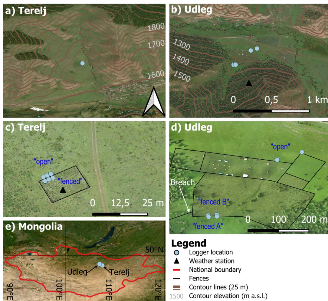
105 Figure 1: Overview showing the location of the temperature loggers in Terelj (a & c) and Udleg (b & d), and the location of our study sites within each site is indicated by blue text in c) and d), while the white arrow shows the location of the fence breach in 2022. All figures are oriented with North facing up, and a) and b) have the same scale. Background: a), b) and e) Satellite imagery (ESRI, 2023), c) and d) drone-based orthomosaic acquired on 17. and 15. August 2023, respectively, and processed in Agisoft Metashape (Agisoft LLC, 2023).
