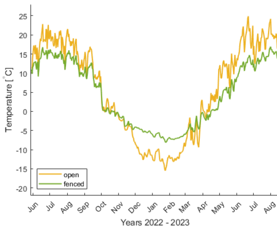
275 Figure 11: Average daily ground surface temperature for the plots in Terelj. The GST evolution of the individual loggers is presented in Fig. B1.
