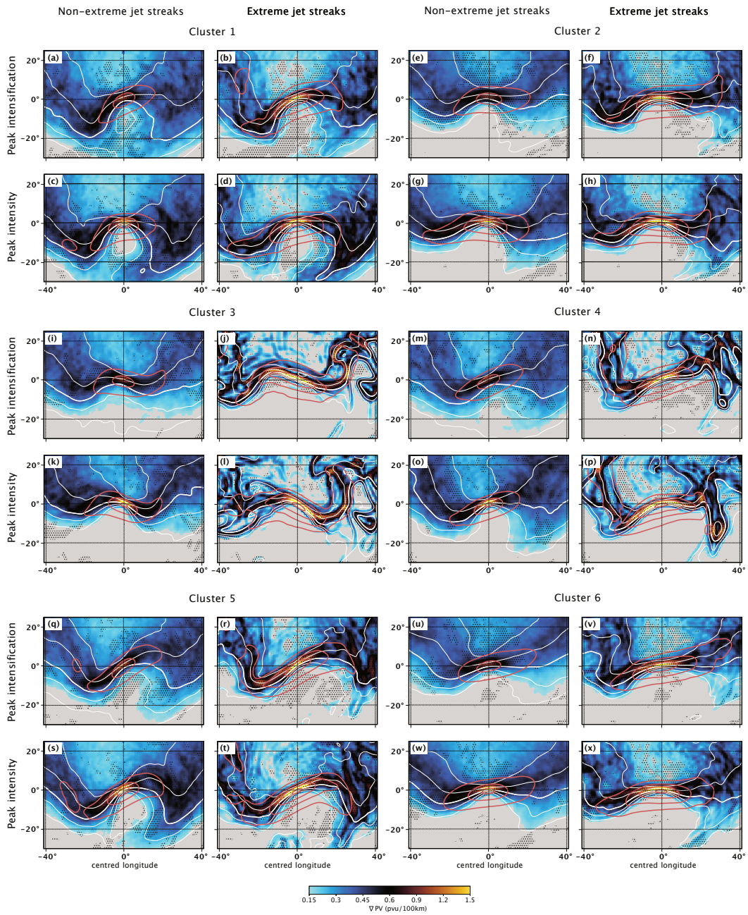
Figure G5. Colours: PV gradient (PVU (100 km) -1 ), values smaller than 0.15 PVU (100 km) -1 are white. Dotted areas indicate where the difference between the mean of PV gradients on central jet streak isentropes of non-extreme and extreme jet streaks is robust. Contours: White: PV on central isentropes, bold blue : 2 PVU, red: wind speed on central isentropes, every 10 m s -1 , starting at 40 m s -1 . Order of panels as in Figure G1.
