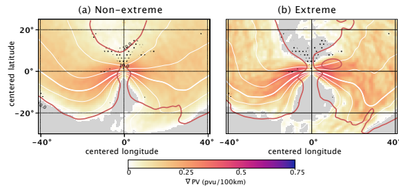
Figure C1. As for Fig. 15, but with the standard deviation of PV gradient instead of PV. Contours: White: PV on central isentropes, 2 PVU, black red : standard deviation of wind speed on central isentropes, every 10 \text{ m s}^{-1} , starting at 10 \text{ m s}^{-1} , white dashed in (b): 2 PVU isolines for all central isentropes of extreme jet streaks at peak jet streak intensity.
