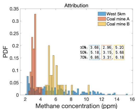
619 Figure 16. Probability density functions (PDF) of CH 4 concentrations (a) observed at the wet 5km site (blue), 620 and concentrations simulated by the 2-box model resulting from emissions attributed to (b) Coal mine A (red), 621 and (c) Coal mine B (orange). The respective 30 th , 50 th , and 70 th percentiles of the distributions are given in 622 text, outlined by the corresponding color box.
