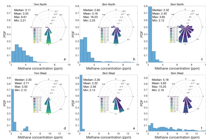
Figure 12. Probability density map for \text{CH}_4 concentration and wind rose measured at 1 km north (a), 1 km west (d), 3 km north (b), 3 km west (e), 5 km north (c), and 5 km west (f) of CM-A and corresponding wind rose chart.
