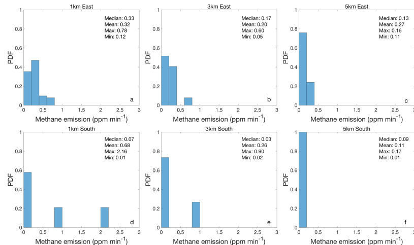
Figure 15. Probability density functions (PDF) of \text{CH}_4 emissions located at 1 km east (a), 3 km east (b), 5 km east (c), 1 km south (d), 3 km south (e), and 5 km south (f) of CM-A, including median, mean, maximum, and
