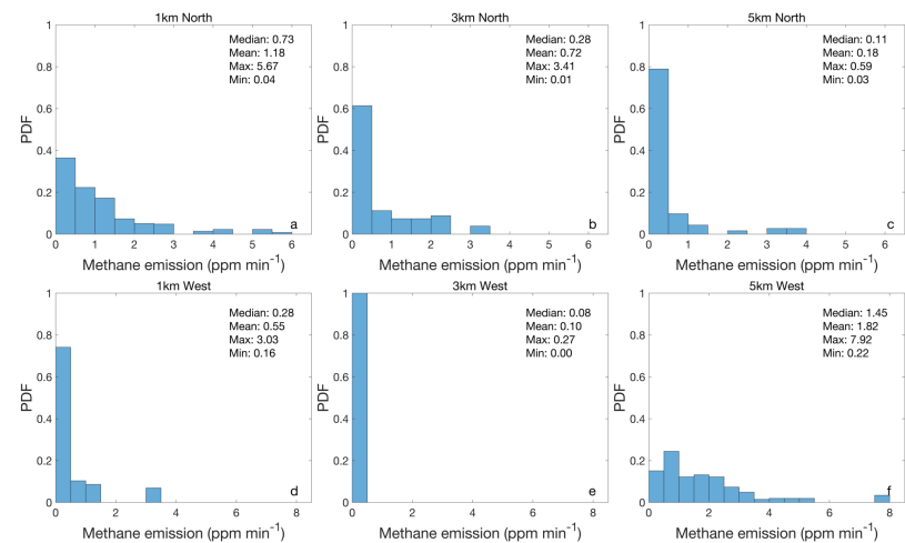
Figure 14. Probability density functions (PDF) of \text{CH}_4 emissions located at 1 km north (a), 3 km north (b), 5 km north (c), 1 km west (d), 3 km west (e), and 5 km west (f) of CM-A, including median, mean, maximum, and minimum statistics.
