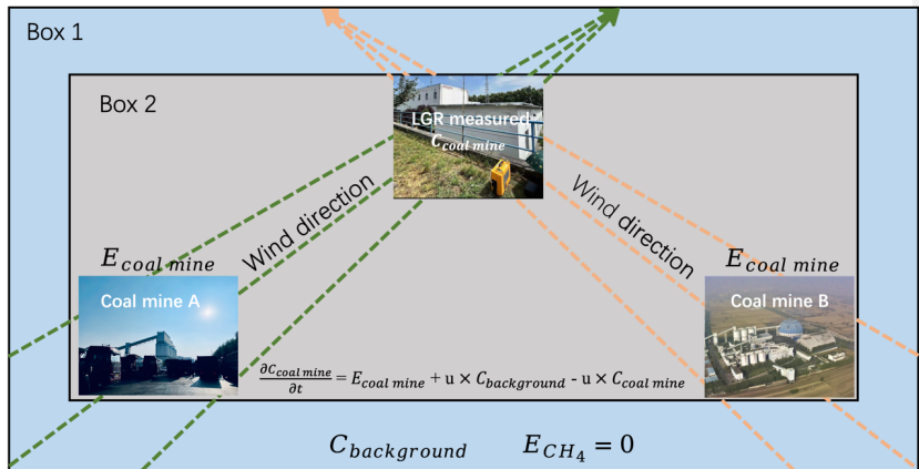
Figure 8. Schematic diagram of the 2-Box model.
