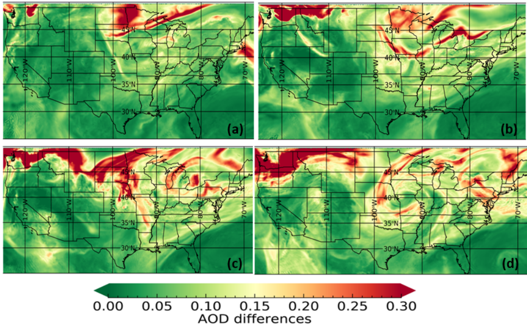
Fig. 2. AOD change due to Canadian wildfires from August 17th to 20th, 2018: (a) August 17th, 2018; (b) August 18th, 2018; (c) August 19th, 2018; (d) August 20th, 2018. The AOD change is calculated using the difference of two WRF-Chem simulations.
