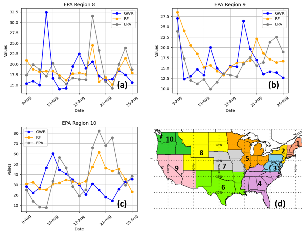
Fig. 12. Mean PM 2.5 concentration variations over the top 3 polluted areas (a) EPA region 8 (b) EPA region 9 (c) EPA region 10 (d)EPA region map
