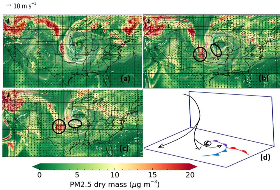
Fig. 6. PM2.5 dry mass distribution on August 20th, 2018 at different levels (a) 773hPa (b) 850hPa (c) 900hPa (d) conceptual model of airflow patterns in a typical extratropical cyclone based on (Cotton et al., 2011).
