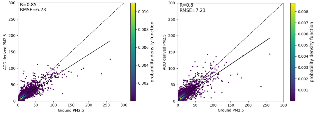
Fig. 10. Fitting and 100-fold cross validation results for GWR method
