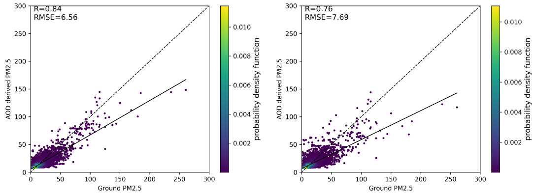
Fig. 11. Fitting and 100-fold cross validation results for RF method
