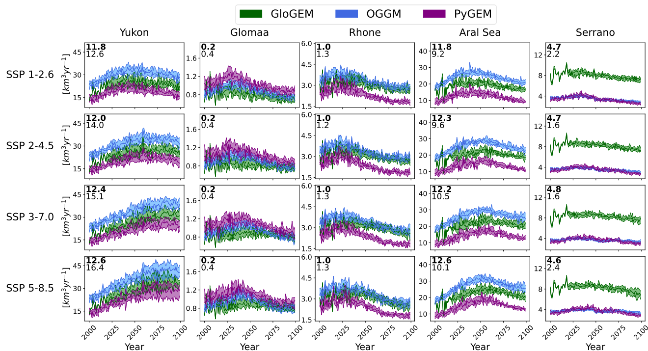
Figure 2. Projected multi-GCM median annual glacier runoff for each glacier model and SSP for selected basins: Yukon basin (North America), the Glomaa basin (Europe), the Rhone basin (Europe), the Aral Sea basin (Asia), and the Serrano basin (South America). The shaded area shows the interquartile range of the 12 single-GCM projections. Annotations on each figure panel state the multi-glacier-model range ( n=3 , bold text) and multi-GCM range ( n=12 ) of projections, both in \text{km}^3\text{yr}^{-1} , computed following Sect. 2.2.
