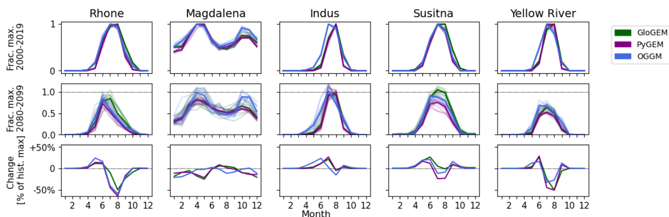
Figure 5. Variability in relative monthly glacier runoff for each glacier model for five example basins over 2000–2019 (top row), 2080–2099 (middle row), and the change between these two periods (bottom row). Monthly glacier runoff for 2000–2019 and 2080–2099 is normalized by the maximum monthly runoff over the 2000–2019 period, computed for each glacier model and GCM individually. The percent change over the two time periods is expressed as a percentage of the 2000–2019 maximum monthly runoff, shown only for the multi-GCM median. Heavier lines show multi-GCM median for each glacier model; light lines show individual GCMs. Results for all basins are shown in Figures A2– A3.
