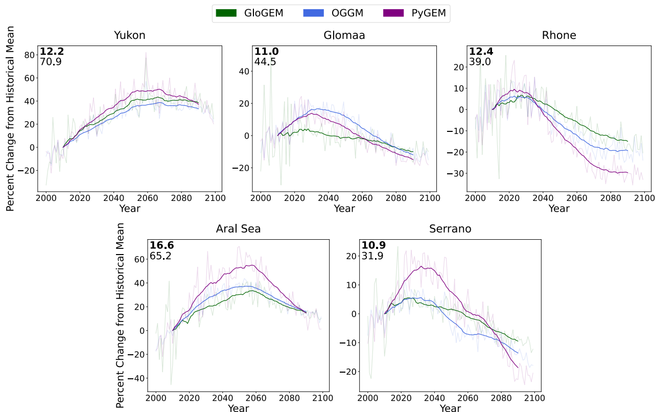
Figure 3. Smoothed (20 year rolling mean) annual multi-GCM median glacier runoff projections as a percent change relative to the historical (2000–2019) average under SSP 2-4.5. The multi-glacier-model and multi-GCM range are given as in Fig. 2, however, in units of %.
