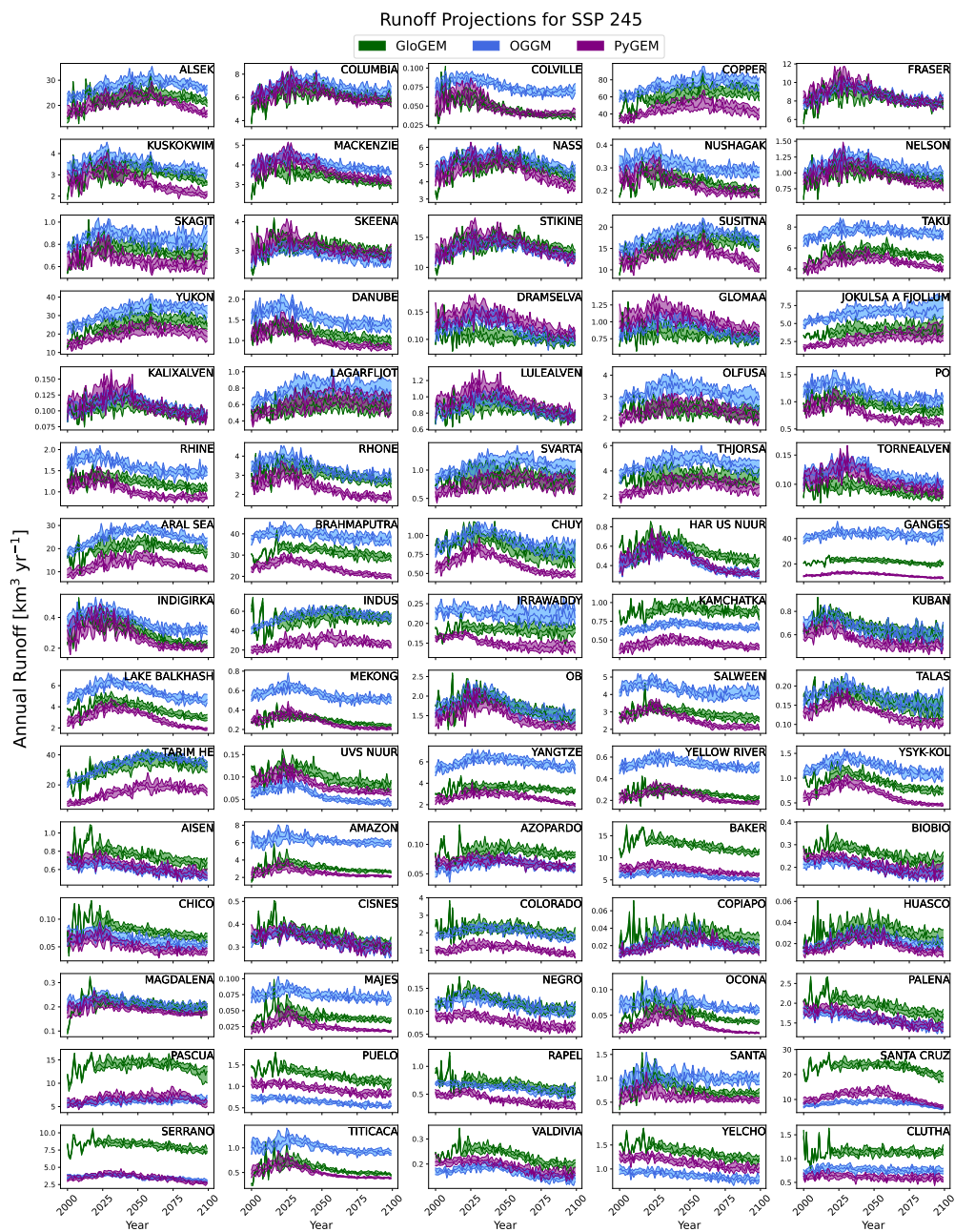
Figure A1. Total annual runoff projections for all 75 glaciated major river basins given SSP 2-4.5. The multi-GCM range is highlighted in the same way as Fig. 2. In this plot we have also indicated the calculated year of peak water with a vertical dashed line. The color of each line corresponds to the glacier evolution model color indicated by the legend.
