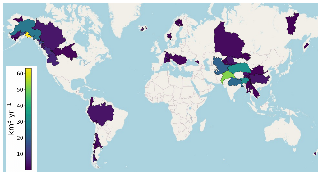
Figure 1. All 75 basins analyzed in the study. The color fill corresponds to the basin’s average annual glacier runoff over the entire period. Average runoff values are derived from the median of each glacier model’s multi-GCM median under the SSP2-4.5 scenario. This map was generated by our online interactive mapping tool (Wimberly, 2024b), available at link when published
