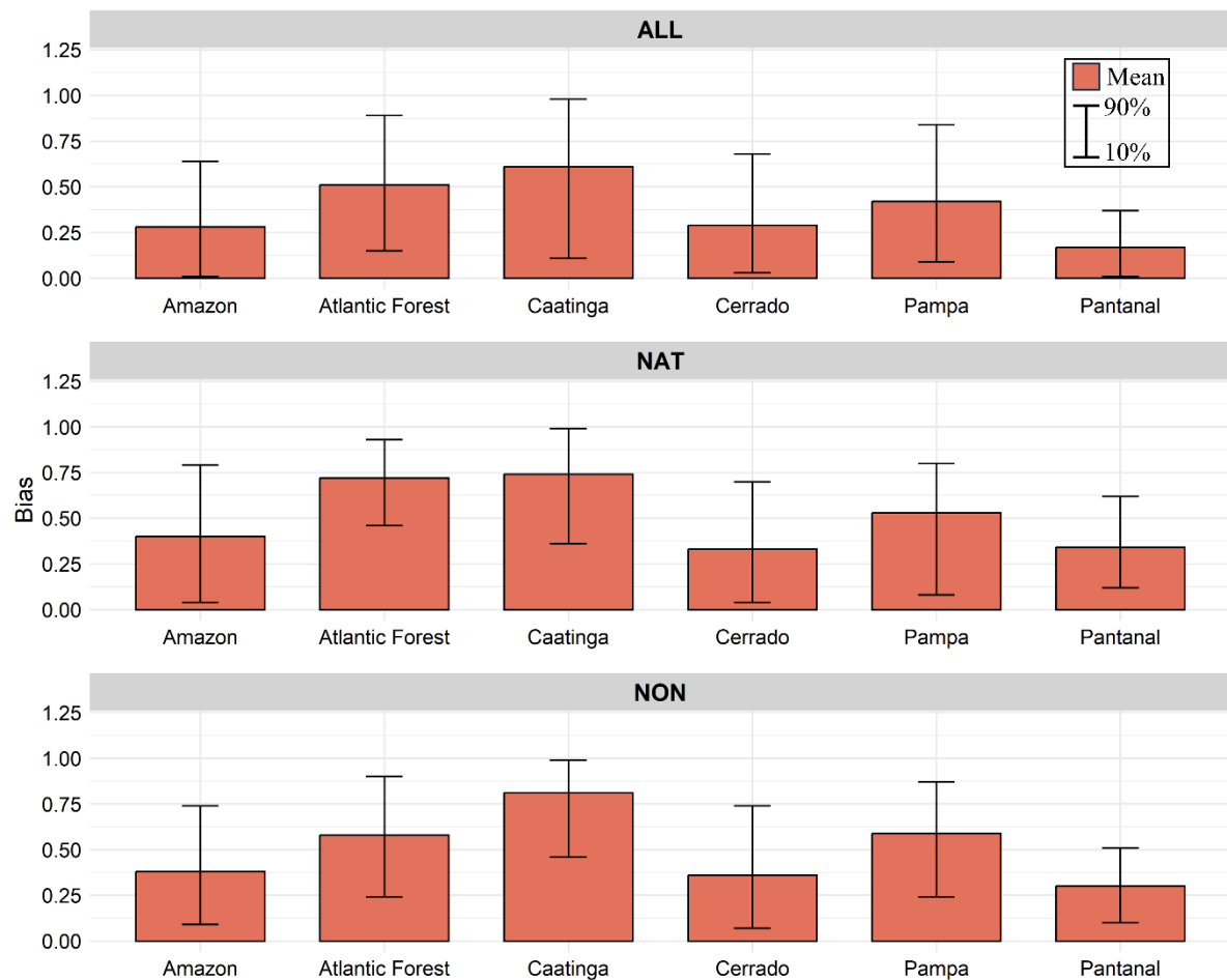
536 Figure 7: Mean bias and 10th and 90th percentiles of the modeled burned area to total area 537 (ALL, top), natural vegetation area (NAT, middle) and non-vegetation area (NON, bottom). 538
