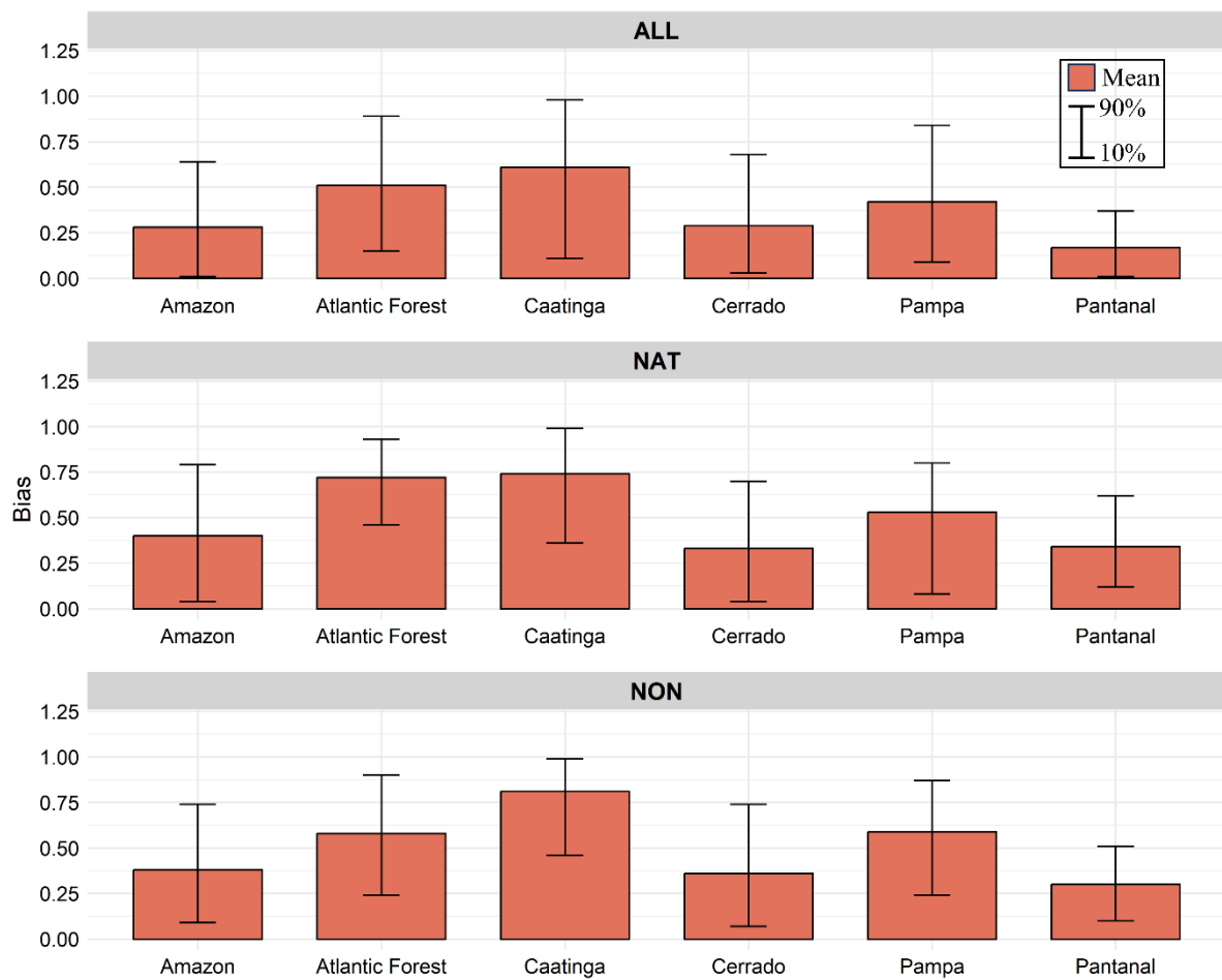
Figure 7: Mean bias and 10th and 90th percentiles of the modeled burned area to total area (ALL, top), natural vegetation area (NAT, middle) and non-vegetation area (NON, bottom).
