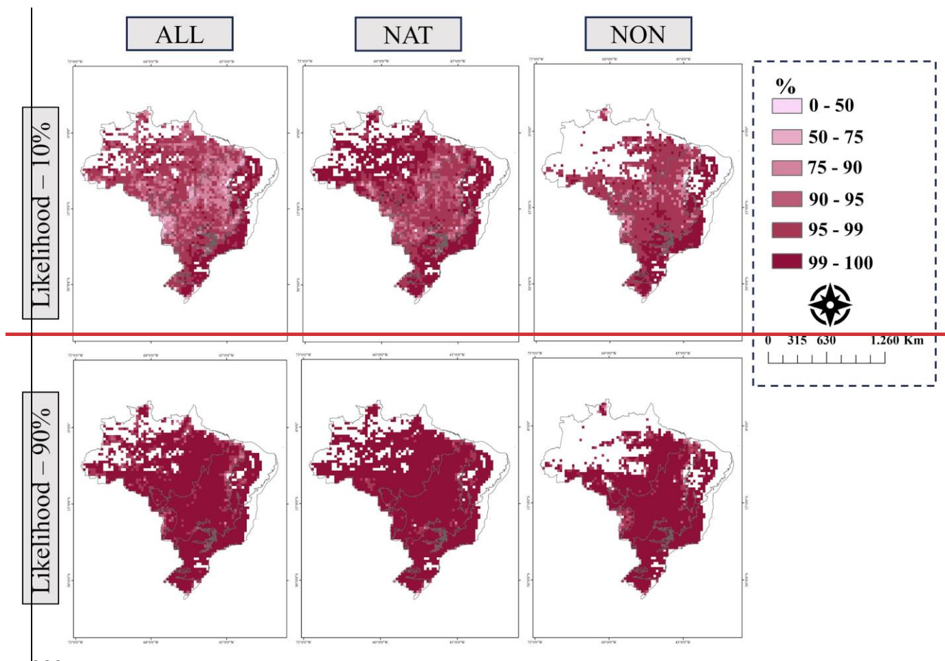
571 Figure 6: Spatial likelihood of the observations given the model parameters considering the 572 months with worst performance (top row) and the months with best performance (bottom 573 row). A satisfactory performance of the model is considered with values above 0.5. The 574 columns represent different fire categories: total burned area (ALL), burned areas in 575 natural vegetation (NAT) and burned areas non-natural vegetation (NON). The rows 576 represent burned area at the 10th and 90th percentiles, respectively.
