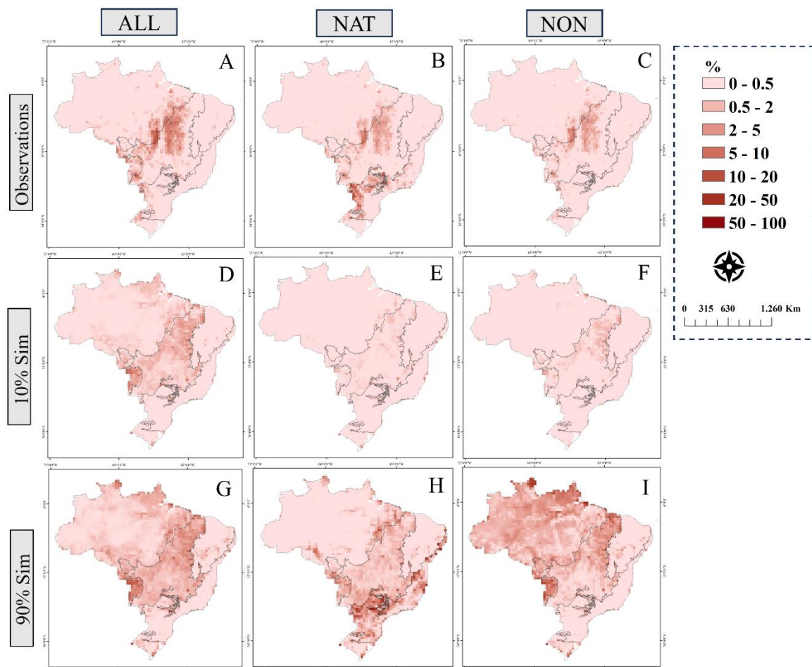
Figure 5: Maps of modeled and observed percentage (%) of burned area . First row: show the observed burned area for , July-September 2002-2009 annual average categorized into total burned area for (ALL, left), burned area in natural vegetation (NAT, middle), and burned area in non-vegetation (NON, right). Second and third row show the
