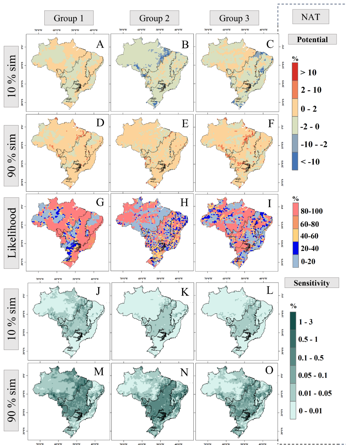
Figure 119: Same as Fig. 1089 but for NAT.
