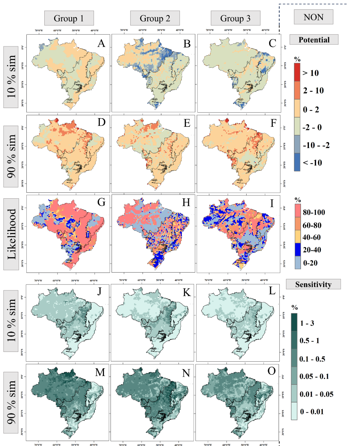
Figure 110: Same as Fig. 1089 but for NON.
