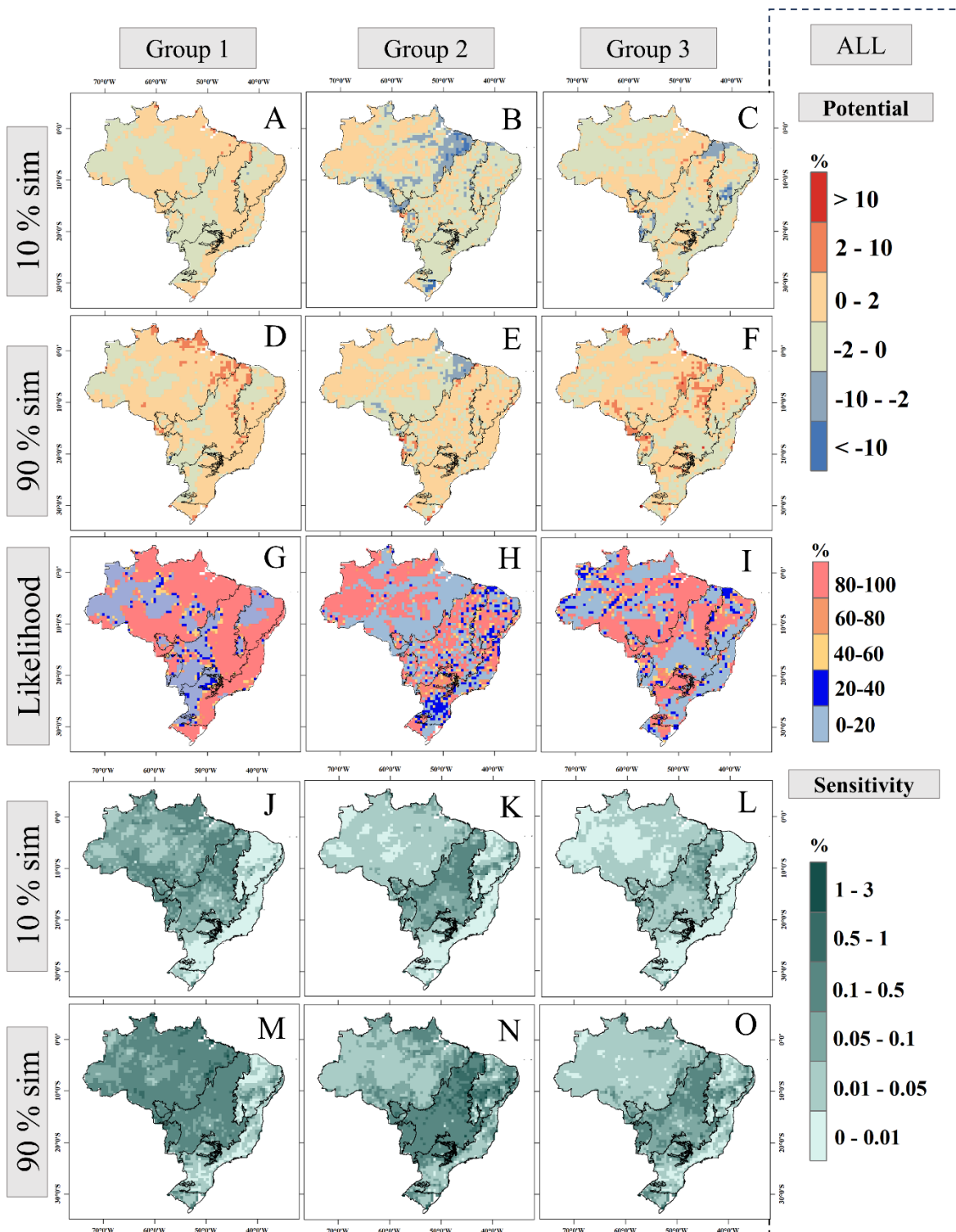
Figure 108: Response maps to ALL displaying the potential 10h percentile (first row), 90th percentile (second row), likelihood (third row) and sensitivity responses 10th percentile (fourth row) and 90th percentile (fifth rows). Each column presents the results for one g Group 1 (Maximum Temperature and Precipitation), Group 2 (Edge density and Road density), and Group 3 (Forest, Pasture, and Carbon in dead vegetation) of explanatory variables.
