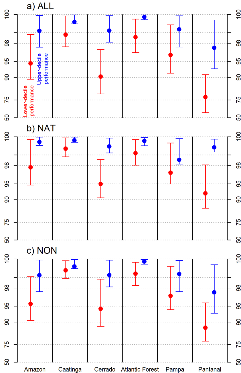
Figure 6: Likelihood (%) per biome of the observations given the model parameters over all cells and timesteps. Lower-decline performance is represented in red and Upper-decline performance in blue for ALL (a), NAT (b) and NON (c).
