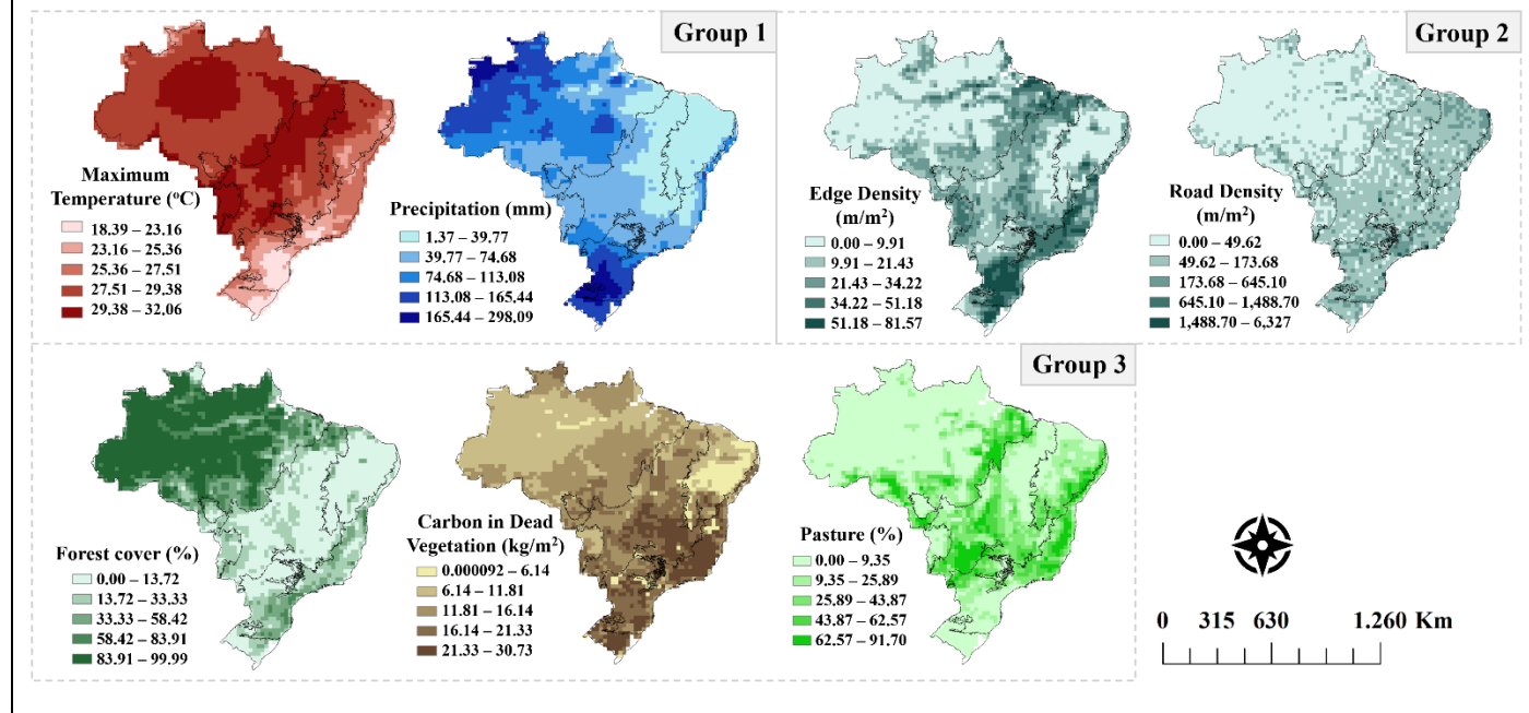
314 Figure 3: Mean of the selected explanatory variables for August, September and October 315 from 2002 to 2019.
