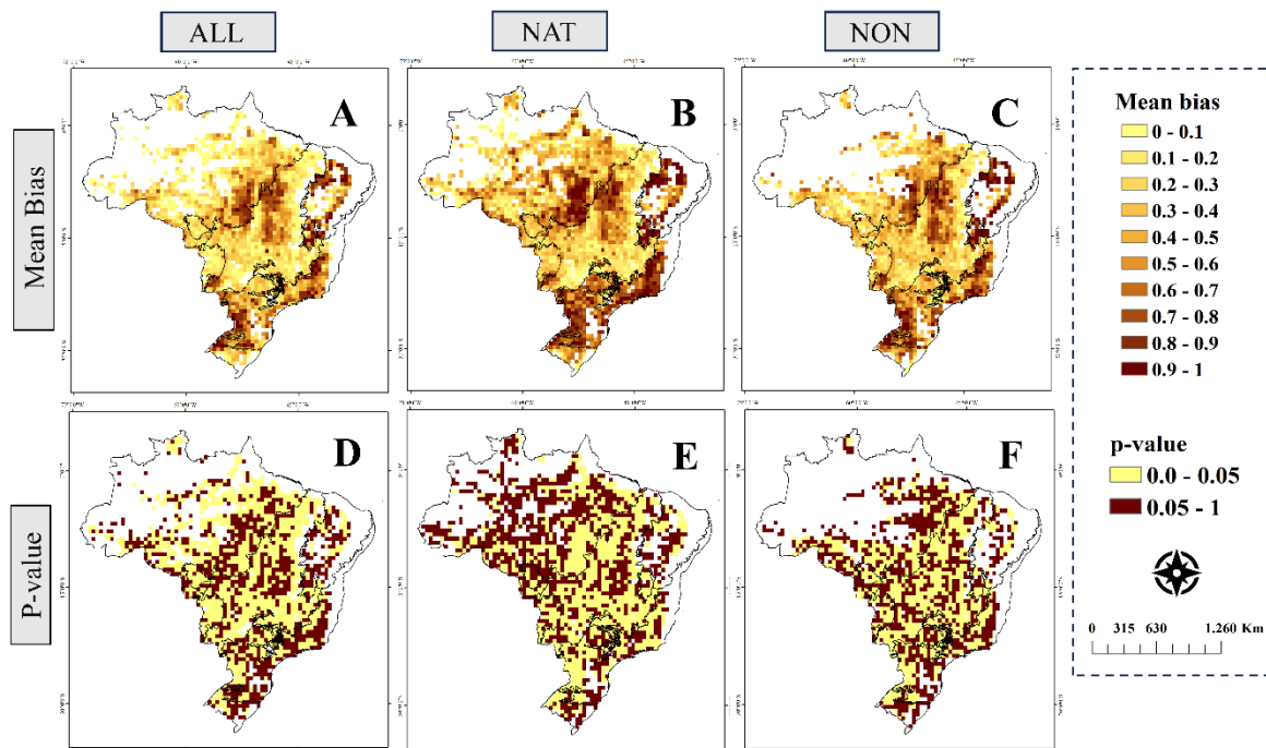
Figure 87: Top row: Spatial mean bias of the modeled burned area to total area (ALL, (left), natural vegetation area (NAT, (middle) and non-vegetation area (NON, (right). Bottom row: Significance of the mean bias considering a 95% confidence level ( p\text{-value} < 0.05 ). Pixels with p\text{-value} > 0.05 (brown color) are not significantly different from 0.5 mean bias meaning that they are unbiased.
