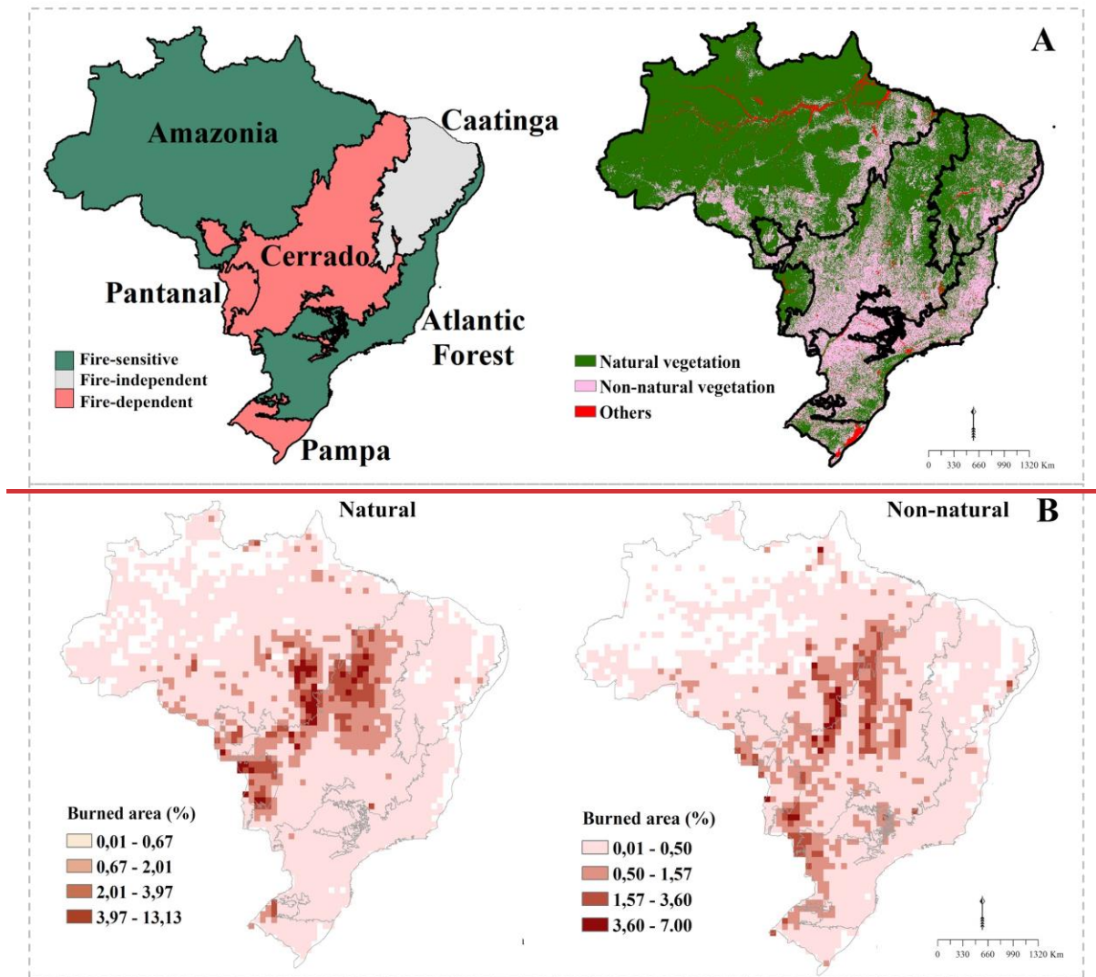
Figure 1: (A) Brazilian biomes classified as Fire-sensitive, Fire-independent and Fire-dependent on the left (Hardesty et al. 2005) and Natural vegetation (Forests, Grasslands and Savannas) and Non-natural vegetation (Pasture, Cropland and Forest Plantations) in 2019 in Brazil on the right. (B) NAT's mean burned area percentage per pixel is on the left and NON is on the right. The maps show the mean for August, September and October from 2002 to 2019.
