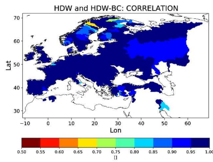
901 Figure S1: Correlation of a) HDW and b) HDW-BC with observations as well as c) 902 HDW with HDW-BC from 1979-2014.
