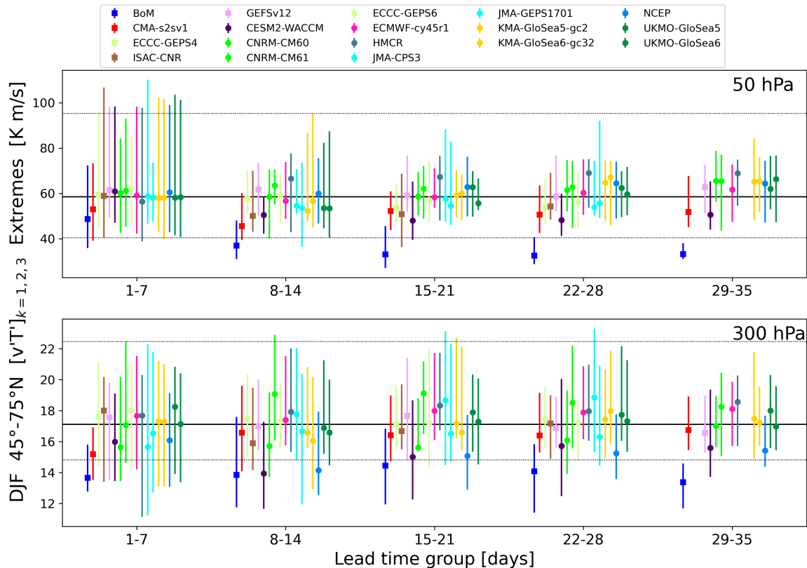
Figure 10. The 95th percentile daily eddy heat flux extremes for 45\text{-}75^\circ\text{N} during winter (DJF) from 1999-2010 for all models by weekly lead time group. The median is indicated by the marker and the \pm 2 standard deviations by the whiskers for (top) 50hPa and (bottom) 300hPa. The equivalent values from reanalysis are given by the horizontal black lines (bold: median; thin: \pm 2 standard deviations).
