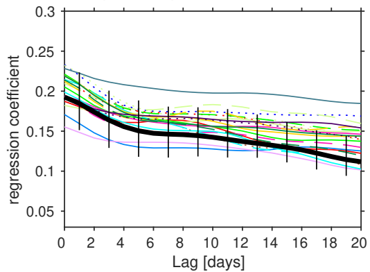
downward coupling of 100hPa polar cap Z with 850hPa polar cap Z SH SON
