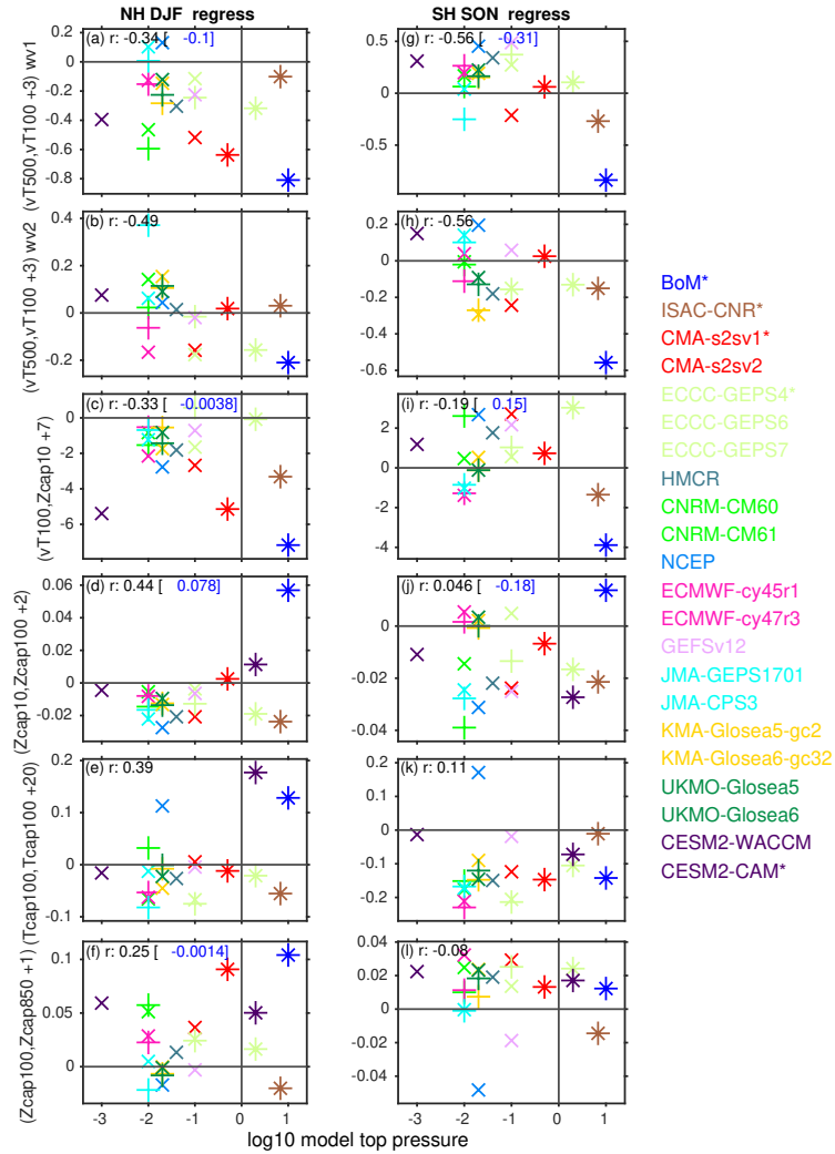
Figure 5. Relationship between the bias in coupling strength as compared to ERA5 for corresponding dates and vertical lid. Coupling strength is defined using regression; the corresponding figure for correlations is in Supplemental Figure S3. The correlation for each panel is indicated, and also the correlation without BoM in blue if this correlation differs from the overall correlation by more than 0.2. The left column is for the NH in DJF, and the right column is for the SH in SON. Low top models are indicated by an ‘*’, older versions of high-top models with a ‘+’, and the latest version of high-top models with an ‘x’. (a,g) upward wave-1 coupling on day 3 from Figure 3; (b,h) upward wave-2 coupling on day 3 from Figure 3; (c,i) sensitivity of Z10hPa polar cap to 100hPa heat flux on day 5 from Figure 8; (d,f) coupling strength of Z10hPa polar cap to Z100hPa polar cap on day 3 from Figure 12; (e,k) persistence of T100hPa polar cap on day 20 from Figure 14; (f,j) coupling strength of Z100hPa polar cap to Z850hPa polar cap on day 20 from Figure 13. The lid of GloSea is at 85km; we represent this with a value of 0.02hPa. The lid of WACCM is at 140km; since the levels in the ionosphere are not expected to improve the representation of stratosphere-troposphere coupling, we represent this model with a lid at 0.001hPa (still the highest lid of any model). A null hypothesis of no relationship can be rejected at the 95% confidence level using a two-sided Student-t test for correlations exceeding 0.42.
