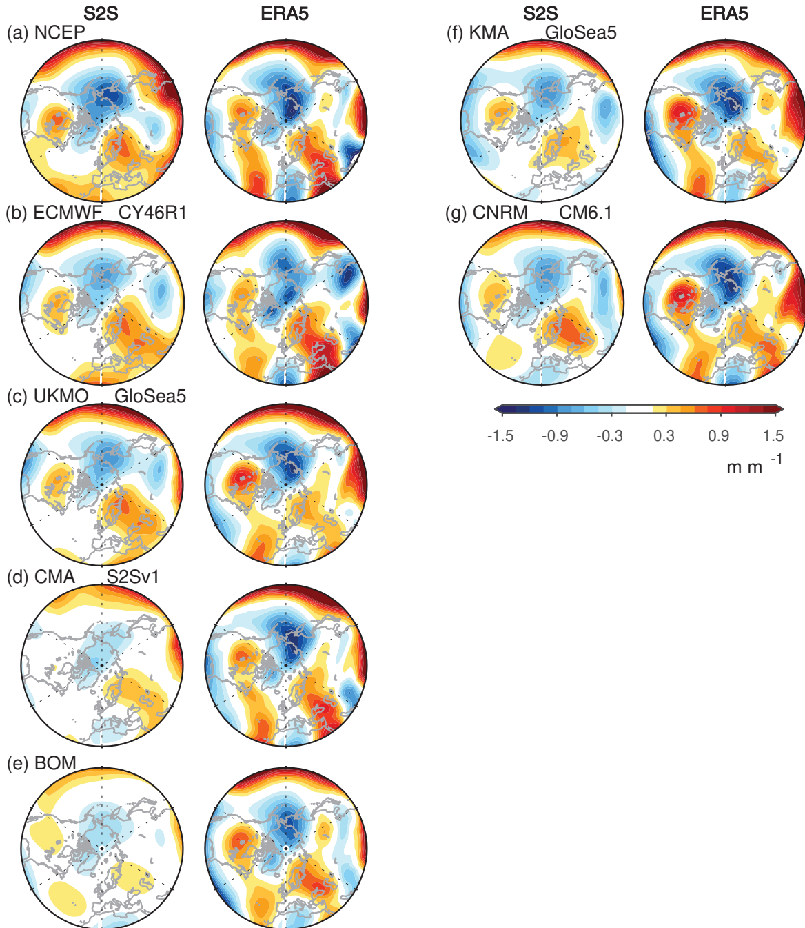
Figure 9. Regression coefficient of the change in polar cap geopotential height at 10-hPa over 10 days ( Z_{\text{pole,day10}} - Z_{\text{pole,day0}} ; a vortex weakening index) with Z500 anomalies on day 0. Uses week 3 and 4 of December/January initializations for Z500 anomalies on day 0. The regression coefficients are computed for each ensemble member, and then averaged.
