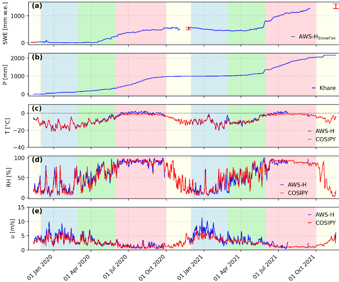
150 Figure 2. Daily values of (a) Cumulative SWE measured by SnowFox (blue line) and manual field measurements represented by red vertical error bars, (b) cumulative precipitation at Khare, (c-d-e) air temperature, relative humidity, and wind speed, respectively, measured at AWS-H (blue) and used to force COSIPY at the corresponding grid cell (red) (see Khadka et al. (2024) for details). The black dashed line in panel c corresponds to T = 0^{\circ}\text{C} . Light red, yellow, blue and green shaded areas represent the monsoon, the post-monsoon, the winter and pre-monsoon, respectively.
