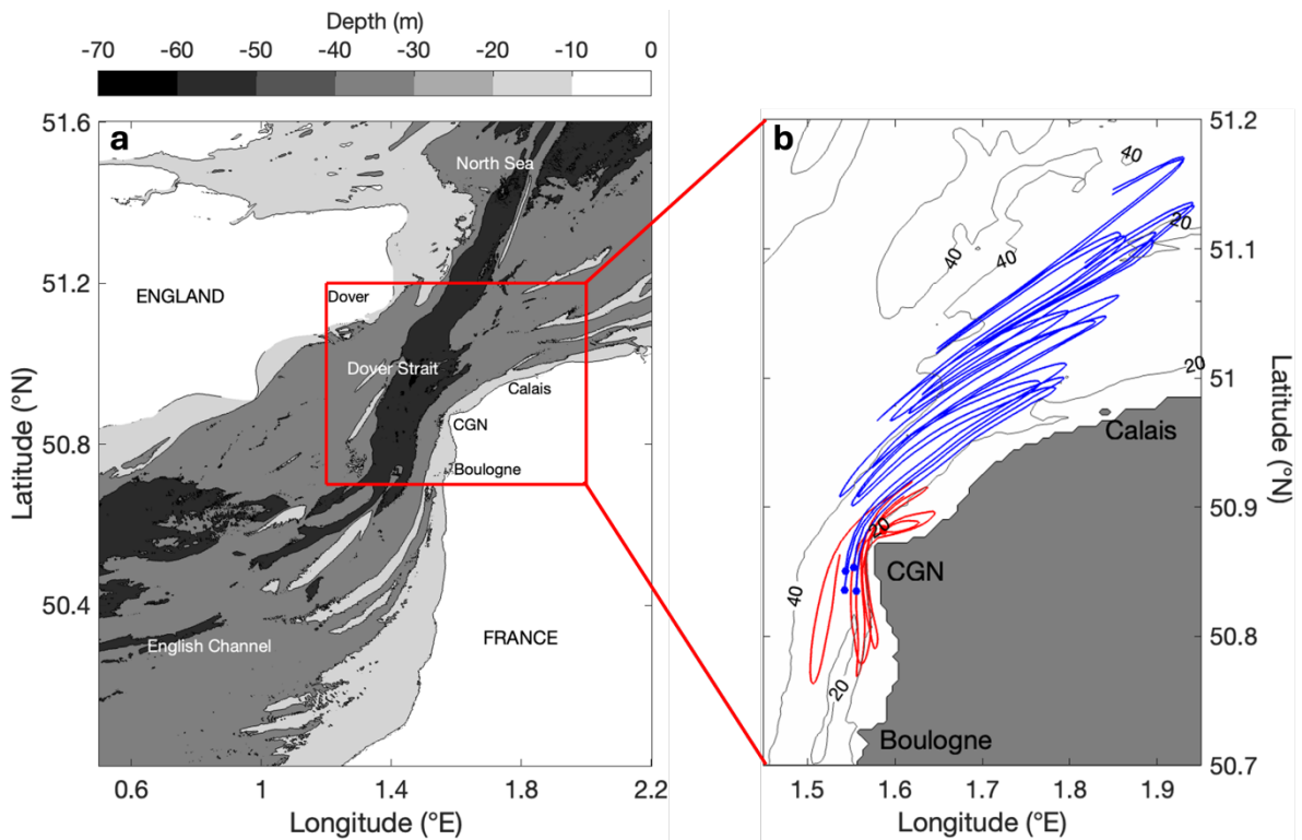
85 Figure 1. (a) Modeling domain. Bathymetry shown by grey shading. Red square delimits the region where the Lagrangian measurements were performed. (b) Trajectories of Lagrangian drifters released during two field surveys on November 26, 2020 (red) and on May 10, 2021 (blue). Geographic names used in the text are also shown.
