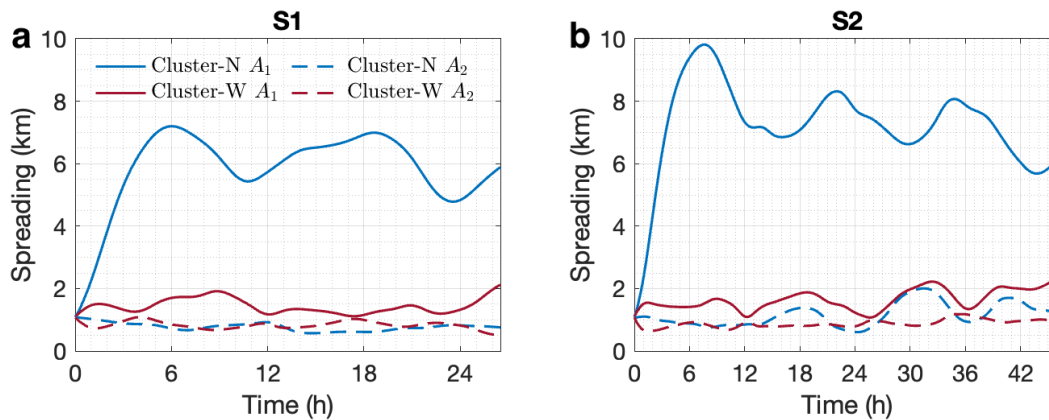
420 Figure 10. Time evolution of spreading A_1 (solid line) and A_2 (dashed line) under environmental conditions observed during S1 (a) and S2 (b). Spreading of cluster-N are shown in blue and of cluster-W in dark red. Results are obtained from the model after performing wind-induced velocity correction.
