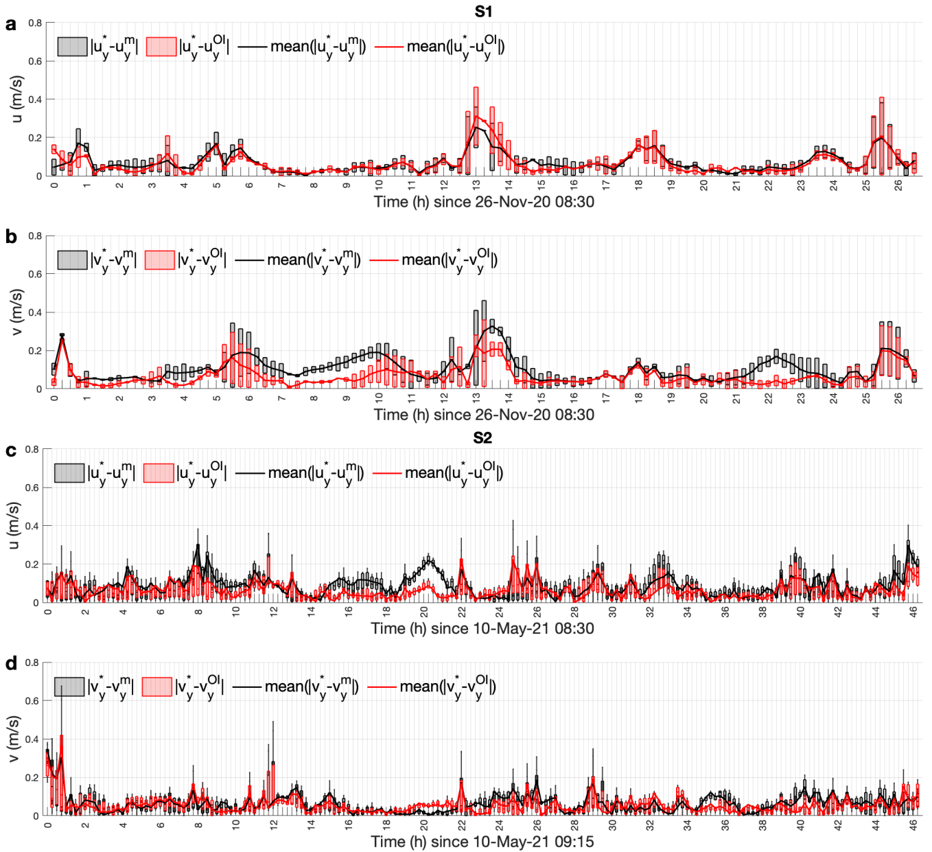
310 Figure 5. Boxplots of absolute zonal (a, c) and meridional (b, d) velocity difference between observations and initial model (black) and observations and optimized model (red) at S1 (a, b) and S2 (c, d) drifter locations. For S1 (a, b), where only two drifters are considered, the top and bottom edges of each box are the maximum and minimum values, and the line within the box indicates the median, equal to the mean. For S2 (c, d), the top and bottom edges of each box are the upper (0.75) and lower (0.25) quartiles, respectively. The line within the box indicates the median. The whiskers above and below each box are the nonoutlier maximum and minimum.
