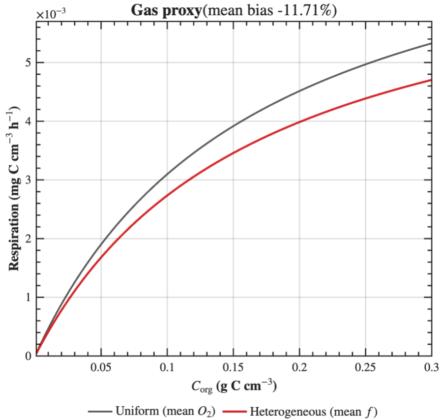
Figure 3: Aerobic respiration across C_{org} when evaluated at the mean O_2 (“Uniform”) versus averaged over the full O_2 distribution (“Heterogeneous”). For the gas-phase proxy, the mean aggregation bias is -11.71% (uniform overestimates respiration).
