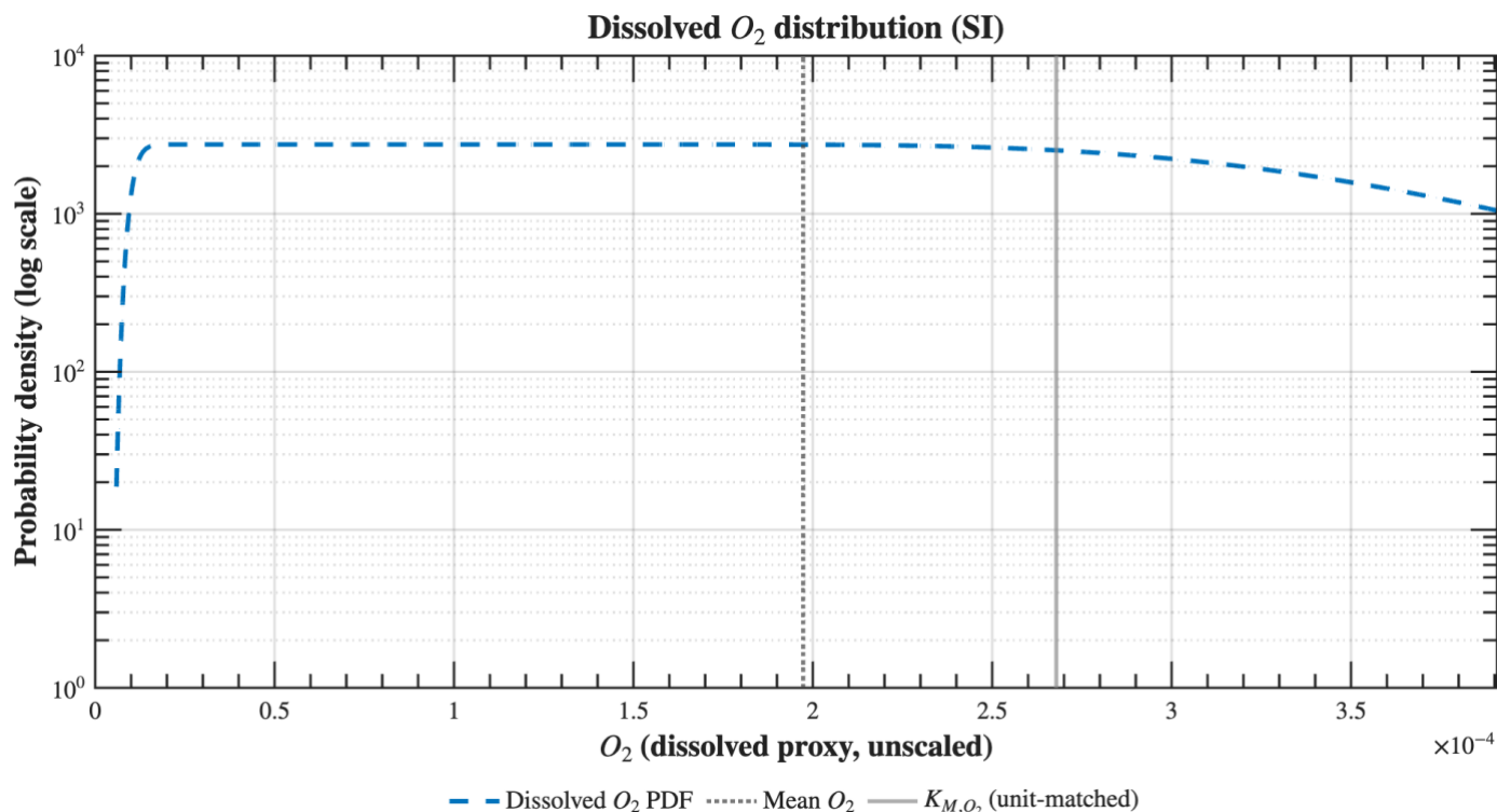
Figure 2b: Dissolved-phase O_2 PDF (log scale) with vertical markers for the distribution mean and the unit-matched K_{M,O_2} used in Fig. 4. This places dissolved and gas cases on comparable relative saturation without rescaling O_2 itself.
