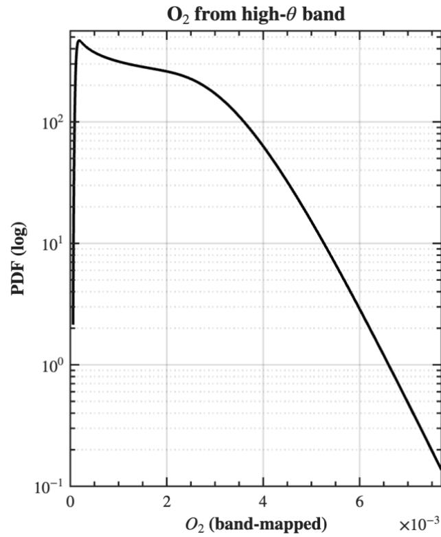
360 Figure S9: Probability density of O_2 obtained by mapping a narrow water-content band, \theta \in [0.65, 0.68] , to gas-phase O_2 using the same proxy as in the main analysis; the density is shown on a log scale. This “high- \theta ” band has much lower variance than the full rhizosphere distribution. Evaluated at C_{org} = 0.15 \text{ g C cm}^{-3} , the respiration predicted at the mean O_2 (uniform configuration) is slightly larger than the heterogeneous average E[f(O_2)] , giving an aggregation bias of -0.51\% (uniform overpredicts). Numerically: R_{uniform} = 1.2657 \times 10^{-4} and R_{heterogeneous} = 1.2592 365 \times 10^{-4} \text{ mg C cm}^{-3} \text{ h}^{-1} (calibrated DAMM parameters; substrate term evaluated at \theta_{ref} = 0.30 ).
