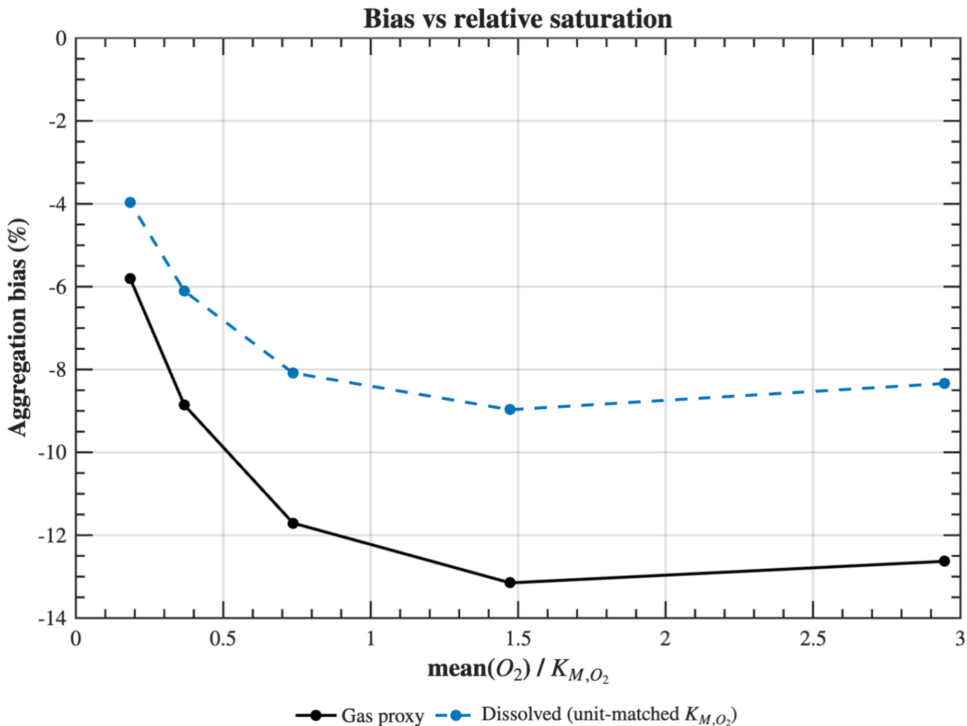
Figure 4: Aggregation bias (%) as a function of mean ( O_2 ) / K_{M,O_2} for two O_2 drivers: gas proxy (solid black) and dissolved proxy with unit-matched K_{M,O_2} (dashed blue). Bias magnitude increases as mean O_2 approaches K_{M,O_2} and decreases at very low or very high relative saturation.
