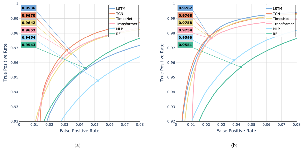
Figure 5. Model comparison shown as ROC curves for two different versions of the six models: (a) model performance with all seven input features - HS, TSS, TA, RSWR, RH, WV and solar altitude, and (b) with the four relevant input features - HS, TSS, TA and RSWR. Every plot additionally shows the macro-F1 score for the threshold where TPR = FPR (the point on the curve).
