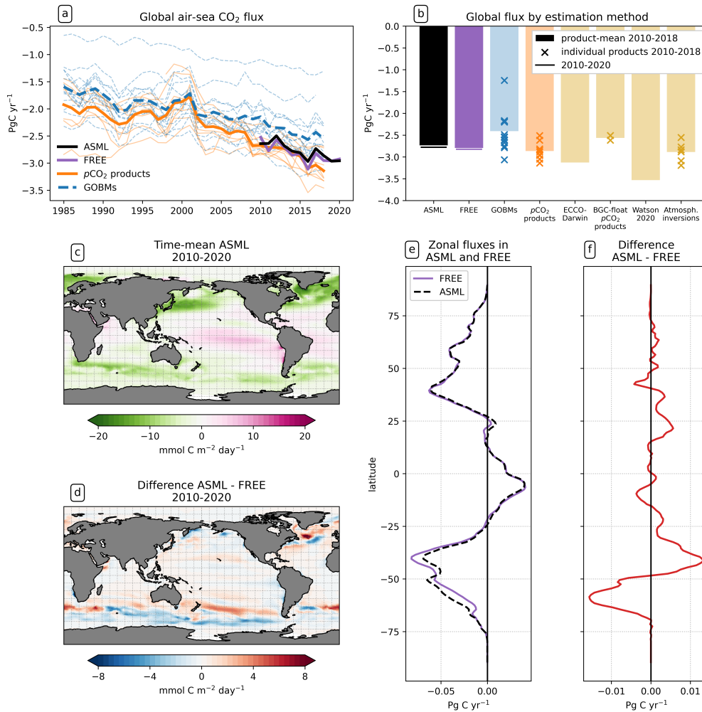
Figure 4. Effect of data assimilation on the air-sea CO 2 flux (negative: into the ocean). (a) Annual time-series of global flux in Pg C yr -1 in FESOM2.1-REcoM3 with ASML (black) and FREE (violet); and RECCAP2 estimates (DeVries et al., 2023) with pCO 2 -products (orange) and GOBMs (blue) and their respective means (bold lines). Here, the river flux adjustment ( -0.65 Pg C yr -1 ) was applied to the pCO 2 products. (b) Time-mean global flux 2010-2018 in ASML (black), FREE (violet); and RECCAP2 estimates grouped by method (DeVries et al., 2023). Crosses represent individual estimates (e.g. individual GOBMs) and bars represent the method mean (e.g. mean of twelve GOBMs). Here, the river flux term was applied to all estimates except the models following the Global Carbon Budget methodology (Friedlingstein et al., 2023). For FESOM2.1-REcoM3, additionally the time-mean 2010-2020 is shown (horizontal lines). (c) Spatial distribution of CO 2 flux averaged over the period 2010-2020 in ASML. (d) Spatial distribution of CO 2 flux difference ASML – FREE averaged over the period 2010-2020 (e) Zonal averages of CO 2 flux 2010-2020 in ASML and FREE, and their difference in (f).
