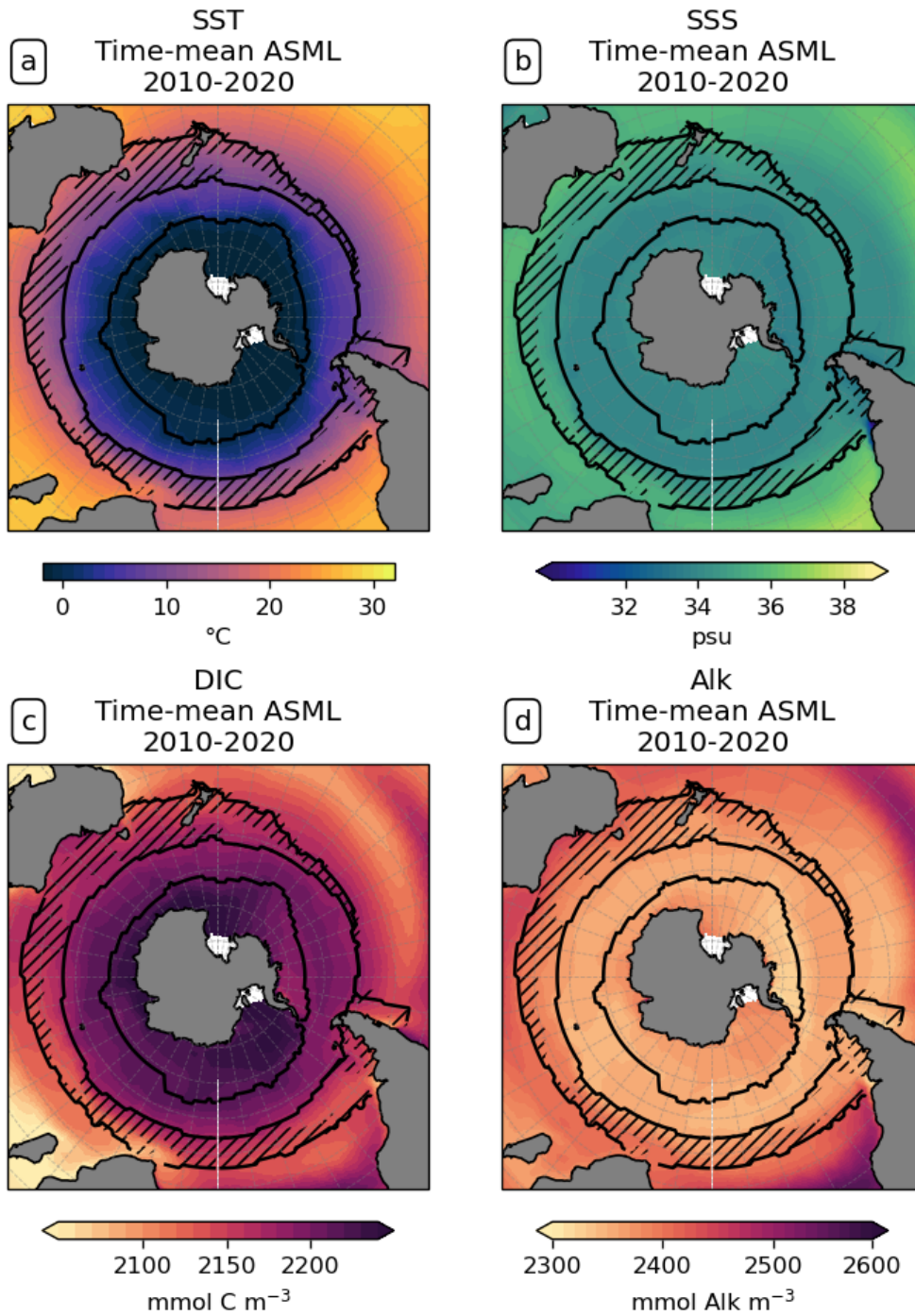
Figure A10. Southern Ocean time-mean sea surface in-ASML , (a) temperature, (b) salinity, (c) DIC and (d) alkalinity in ASML .
