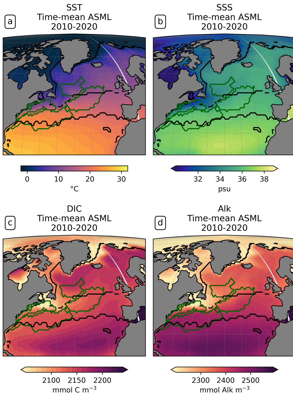
Figure A15. North Atlantic time-mean sea surface in ASML , (a) temperature, (b) salinity, (c) DIC and (d) alkalinity in ASML .
