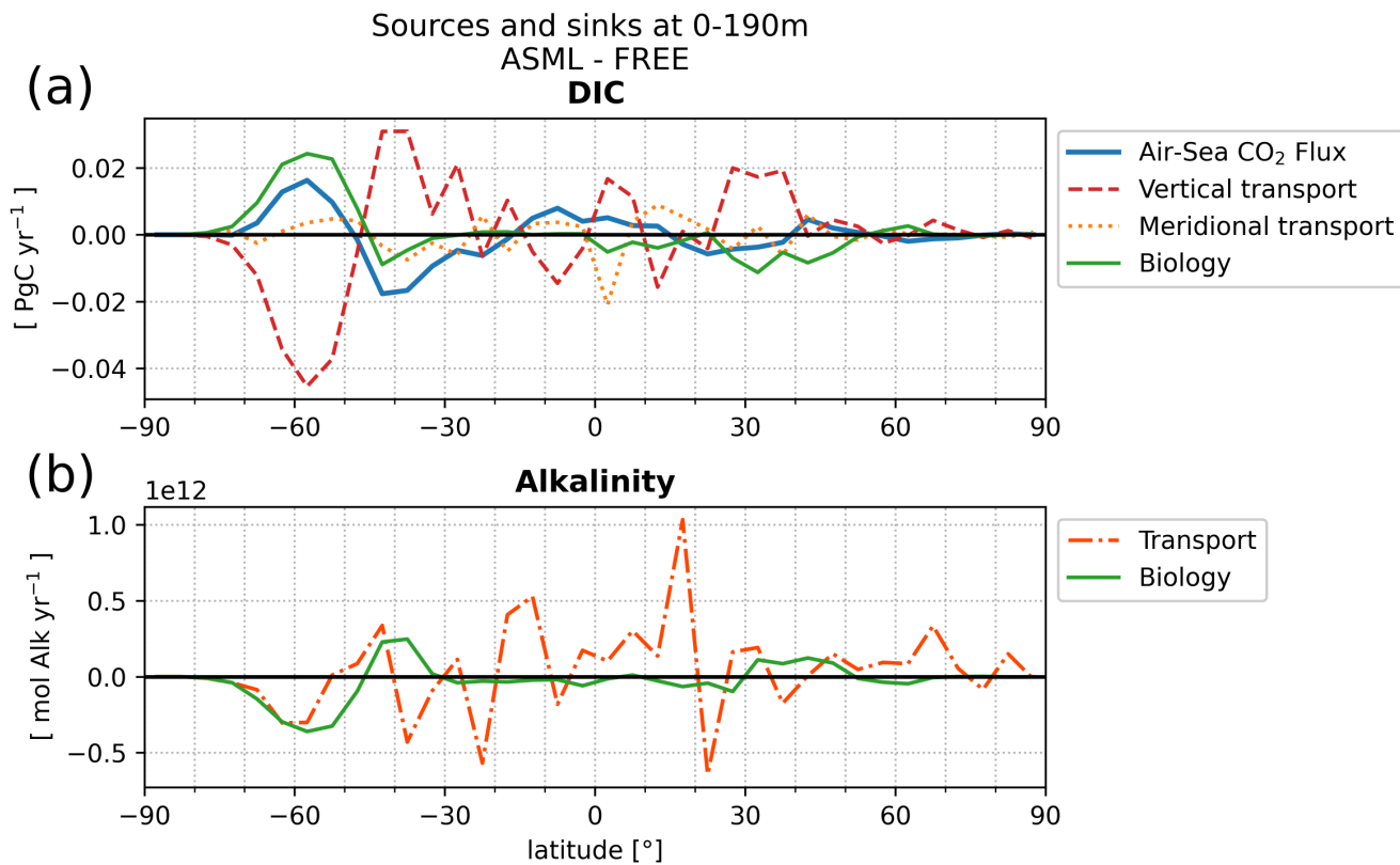
Figure A13. The difference (ASML-FREE) - ASML - FREE of source and sink terms for the ocean's (a) DIC and (b) alkalinity content integrated over 0-190 m per 1^\circ latitude in the year 2020. Transport terms include advection and diffusion of DIC and alkalinity. Meridional transport is averaged across bins of 5^\circ latitude. In panel b, vertical and horizontal transport are summed up for readability. Biological terms for DIC are the sum of: photosynthesis, respiration, remineralization of dissolved organic carbon, and formation and dissolution of calcite. Biological terms for alkalinity are the sum of: nitrogen assimilation and remineralization, and formation and dissolution of calcite.
