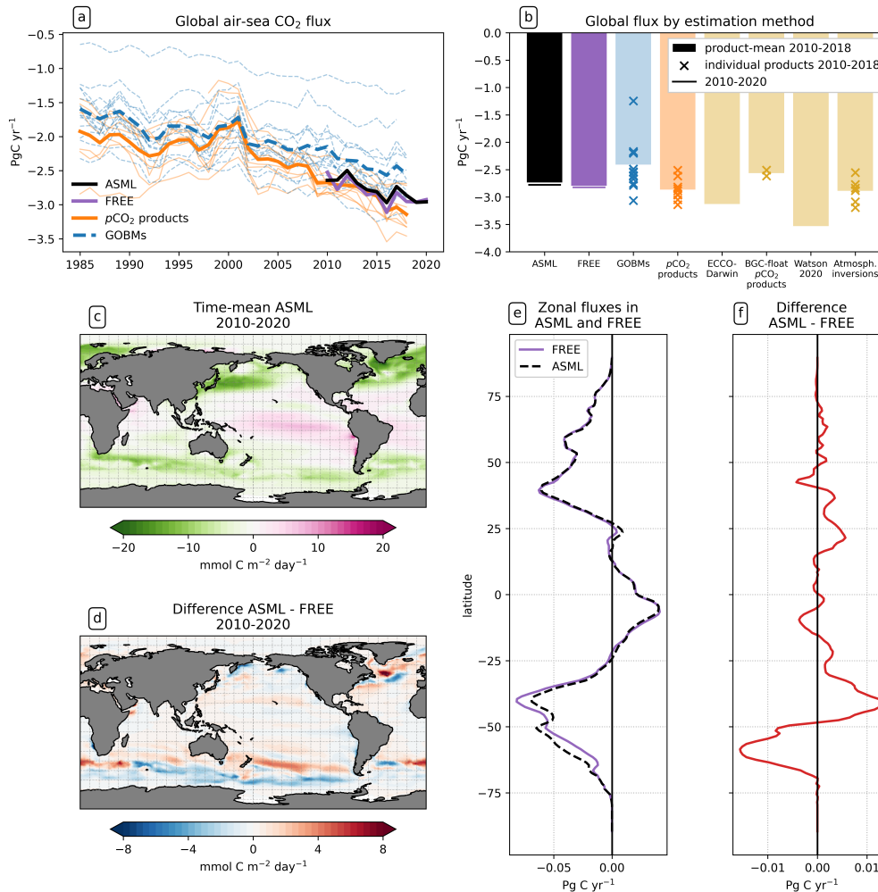
Figure 4. Effect of data assimilation on the air-sea CO 2 flux (negative: into the ocean). (a) Annual time-series of global flux in Pg C yr -1 in FESOM-REcoM-PDAF FESOM2.1-REcoM3 with ASML (black) and FREE (violet); and RECCAP2 estimates (DeVries et al., 2023) with pCO 2 -products (orange) and GOBMs (blue) and their respective means (bold lines). Here, the river flux adjustment ( -0.65 Pg C yr -1 ) was applied to the pCO 2 products. (b) Time-mean global flux 2010-2018 in ASML (black), FREE (violet); and RECCAP estimates grouped by method (DeVries et al., 2023). Crosses represent individual estimates (e.g. individual GOBMs) and bars represent the method mean (e.g. mean of twelve GOBMs). Here, the river flux term was applied to all estimates except the models following the Global Carbon Budget methodology (Friedlingstein et al., 2023). For FESOM-REcoM-PDAF FESOM2.1-REcoM3 , additionally the time-mean 2010-2020 is shown (horizontal lines). (c) Spatial distribution of CO 2 flux averaged over the period 2010-2020 in ASML. (d) Spatial distribution of CO 2 flux difference between ASML and FREE ASML - FREE averaged over the period 2010-2020 (e) Zonal averages of CO 2 flux 2010-2020 in ASML and FREE, and their difference in (f).
