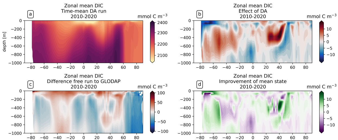
Figure A17. Zonally averaged DIC: (a) time-mean in ASML, (b) difference \text{ASML} - \text{FREE} , (c) difference \text{FREE} - \text{OBS} compared to \text{FREE} - \text{OBS} based on the GLODAP climatology for DIC (Lauvset et al., 2016) and (d) improvement respective to the GLODAP climatology.
