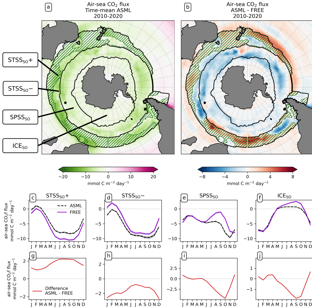
Figure 5. Effect of data assimilation on Southern Ocean CO 2 flux ( negative: into the ocean ) and its seasonality averaged over the period 2010-2020. Negative numbers indicate a flux into the ocean. Additionally, lines in a and b denote the regions, and the green hatching denotes the STSS S0+ . (a) Map of mean CO 2 flux in ASML. (b) Map of difference between CO 2 flux in ASML and FREE difference ASML - FREE . (c - f) Seasonal cycle of air-sea CO 2 flux by region. Shading indicates the range of ensemble members in the year 2020. (g - j) Seasonal difference in air-sea CO 2 flux between ASML and FREE difference ASML - FREE by region. Note the different scales.
