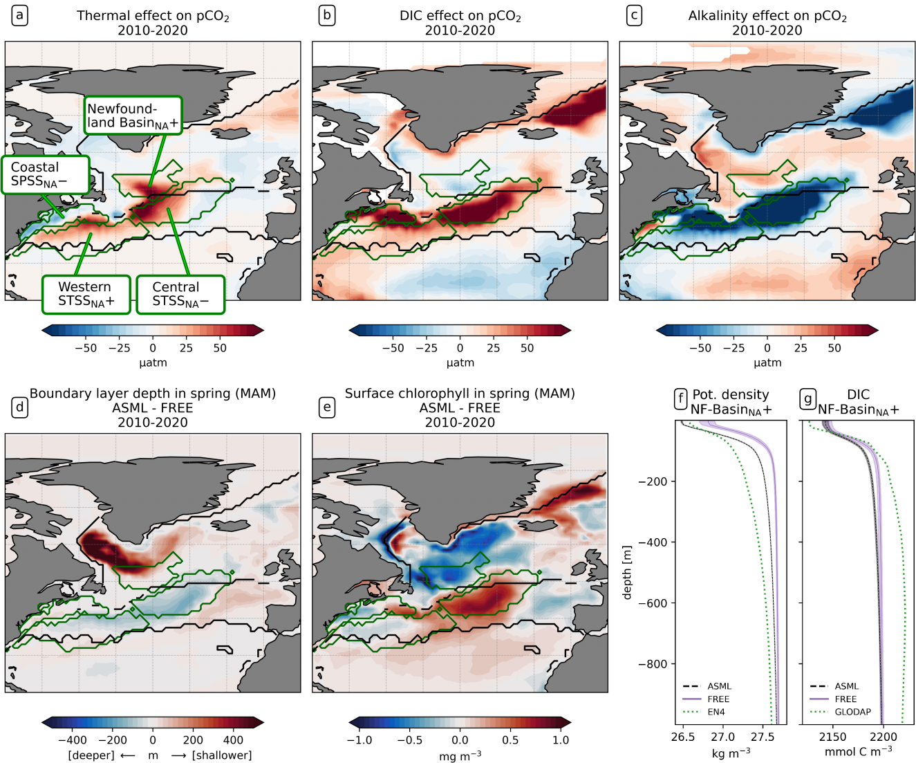
Figure 8. Drivers of the effects of data assimilation on air-sea \text{CO}_2 flux- \text{pCO}_2 in the North Atlantic. Panels a, b and c show the effects of SST, surface DIC and alkalinity differences between-ASML and FREE-ASML - FREE on surface \text{pCO}_2 . (d) Difference of boundary layer depth ( ASML-FREE-ASML - FREE ) for spring (MAM) 2010-2020, where positive denotes a shallower boundary layer in the-ASML . (e) Difference of surface chlorophyll ( ASML-FREE-ASML - FREE ) for spring (MAM) 2010-2020. (f) Potential density profiles for the Newfoundland Basin NA+ region, with FREE (violet line) and ASML (dashed black line) based on daily T and S, and with EN4-OA (dotted green line) based on monthly T and S. (g) DIC profiles for the Newfoundland Basin NA+ region, showing FREE (violet line), ASML (dashed black line) from 2010-2020 and climatological DIC from GLODAP. Shading in f and g indicates the range of ensemble members in the year 2020.
