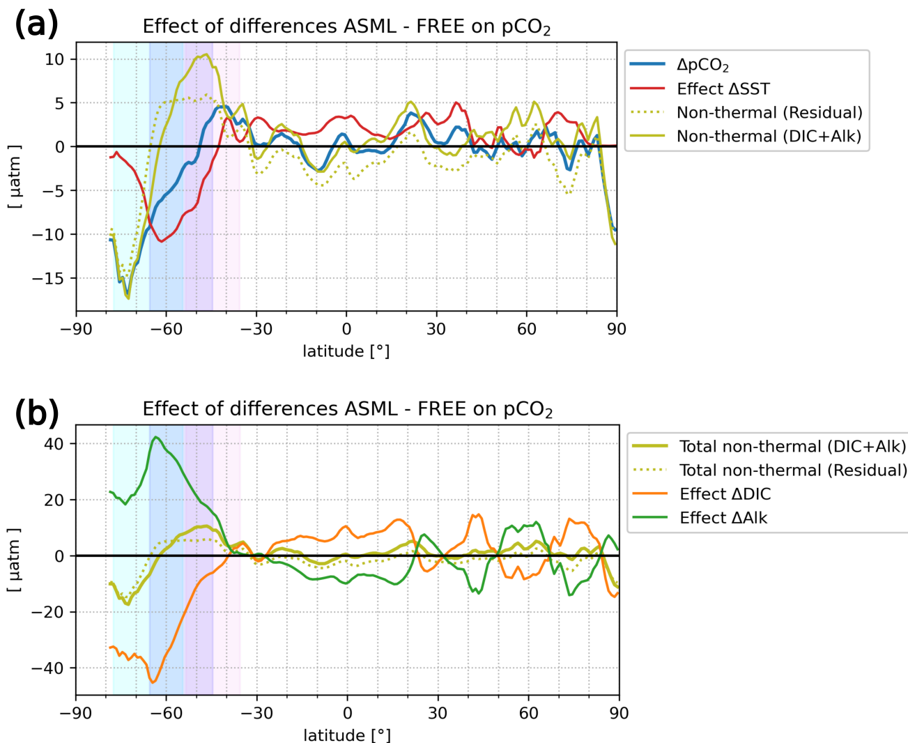
Figure A9. The net difference (ASML-FREE) - ASML - FREE of surface pCO 2 by latitude (panel a, blue line), and the offline-approximated effects causing that pCO 2 difference for the period 2010-2020: Thermal effect (panel a, red line); non-thermal effect calculated, firstly \tau as the residual i.e. net-minus-thermal (panels a and b, light-green dotted lines) and, and secondly \tau as the sum of alkalinity and DIC effects (panels a and b, light-green solid lines); and effects of alkalinity and DIC individually (panel b, orange and dark-green lines). The shaded areas in the background indicate the zonal extent of defined biomes in the Southern Ocean: ICE SO in light-blue, SPSS SO in blue and STSS SO in pink. Colors blend where the regions overlap.
