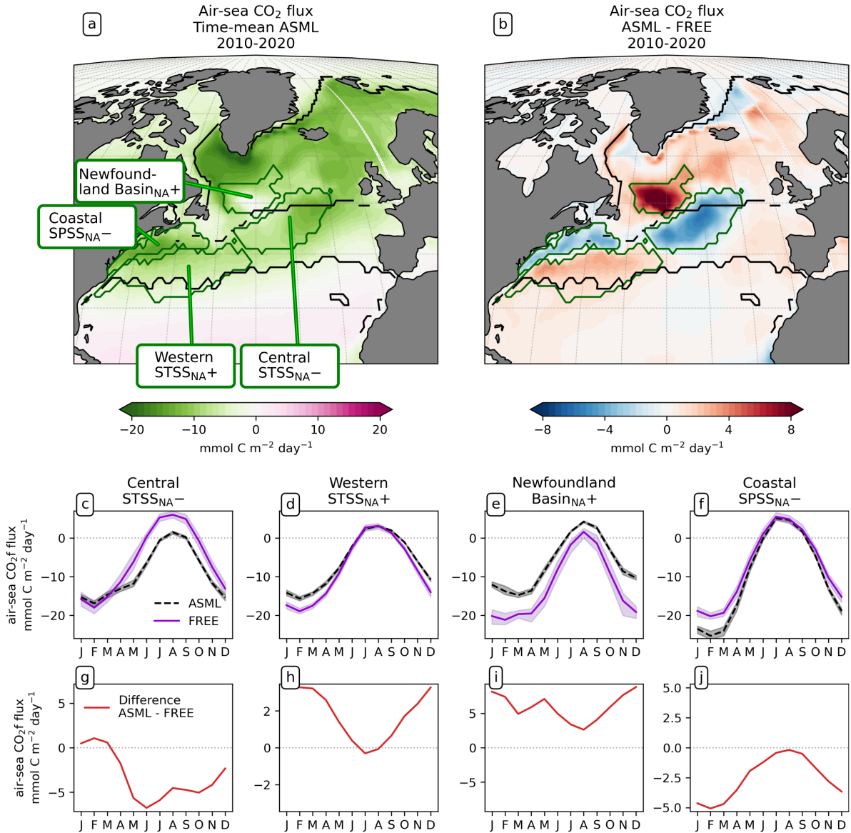
Figure 7. Effect of data assimilation on North Atlantic CO 2 flux (negative: into the ocean) and its seasonality averaged over the period 2010-2020. Negative numbers indicate a flux into the ocean. (a) Map of mean CO 2 flux in ASML. (b) Map of difference between CO 2 flux in ASML and FREE difference ASML – FREE. (c - f) Seasonal cycle of air-sea CO 2 flux by region. Shading indicates the range of ensemble members in the year 2020. (g - j) Seasonal difference in air-sea CO 2 flux between ASML and FREE difference ASML – FREE by region. Note different scales.
