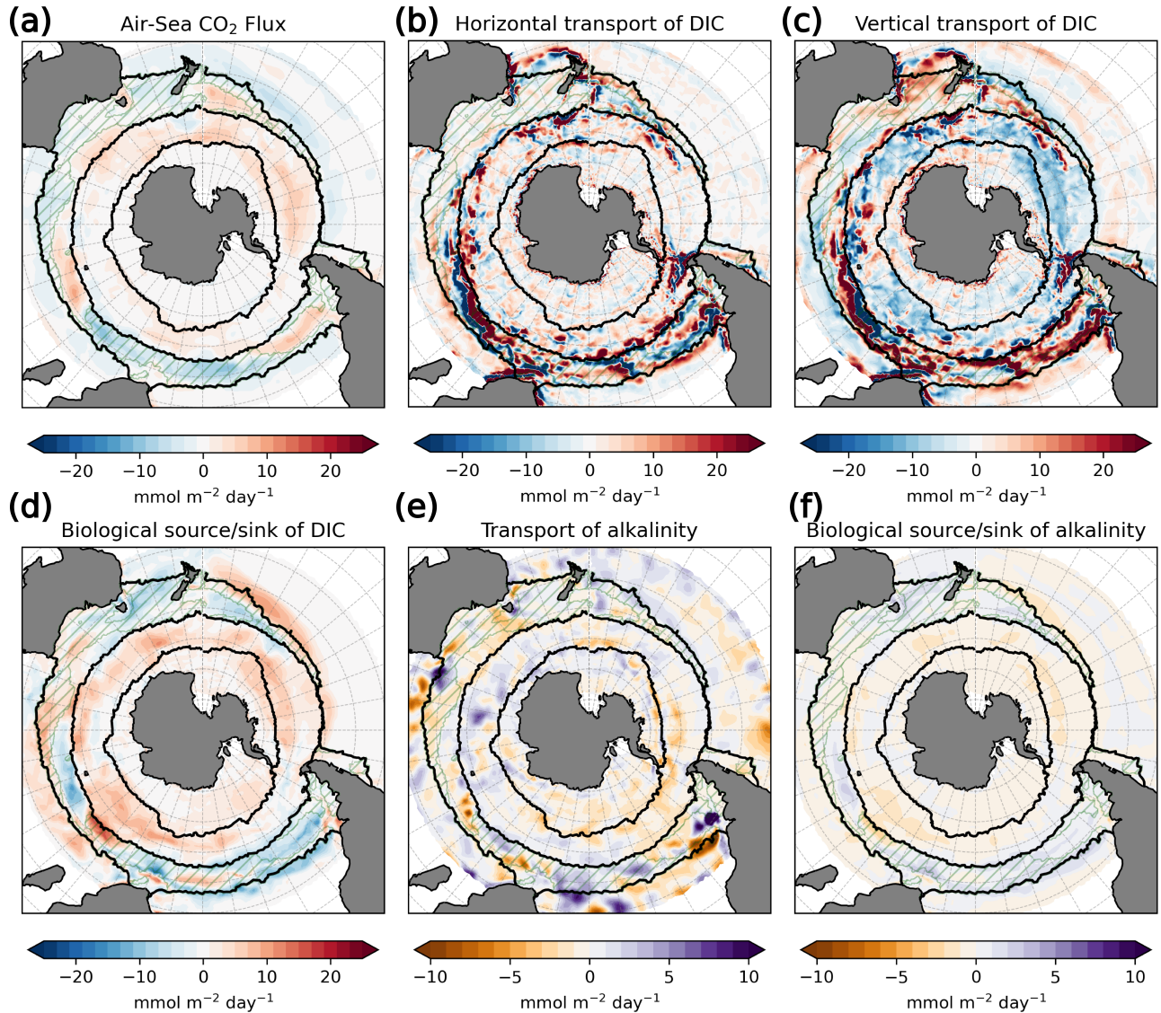
Figure A11. The difference (ASML-FREE) - ASML - FREE of source and sink terms for the ocean's DIC and alkalinity content integrated over 0-190 m in the Southern Ocean in the year 2020. Transport terms include advection and diffusion of DIC and alkalinity. Biological terms for DIC are the sum of: photosynthesis, respiration, remineralization of dissolved organic carbon, and formation and dissolution of calcite. Biological terms for alkalinity are the sum of: nitrogen assimilation and remineralization, and formation and dissolution of calcite.
