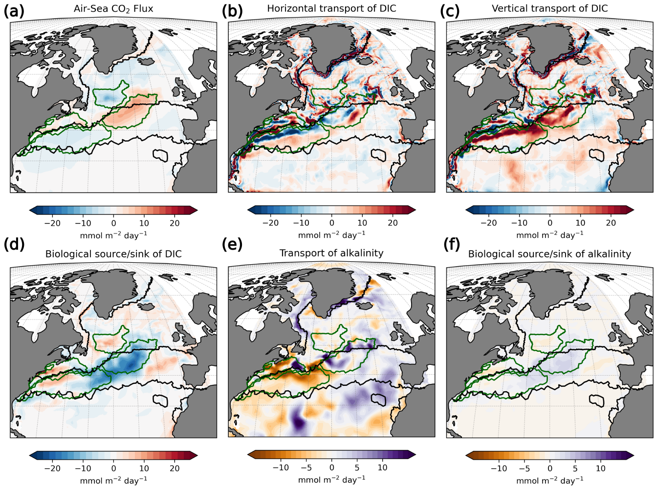
Figure A16. The difference (\text{ASML-FREE}) - \text{ASML-FREE} of source and sink terms for the ocean's DIC and alkalinity content integrated over 0-190 m in the North Atlantic in the year 2020. Transport terms include advection and diffusion of DIC and alkalinity. Biological terms for DIC are the sum of: photosynthesis, respiration, remineralization of dissolved organic carbon, and formation and dissolution of calcite. Biological terms for alkalinity are the sum of: nitrogen assimilation and remineralization, and formation and dissolution of calcite.
