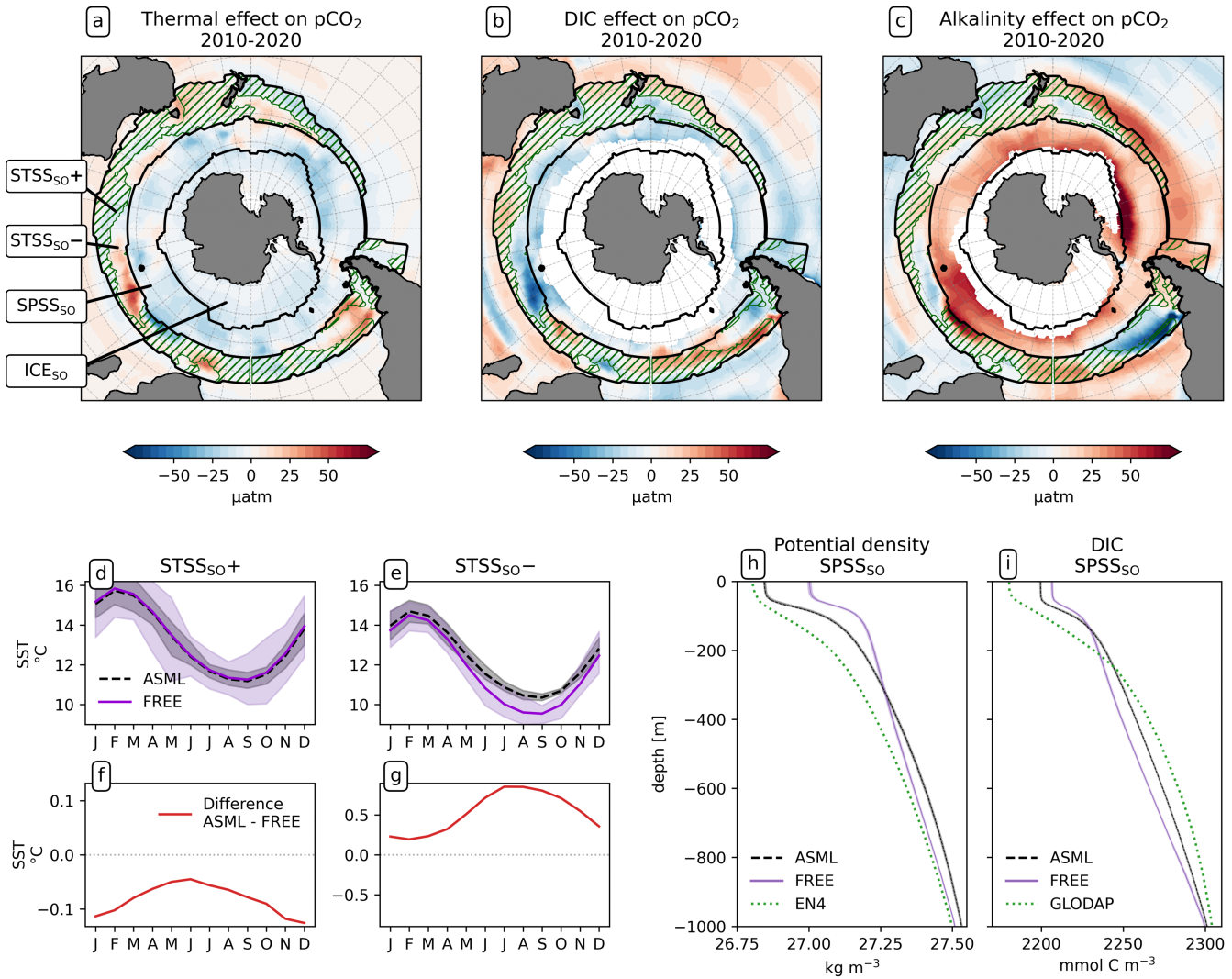
Figure 6. Drivers of the effects of data assimilation on air-sea \text{CO}_2 fluxes \text{pCO}_2 in the Southern Ocean. Panels a, b and c show the effects of SST, DIC and alkalinity differences between the ASML and FREE \text{ASML} - \text{FREE} simulations on surface \text{pCO}_2 , where positive denotes an increase in \text{pCO}_2 . Hatching Additionally, hatching inside the \text{STSS}_{50} indicates where net \text{pCO}_2 is increased through the assimilation ( \text{STSS}_{50+} ). (d and e) Seasonal cycle of SST averaged over the regions \text{STSS}_{50+} and \text{STSS}_{50-} , and (f and g) the difference between ASML and FREE \text{ASML} - \text{FREE} for each region. (h) Potential density profiles for the \text{SPSS}_{50} , with FREE (violet line) and ASML (dashed black line) based on daily T and S, and with EN4-OA (dotted green line) based on monthly T and S. (i) DIC profiles for the \text{SPSS}_{50} , showing FREE (violet line), ASML (dashed black line) from 2010-2020 and climatological DIC from GLODAP. Shading in d, e, h and i indicates the range of ensemble members in the year 2020.
