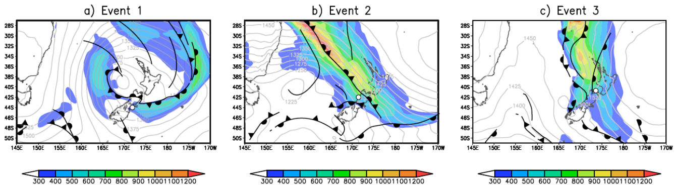
110 Figure 1: IVT magnitude (shading) and 850 hPa geopotential (grey isolines), with analysis of frontal activity for each of the three case study events overlain. Event 1: 0000 UTC, 30/05/2021; Event 2: 1200UTC, 16/07/2021; Event 3: 1200UTC, 16/08/2022. The white dots with black outline indicate the approximate location of peak flooding for each event.
