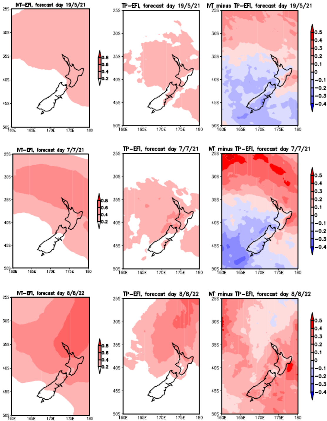
160 Figure 3: 10–15-day EFI forecast for TP, IVT, and IVT minus TP difference for Event 1 (upper row), Event 2 (middle row) and Event 3 (lower row).
