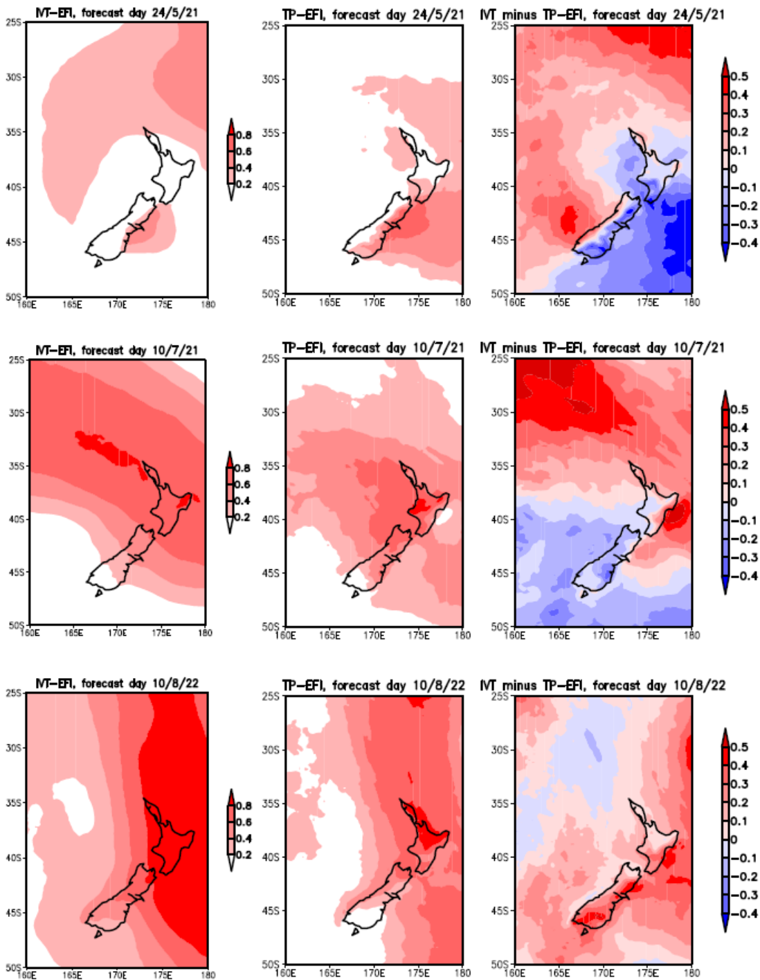
125 Figure 2: 7–9-day EFI forecast for TP, IVT, and IVT minus TP difference for Event 1 (upper row), Event 2 (middle row) and Event 3 (lower row).
