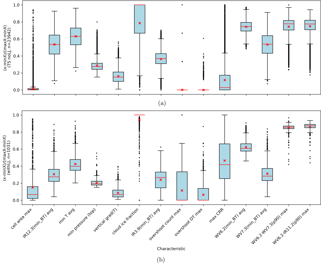
Figure 2. Normalized characteristics for (a) the thunderstorms (TSs) without LJs and (b) the storms with LJs (singleLJ + multiLJ). Red cross shows the mean, red line the median of each characteristic.
