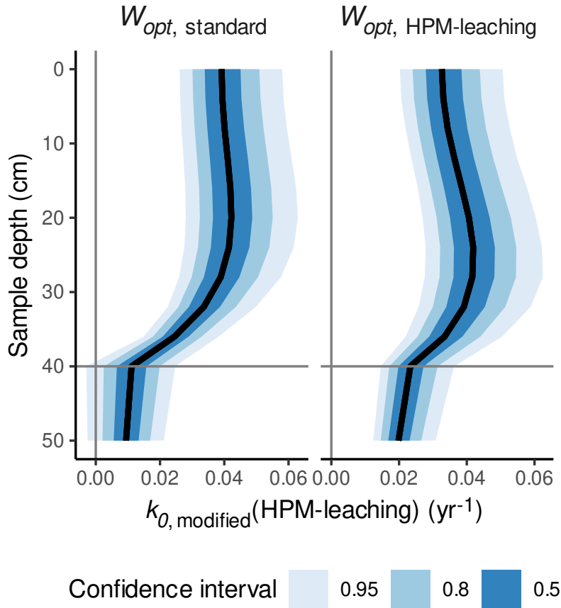
Figure 7. Decomposition rates predicted with HPM-leaching ( k_{0, \text{modified}}(\text{HPM-leaching}) ) for S. fuscum (hummocks), using either the standard value for W_{\text{opt}} or the W_{\text{opt}} value estimated by HPM-leaching versus depth of the litter below the peat surface. The horizontal line is the average water table depth. Shaded areas are central confidence intervals with probabilities given in the figure legend.
