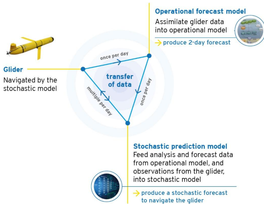
Fig.5. A schematic illustration of a digital twin system navigating fully autonomous gliders to areas of observational interest. The Figure is reproduced from Ford et al (2022), with a similar scheme also being applied in Partridge et al (2025), in prep. The digital twin system is based on information flowing in all directions: (i) glider observations are being assimilated into the pre-operational forecasting model (i.e. the model is updated by the glider). (ii) The operational model subsequently produces forecasts for a stochastic/ML model, with additional inputs into the stochastic model provided by the glider directly, (iii) The stochastic model then provides the system with a fully autonomous path-planning capacity close to the glider's spatial scale of operations, navigating the glider into the expected areas of observational interest (i.e. the model tells glider "where to go"). This exchange of information then cycles throughout the glider mission.
