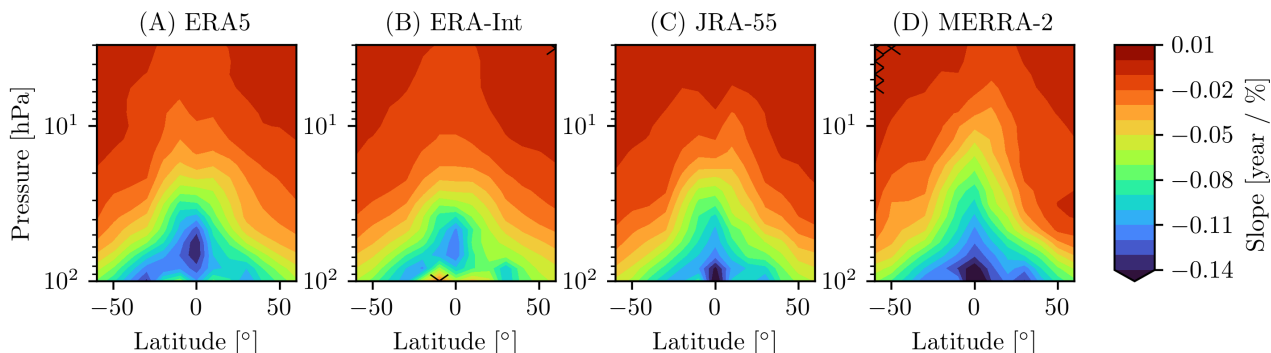
Figure 5. Slope from linear fit to CLaMS AoA and N_2O for 2004–2017. Results are shown for CLaMS driven with four different reanalyses. Hatching denotes statistically insignificant slopes at the 2\sigma level (only MERRA-2 and ERA-Int have hatching, and very few bins are hatched). The hatched bins are at the highest latitudes and pressure levels .
