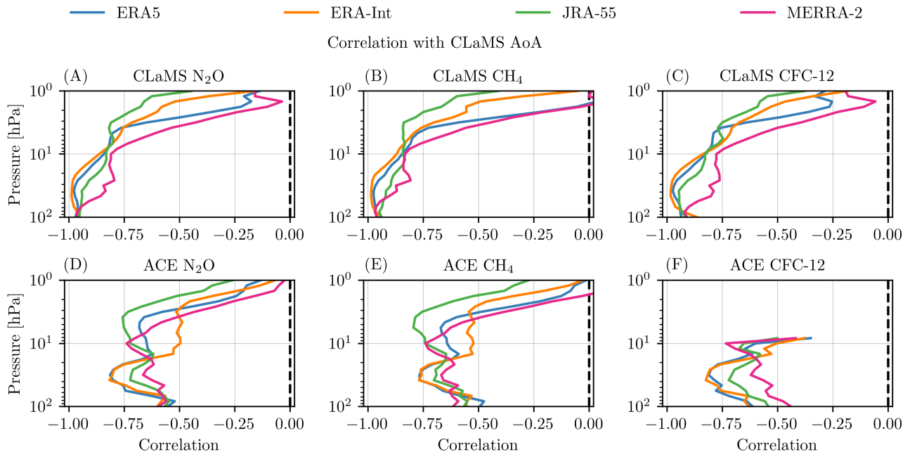
Figure 2. Correlation of \text{N}_2\text{O} , \text{CH}_4 , and CFC-12 with AoA from CLaMS driven with four different reanalyses as a function of pressure level. Top row: VMR anomaly profiles from CLaMS. Bottom row: VMR anomaly profiles from ACE-FTS. All results for SH-NH difference over 2004–2017. CFC-12 observations from ACE-FTS are only available up to 8 hPa.
