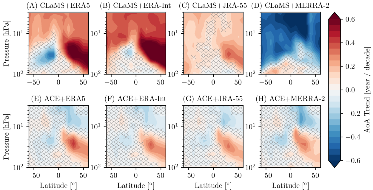
Figure 7. Top row: AoA trends from CLaMS driven with four different reanalyses. Bottom row: AoA trends derived using ACE-FTS retrievals of N 2 O and the relationship between AoA and N 2 O in CLaMS driven with four different reanalyses. All AoA trends are for 2004–2017. Hatching denotes statistically insignificant trends at the 2 \sigma level.
