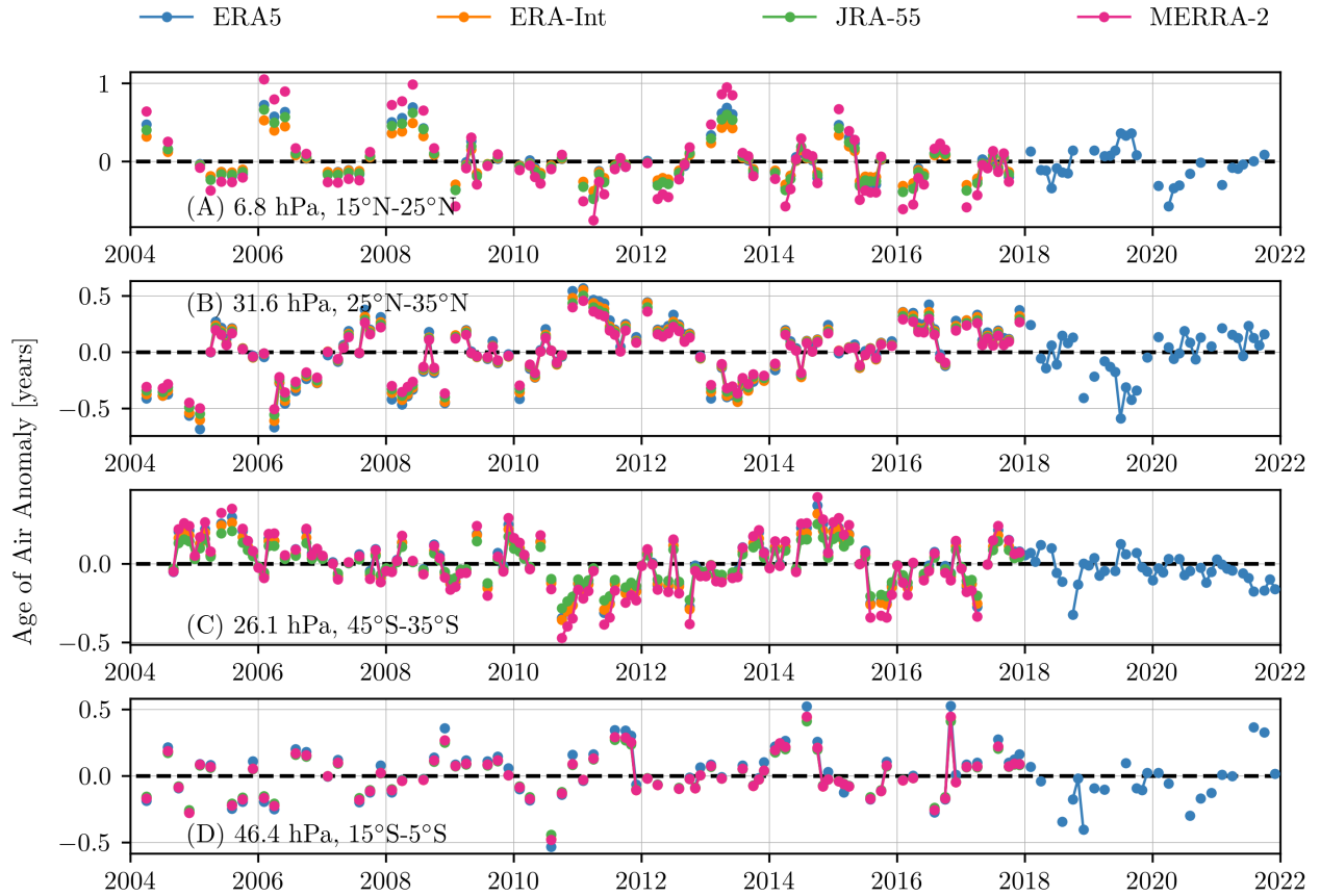
Figure 6. AoA anomaly for four latitude and altitude bins. The AoA anomaly is derived using ACE-FTS retrievals of N_2O and the relationship between AoA and N_2O in CLaMS driven with four different reanalyses
