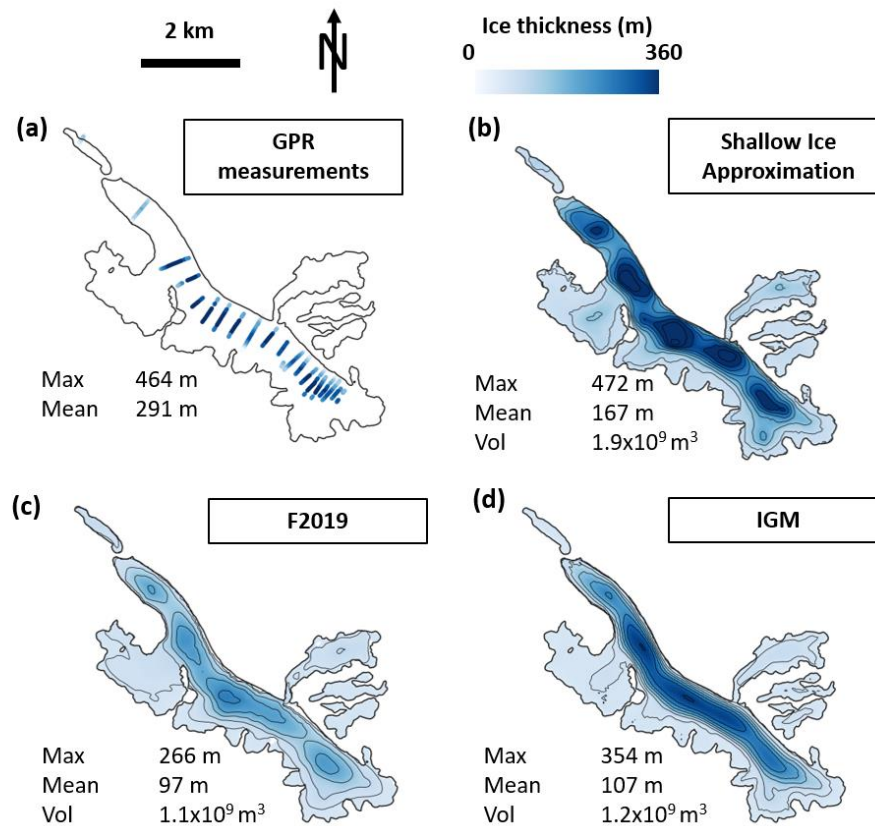
365 Figure 4: (a) Ice thickness from in situ GPR measurements. (b) Distributed ice thickness obtained using the shallow ice approximation. (c) Distributed ice thickness from the Farinotti et al. (2019) estimate. (d) Mean distributed ice thickness from the 100 ice thickness inversions obtained with IGM. The black thickness contour lines are spaced every 50 m. The black glacier outlines were derived from the 08/09/2020 Pléiades orthoimage. The numbers in each panel indicate the maximum and mean thickness and the total glacier volume.
