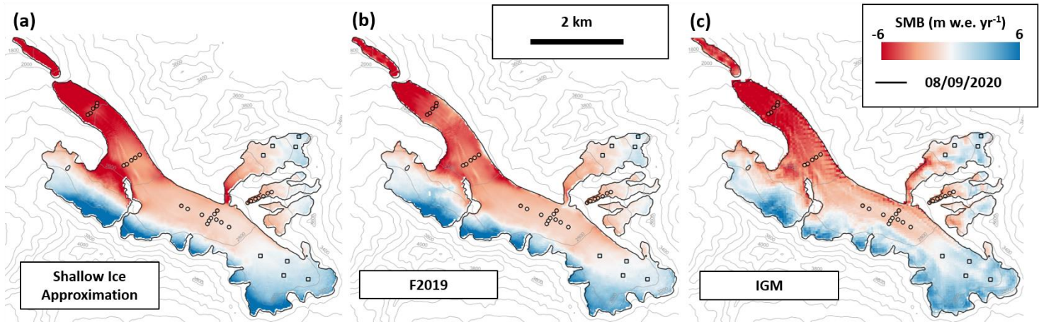
Figure 5: SMB obtained with (a) the SIA, (b) the F2019 and (c) the IGM modelling approaches SMB estimates. The coloured dots indicate the mean annual mass balances over the period 2012-2021 from the stake measurements. The black glacier outlines were derived from a Pléiades orthoimage acquired on 08/09/2020.
