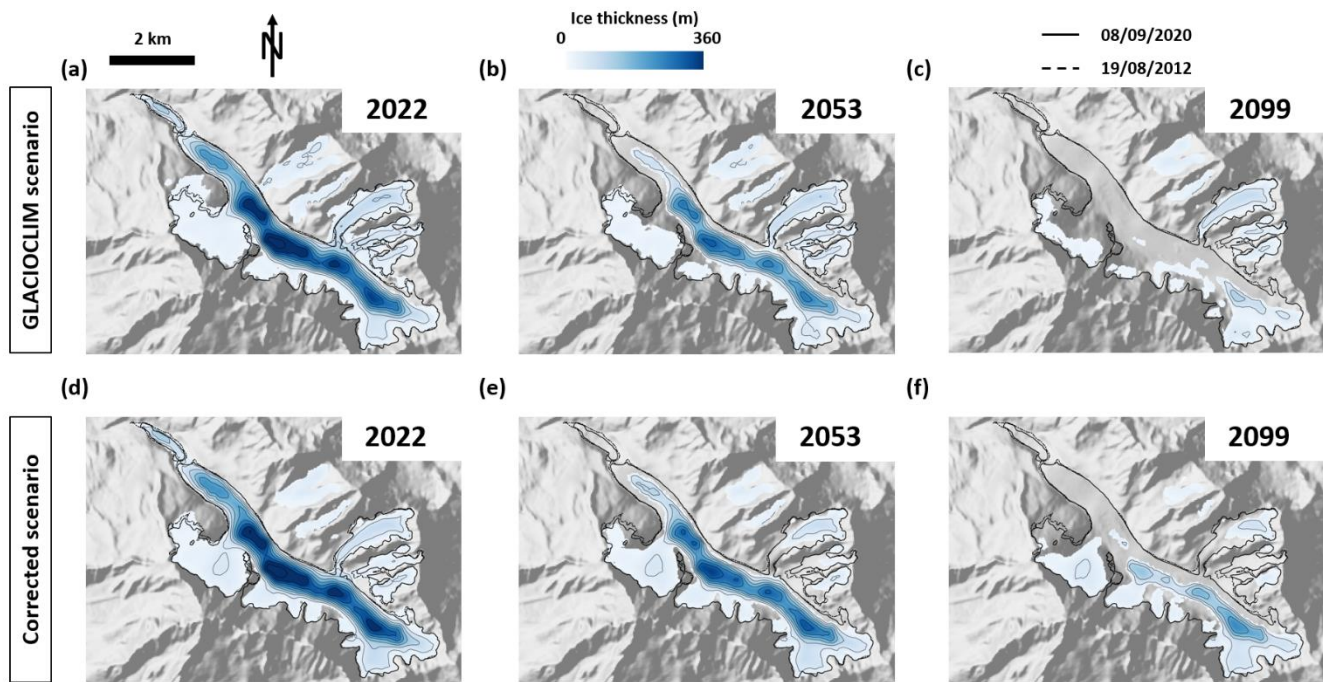
465 470 Figure 9: Distributed ice thickness evolution in the Argentière catchment for the period 2022-2099 using the RCP 4.5 climate scenario for the GLACIOCLIM (a-c) and Corrected (d-f) scenarios. Background is the hillshade of the AW3D30 30 m DEM (Tadono et al., 2014). The black thickness contour lines are spaced every 50 m. The black outlines indicate the glacier outlines manually derived from the 08/09/2020 Pléiades orthoimage, and the dashed outlines show the glacier outlines derived from the 19/08/2012 Pléiades orthoimage.
