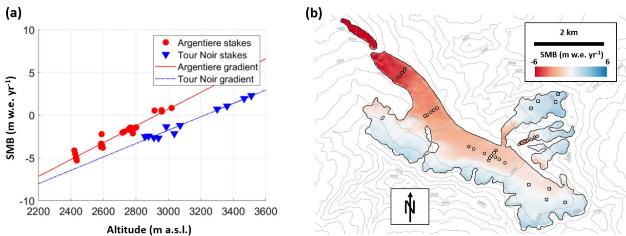
250 Figure 2: (a) average annual SMB for the period 2012-2021 at the stake locations on Argentière Glaciers (red dots) and Tour Noir and Améthystes Glaciers (blue triangles), and corresponding altitudinal SMB gradients. (b) Mean annual 2012-2021 stake measurements at the stake locations (circles indicate stakes in the ablation zone and squares show stakes in the accumulation zone), and mean annual SMB over the period 2012-2021, as obtained from the GLACIOCLIM ETI SMB model (section 2.10). The grey elevation contour lines are spaced every 200 m. The black glacier outlines were derived from a Pléiades orthoimage acquired on 08/09/2020.
