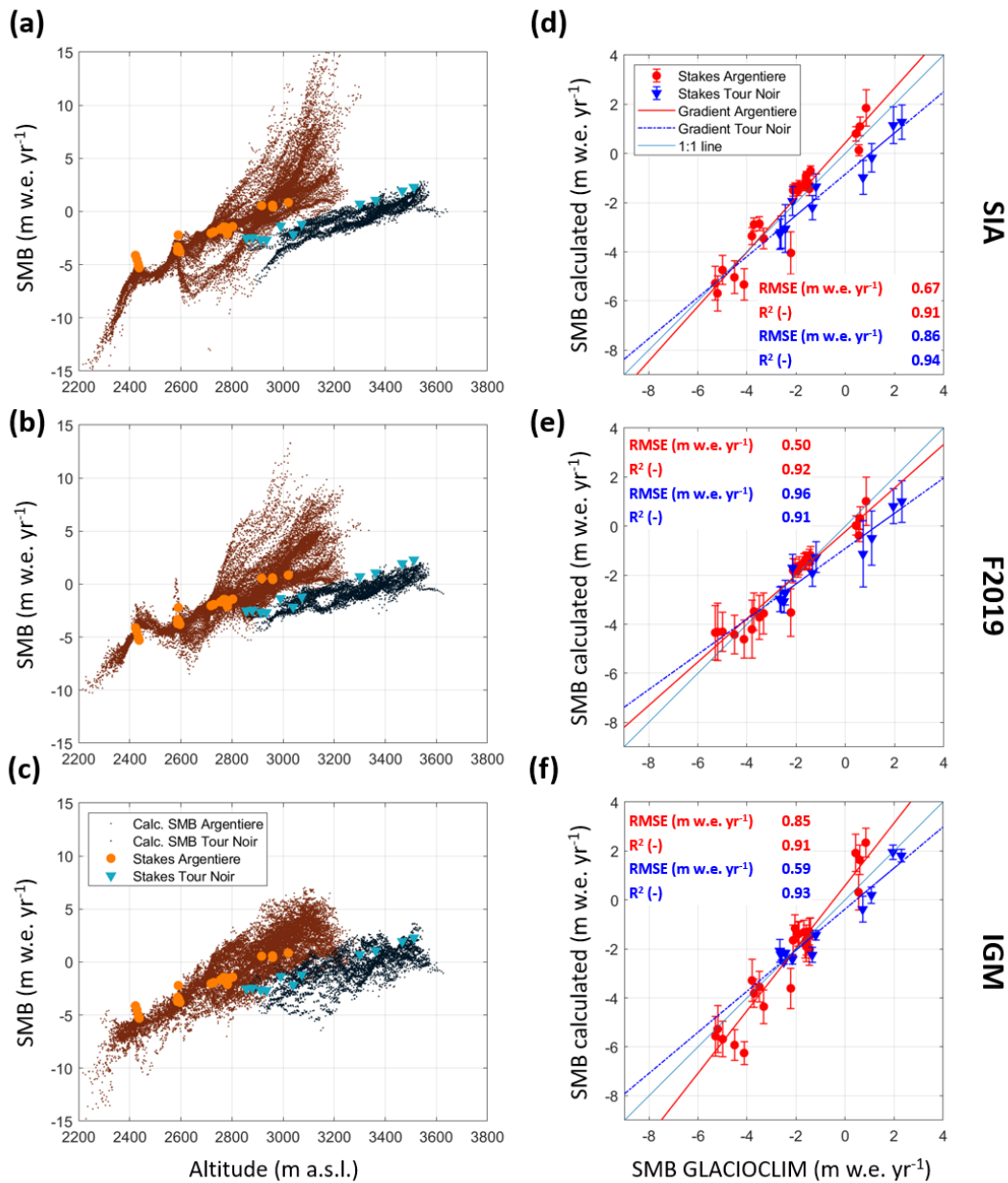
415 Figure 6: (a-c) Altitudinal patterns of mean annual SMB calculated with the different modelling approaches and of the mean annual mass balances over the period 2012-2021 from the stake measurements. (d-f) Direct comparison of mean annual SMB calculated with the different modelling approaches, with the mean annual mass balances over the period 2012-2021 from the stake measurements, at the stake locations.
