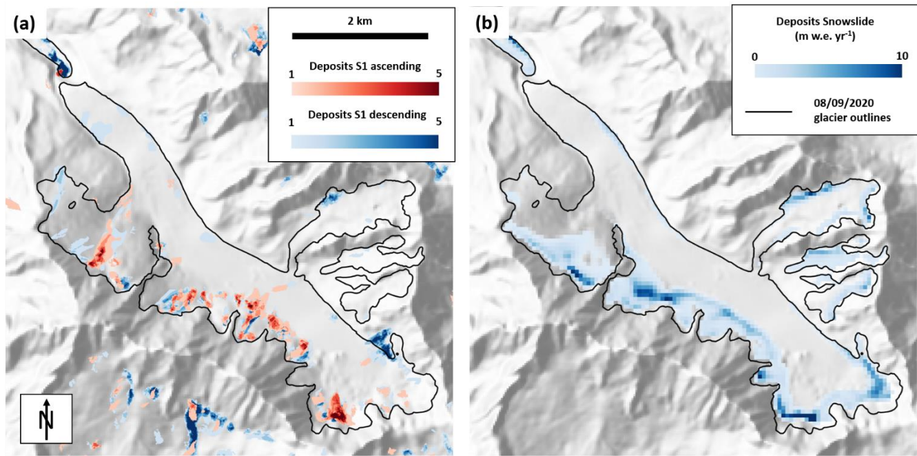
440 Figure 7: (a) Total number of detected avalanches on Argentière Glacier for the period 11/2016-10/2021 using Sentinel-1 synthetic aperture radar images at 6 days intervals, both in the ascending (red) and descending (blue) orbits. Data from Kneib et al. (2023). (b) Average yearly snow accumulation by avalanches predicted by the SnowSlide model for the period 2012-2021. Background image is the hillshade of the AW3D30 30 m DEM (Tadono et al., 2014). The black glacier outlines were derived from the 08/09/2020 Pleiades orthoimage.
