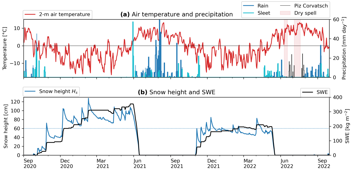
Figure 5. Meteorological conditions. (a) Air temperature (daily mean) and precipitation (daily sum). (b) Snow height and SWE. Rain and sleet (mixed precipitation) separated based on a wet-bulb temperature threshold of 2^{\circ}\text{C} (Amschwand et al., 2024a). A snow height of h_s = 60 cm (measured on a windswept ridge) discriminates between a semi-closed and a closed/insulating snowpack (cf. Fig. 8). Precipitation data at station Piz Corvatsch from MeteoSuisse.
