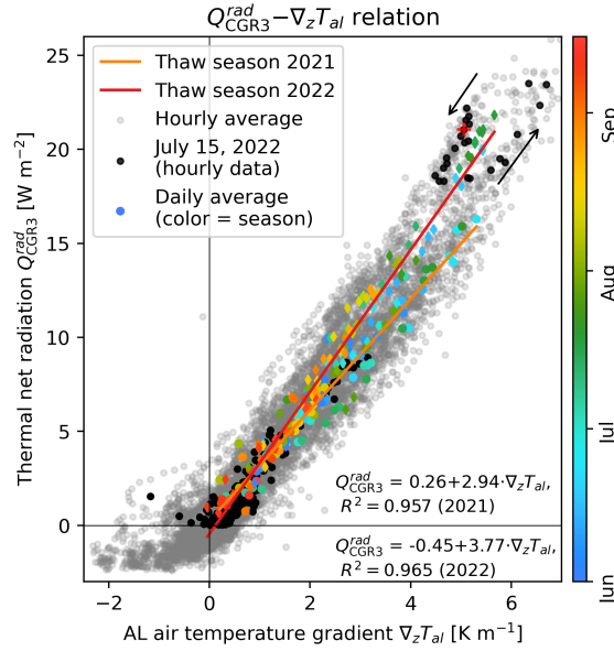
Figure 9. Thermal net radiation Q_{\text{CGR3}}^{\text{rad}} vs. vertical AL air temperature gradient \nabla_z T_{\text{al}} . Daily averages are highly correlated (Eq. 17). Hourly values show a diurnal loop.
