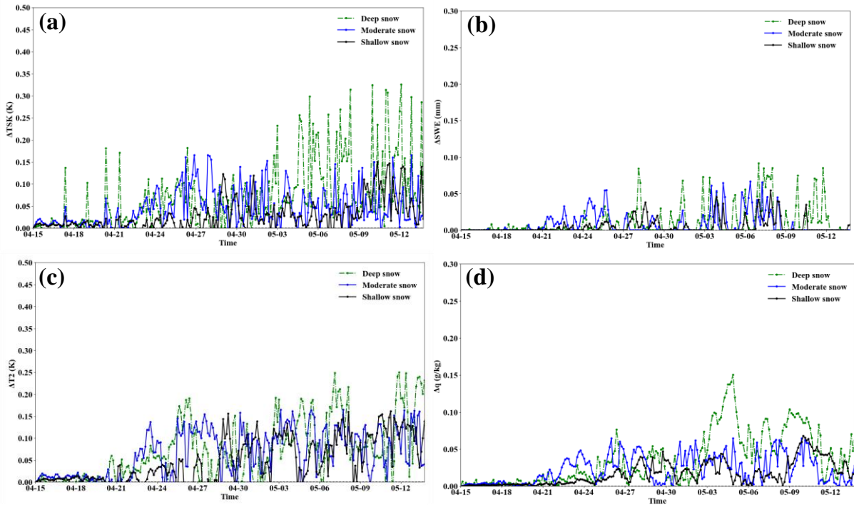
560 Figure 11. Averaged three-hour on-line simulation results of the changes (a) surface temperature (K) (b) snow melt (mm h -1 ) (c) 2-m air temperature (K) and (d) 2-m specific humidity (g kg -1 ) induced by BC deposition in different snow layers.
