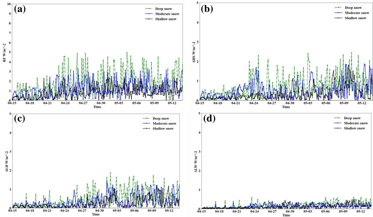
510 Figure 9. Averaged three-hour on-line simulation results of the change in the (a) RF ( W m^{-2} ) (b) sensible heat flux (HS) ( W m^{-2} ) (c) latent heat flux (LH) ( W m^{-2} ) (d) surface upwelling longwave radiation (LW) ( W m^{-2} ) induced by BC deposition in different snow layers. Positive (negative) values indicate gain (loss) by the atmosphere apart from RF.
