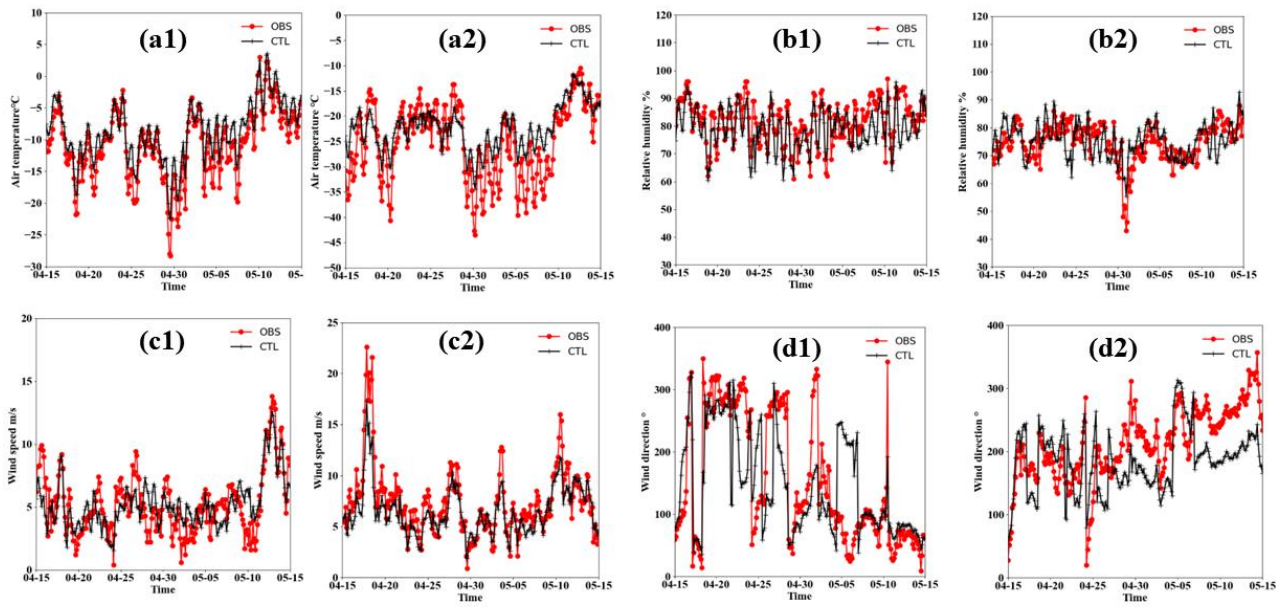
350 Figure 2. Time series of observed and simulated three-hourly average 2-m temperature ( ^{\circ}\text{C} ), 2-m relative humidity ( \% ), 10-m wind speed ( \text{m s}^{-1} ), and 10-m wind direction ( ^{\circ} ) at the Barrow station (a1-d1) and Summit station (a2-d2) from 15 April to 15 May 2020.
