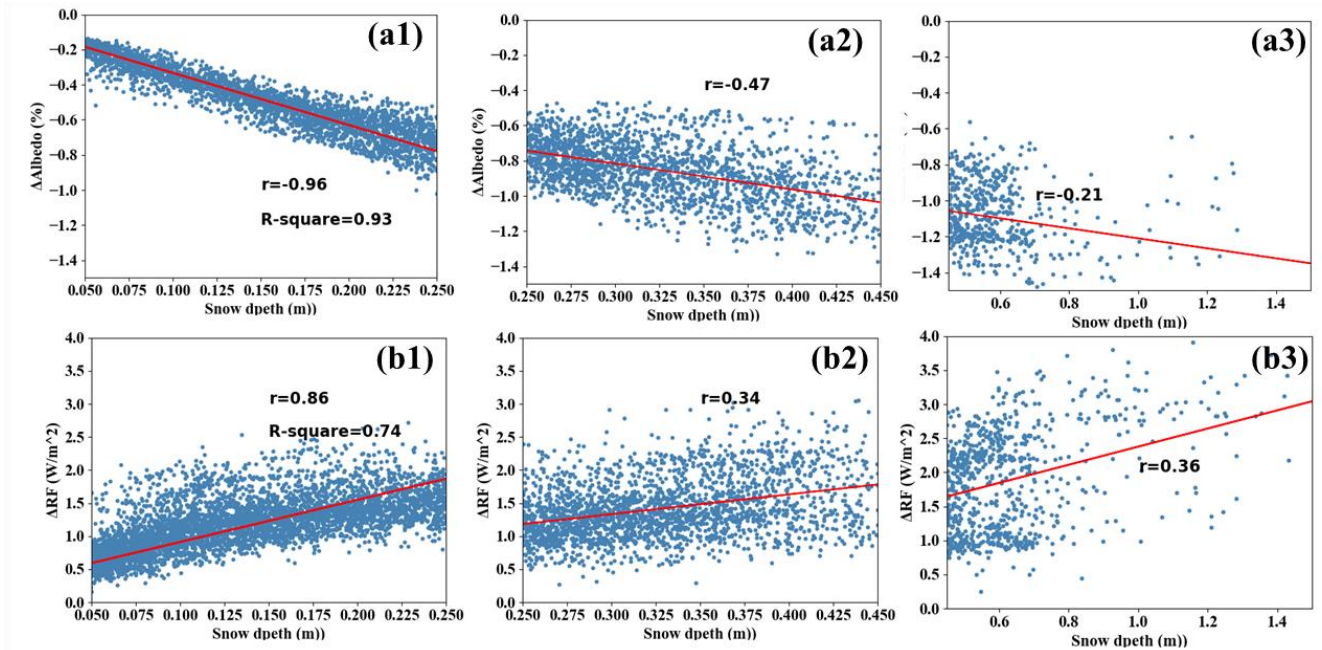
Figure 8. Relationship between (a1-a3) the snow albedo reduction (%) induced by BC deposition and snow depth (m) and between (b1-b3) the RF ( \text{W m}^{-2} ) and snow depth (m)
