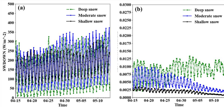
515 Figure 10. Averaged three-hour on-line simulation results of the (a) incident solar radiation ( \text{W m}^{-2} ) and (b) snow albedo reduction induced by BC deposition in different snow layers.
