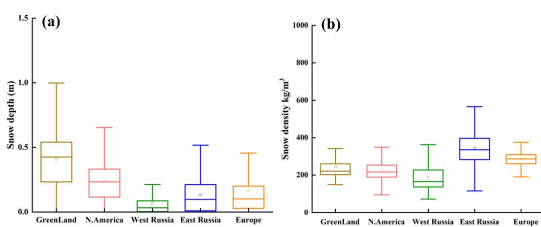
Figure 7. Distribution of (a) snow depth (m) and (b) snow density ( \text{kg m}^{-3} ) across different Arctic regions.
