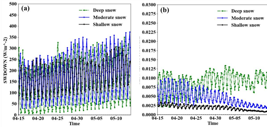
465 Figure 10. Averaged three-hour on-line simulation results of the (a) incident solar radiation ( W m^{-2} ) and (b) snow albedo reduction induced by BC deposition in different snow layers.
