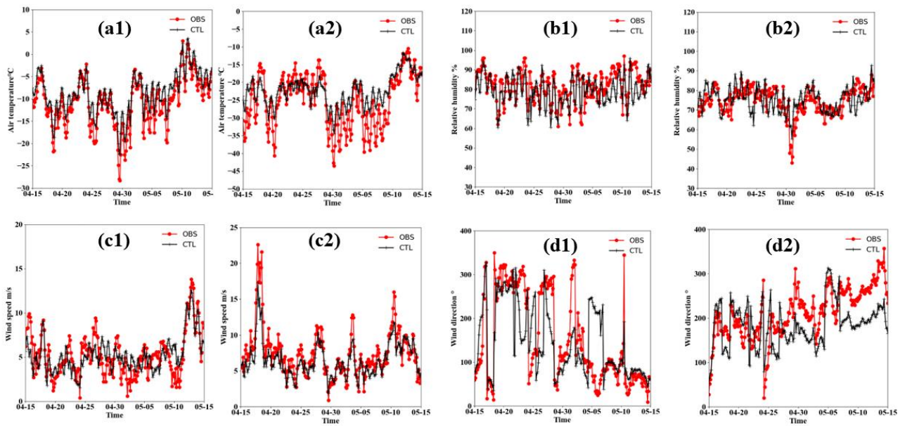
Figure 2. Time series of observed and simulated three-hourly average 2-m temperature ( ^{\circ}\text{C} ), 2-m relative humidity ( \% ), 10-m wind speed ( \text{m s}^{-1} ), and 10-m wind direction ( ^{\circ} ) at the Barrow station (a1-d1) and Summit station (a2-d2) from 15 April to 15 May 2020.
