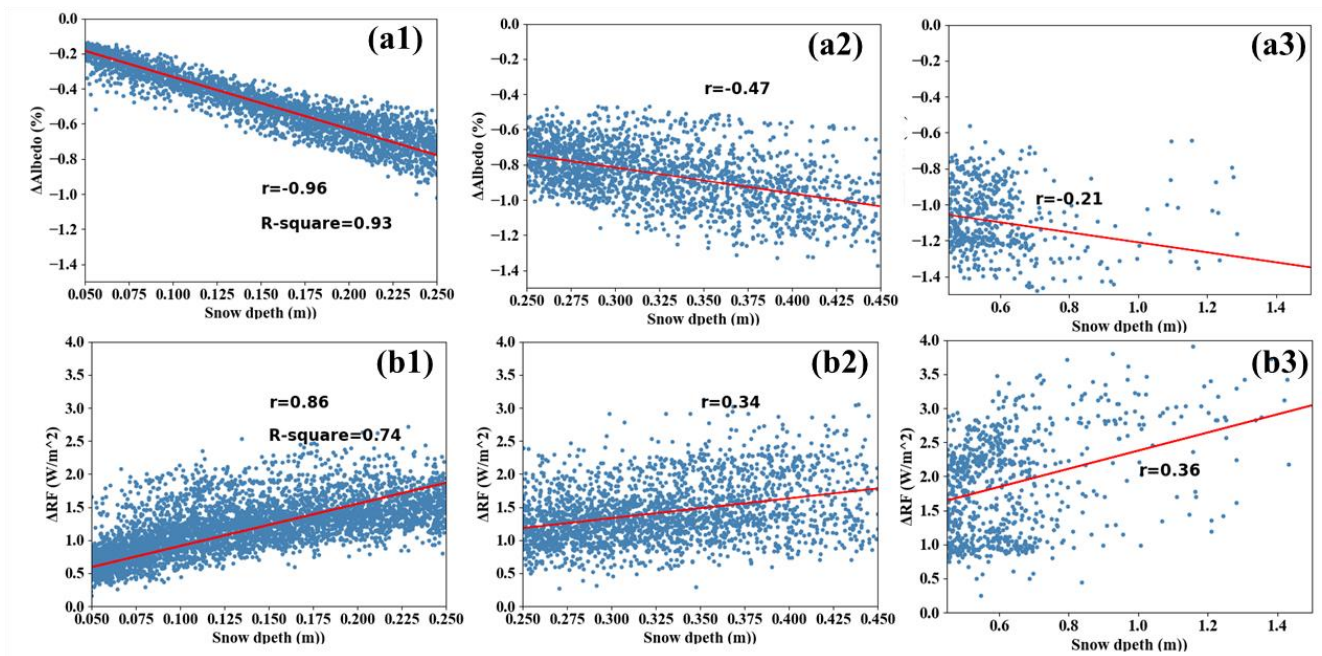
455 Figure 8. Relationship between (a1-a3) the snow albedo reduction (%) induced by BC deposition and snow depth (m) and between (b1-b3) the RF ( W m^{-2} ) and snow depth (m)
