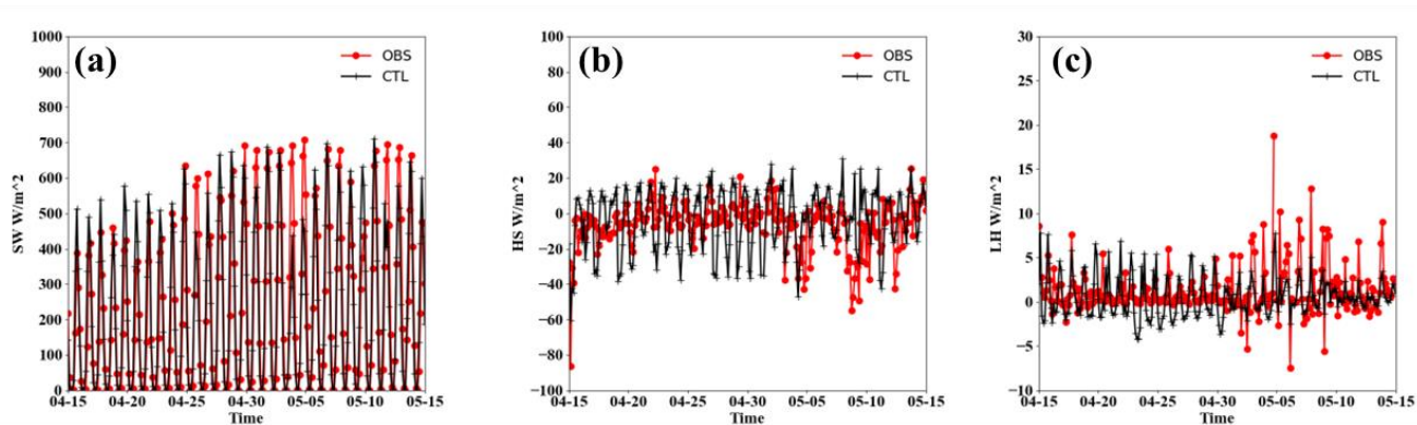
Figure 3. Time series of observed and simulated three-hourly average (a) incident solar radiation (SW) ( \text{W m}^{-2} ), (b) sensible heat flux (HS) ( \text{W m}^{-2} ) and (c) latent heat flux (LH) ( \text{W m}^{-2} ) in Alaska from 15 April to 15 May 2020. Positive (negative) values indicate gain (loss) by the atmosphere.
