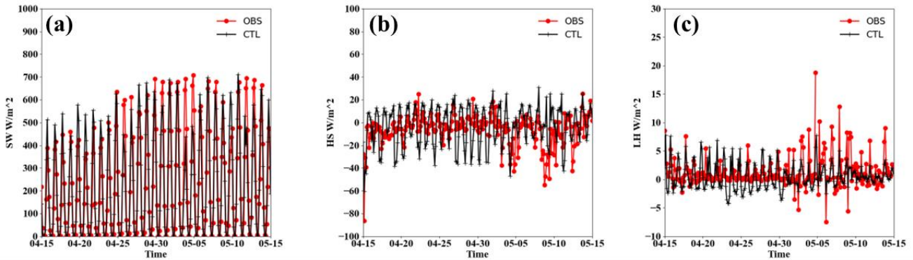
360 Figure 3. Time series of observed and simulated three-hourly average (a) incident solar radiation (SW) ( \text{W m}^{-2} ), (b) sensible heat flux (HS) ( \text{W m}^{-2} ) and (c) latent heat flux (LH) ( \text{W m}^{-2} ) in Alaska from 15 April to 15 May 2020. Positive (negative) values indicate gain (loss) by the atmosphere.
