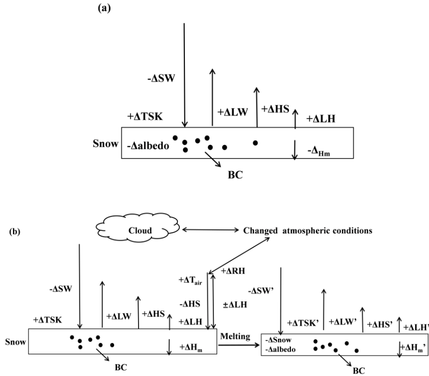
Figure 14. Conceptual diagram of SDE due to BC deposition on the surface energy exchange process: (a) off-line (b) on-line
