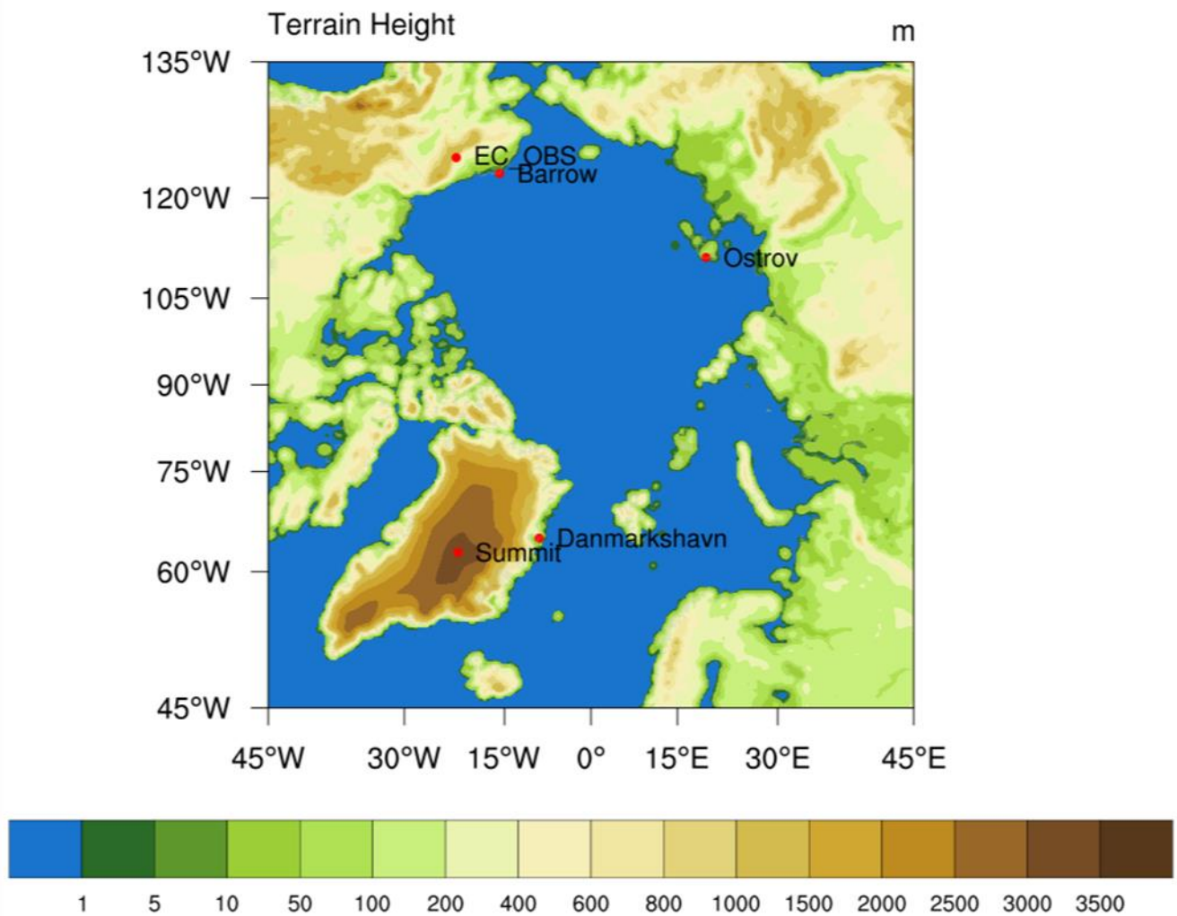
295 Figure 1. Polar-WRF domain and terrain height. The red circles indicate the locations of the observation sites chosen for model evaluation in this study. The data from the Barrow and Summit stations are used to validate the
