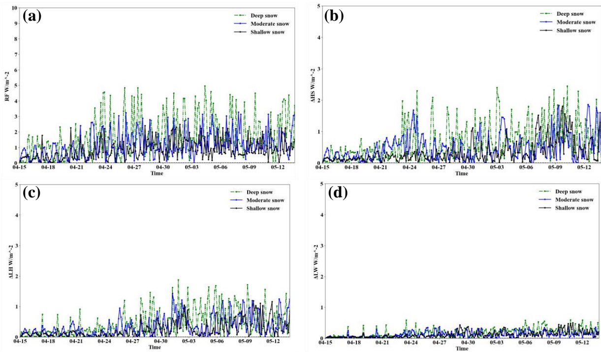
515 Figure 9. Averaged three-hour on-line simulation results of the change in the (a) RF ( \text{W m}^{-2} ) (b) sensible heat flux (HS) ( \text{W m}^{-2} ) (c) latent heat flux (LH) ( \text{W m}^{-2} ) (d) surface upwelling longwave radiation (LW) ( \text{W m}^{-2} ) induced by BC deposition in different snow layers. Positive (negative) values indicate gain (loss) by the atmosphere apart from RF.
