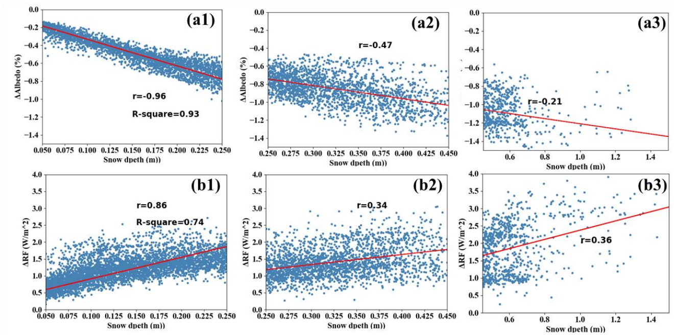
510 Figure 8. Relationship between (a1-a3) the snow albedo reduction (%) induced by BC deposition and snow depth (m) and between (b1-b3) the RF ( \text{W m}^{-2} ) and snow depth (m)
