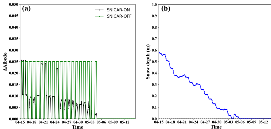
Figure 12. (a) Averaged three-hour simulation results of the snow albedo reduction by BC deposition and (b) snow depth change during the period.
