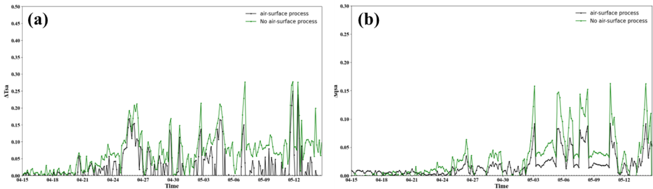
645 Figure 134. Differences between the (a) temperature (K) and (b) specific humidity ( \text{g kg}^{-1} ) of the surface and air during the air-surface exchange process (black line) and without the air-surface process (green line)
