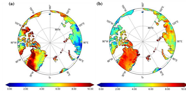
410 Figure 45. Mean snow albedo reduction ( 10^{-3} ) induced by BC deposition in (a) SNICAR-OFF, and (b) SNICAR-ON.
