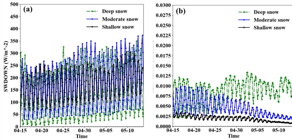
Figure 10.11. Averaged three-hour on-line simulation results of the (a) incident solar radiation ( \text{W m}^{-2} ) and (b) snow albedo reduction induced by BC deposition in different snow layers.
