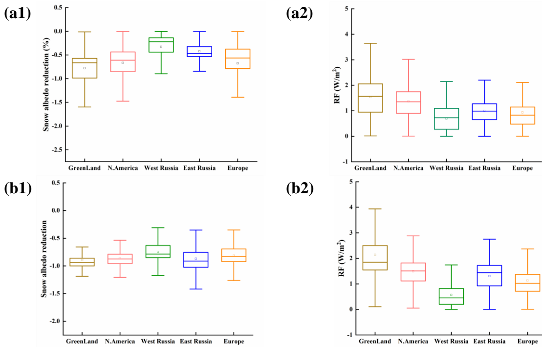
Figure 67. Snow albedo reduction and RF induced by BC in snow from SNICAR-OFF (a1-a2) and SNICAR-ON (b1-b2) across different Arctic regions.
