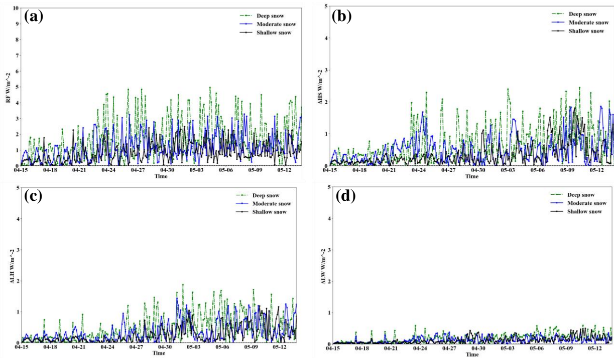
Figure 109. Averaged three-hour on-line simulation results of the change in the (a) RF ( W m^{-2} ) (b) sensible heat flux (HS) ( W m^{-2} ) (c) latent heat flux (LH) ( W m^{-2} ) (d) surface upwelling longwave radiation (LW) ( W m^{-2} ) induced by BC deposition in different snow layers. Positive (negative) values indicate gain (loss) by the atmosphere apart from RF.
