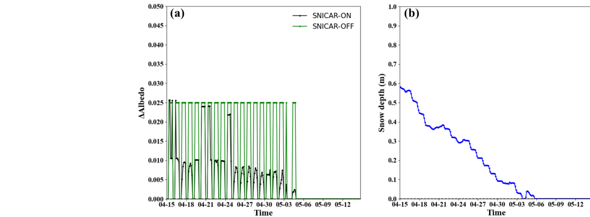
585 Figure 12.13. (a) Averaged three-hour simulation results of the snow albedo reduction by BC deposition and (b) snow depth change during the period.
