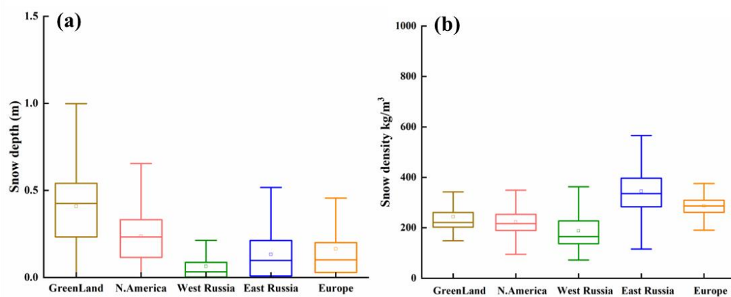
500 Figure 78. Distribution of (a) snow depth (m) and (b) snow density ( \text{kg m}^{-3} ) across different Arctic regions.
