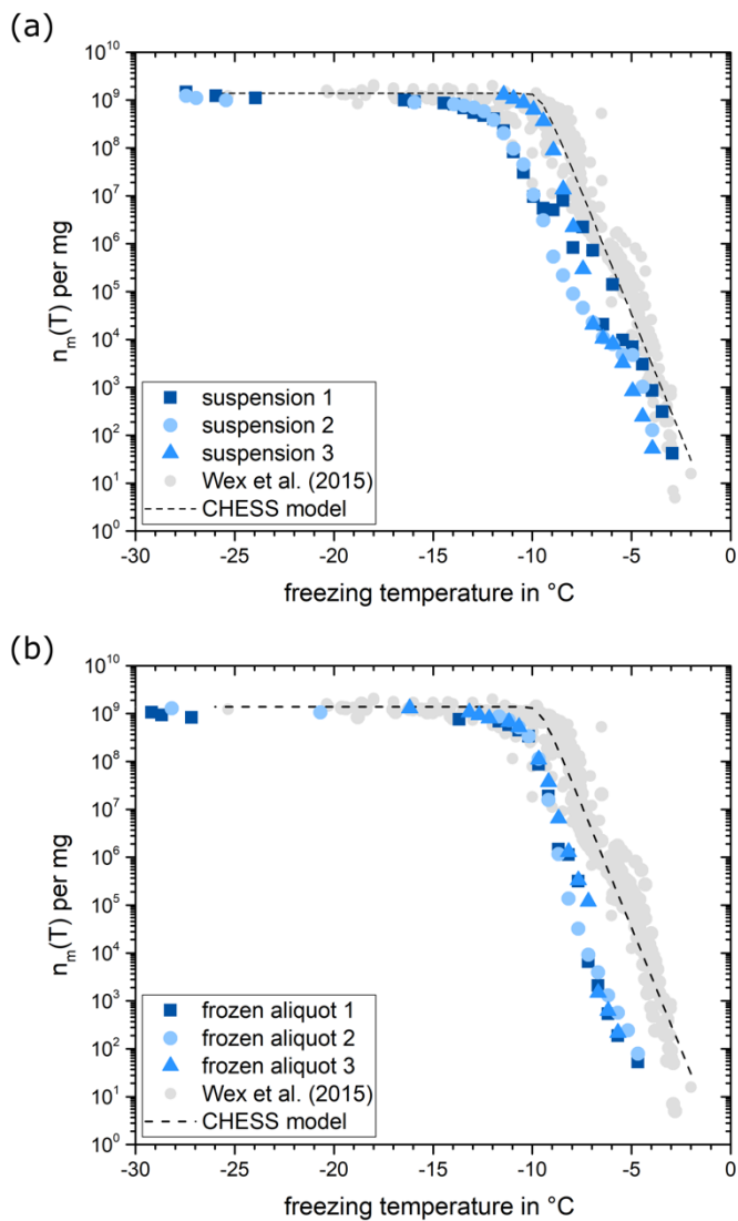
Figure 5: (a) Number of INPs per mg Snomax measured for suspensions with 10^{-2} mg \text{ml}^{-1} to 10^{-7} mg \text{ml}^{-1} Snomax prepared freshly on three different days. The data was binned in 0.5 ^{\circ}\text{C} temperature bins. Grey data points represent the results from various ice nucleation instruments investigated by Wex et al. (2015). The dashed line is based on the CHES model by Hartmann et al. (2013). (b) The same is shown as in (a) but with the Snomax suspension that was prepared once, stored frozen in aliquots, and the measurement was repeated on freshly thawed aliquots three times.
