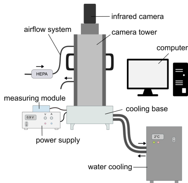
105 Figure 1: Schematic drawing of the micro-PINGUIN instrument.
