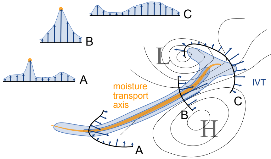
Figure 1. Illustration of the detection method. Blue contours shading and vectors show the magnitude and direction of the vertically integrated water vapor vapour transport (IVT). The black lines marked A, B, and C are cross sections perpendicular to the local IVT direction. Well-defined maxima in the local IVT along the sections are marked by yellow circles in A and B; these well-defined maxima are then connected to form the yellow moisture transport axis line. Black contours indicate isobars, and the labels L and H mark a cyclone and an anticyclone, respectively.
