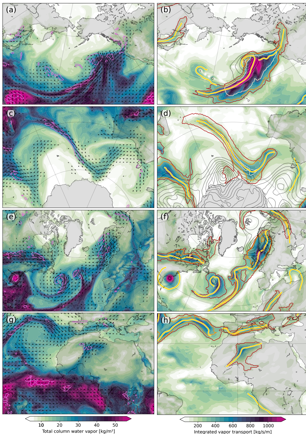
Figure 2. Snapshots of moisture transport axis occurrence. Panels (a-d) show atmospheric river cases discussed by Lora et al. (2020) by-on 5 November 2006, 09Z, and 14 November 2006, 09Z, respectively, (e,f) the strongest river case listed in Azad and Sorteberg (2017) on 14 September 2005, 00Z, and (g,h) a moisture transport axis over the Saharan Desert on 15 December 2017, 06 UTC. The left column shows total column water vapor [kg/m 2 ] (shading), IVT (arrows), and total precipitation (pink contour, 1 mm/h). The right column shows the magnitude of IVT [kg/s/m]. Black contours show sea-level pressure below 1010hPa in steps of 5hPa. Red, orange, and pale red contours show the number of atmospheric river detections in the ARTMIP-ERA5 dataset with contours at 1, 3, and 6 of 6 available global algorithms. Finally, the yellow lines show detected moisture transport axes.
