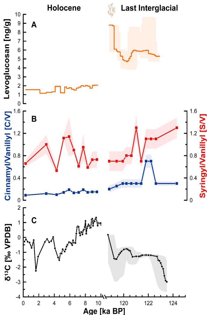
Figure 3: (A) Median levoglucosan concentration (orange line) with 95% confidence intervals (shaded area). (B) Median C/V (blue) and S/V (red) ratios with 1σ error margins (shaded area). (C) Median δ¹³C (black) with 95% confidence intervals (shaded area). Confidence intervals were derived from 2000 Monte Carlo simulations in the COPRA age modelling calculations and incorporate the interpolation and transfer of age uncertainty into the proxy domain. Error was negligible during the Holocene in plots A, B (CV) and C.
