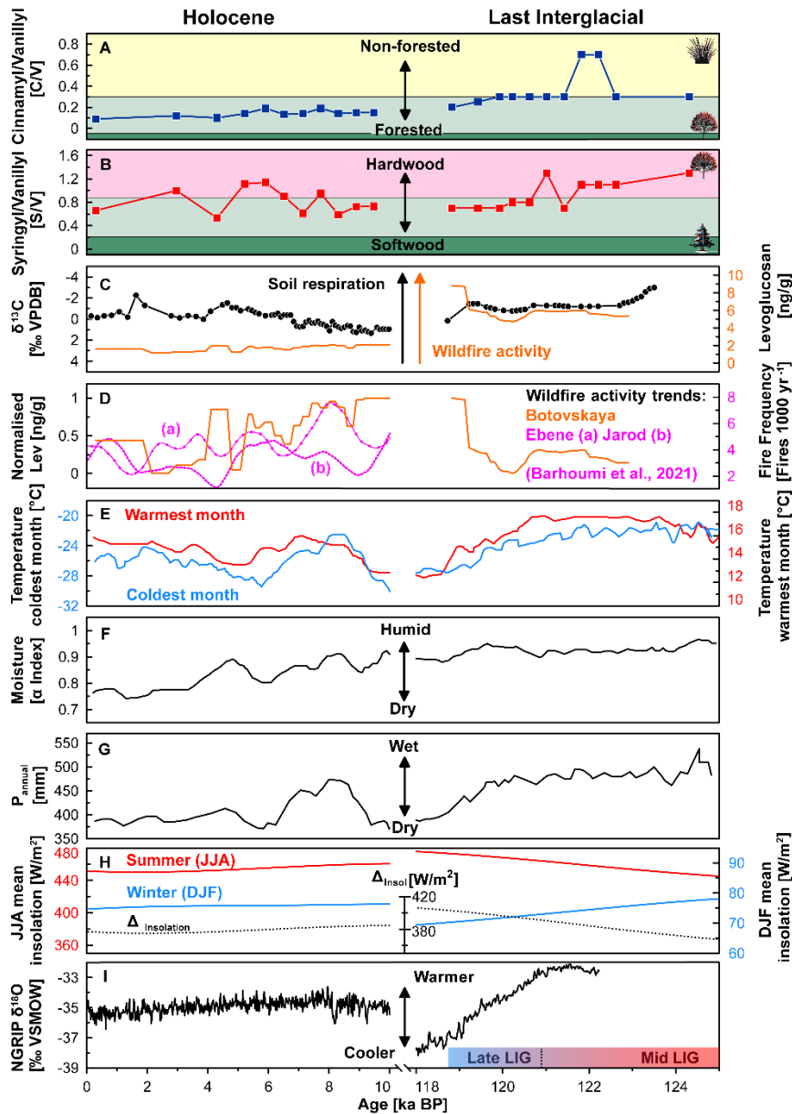
355 Figure 5: Vegetation (A, B), wildfire and climate (C, D) signals derived from Botovskaya cave shown with published regional and hemispheric records of vegetation and climate (D-I). (A) Dark green shading indicates predominantly forested vegetation, yellow shading open vegetation, and yellow/green mixed vegetation. (B) Pink shading indicates hardwood, dark green softwood and pink/green mixed vegetation. (C) The \delta^{13}\text{C} record reflects local hydrological conditions and soil respiration, with lower values indicating wetter conditions and increased soil respiration. (D) Normalised levoglucosan levels highlight multi-centennial trends during the LIG and the Holocene, and local wildfire records (Barhoumi et al., 2021) from lake Ebene (a) and Jarod (b) present fire frequency trends for the Holocene. Lake Baikal pollen records (Tarasov et al., 2007) include temperatures of the warmest and coldest 360
