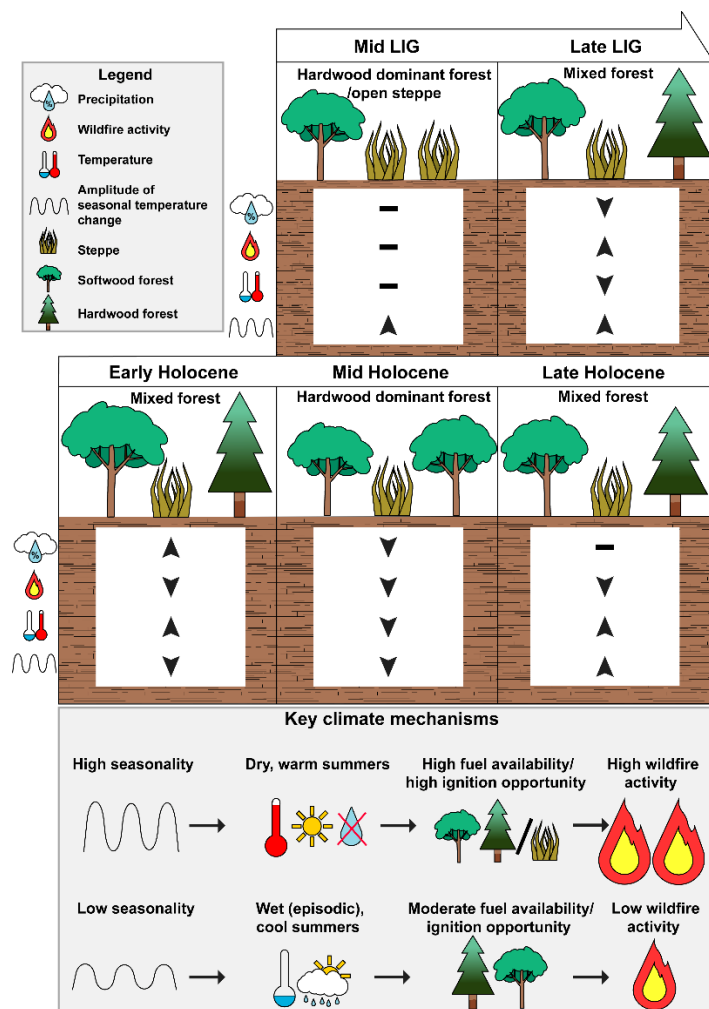
Figure 6: Schematic detailing the general trends summarised in Fig. 5. The arrows and horizontal lines in the upper (LIG) and middle (Holocene) panels summarise the overall trend of each parameter (precipitation, wildfire activity, temperature, and seasonal temperature change) with up, down, and horizontal lines denoting increasing, decreasing, and stable trends respectively. The lower panel summarises the general mechanisms we identified that support wildfire activity and specify the hydrological and environmental parameters leading to both low and high wildfire activity in southern Siberia.
