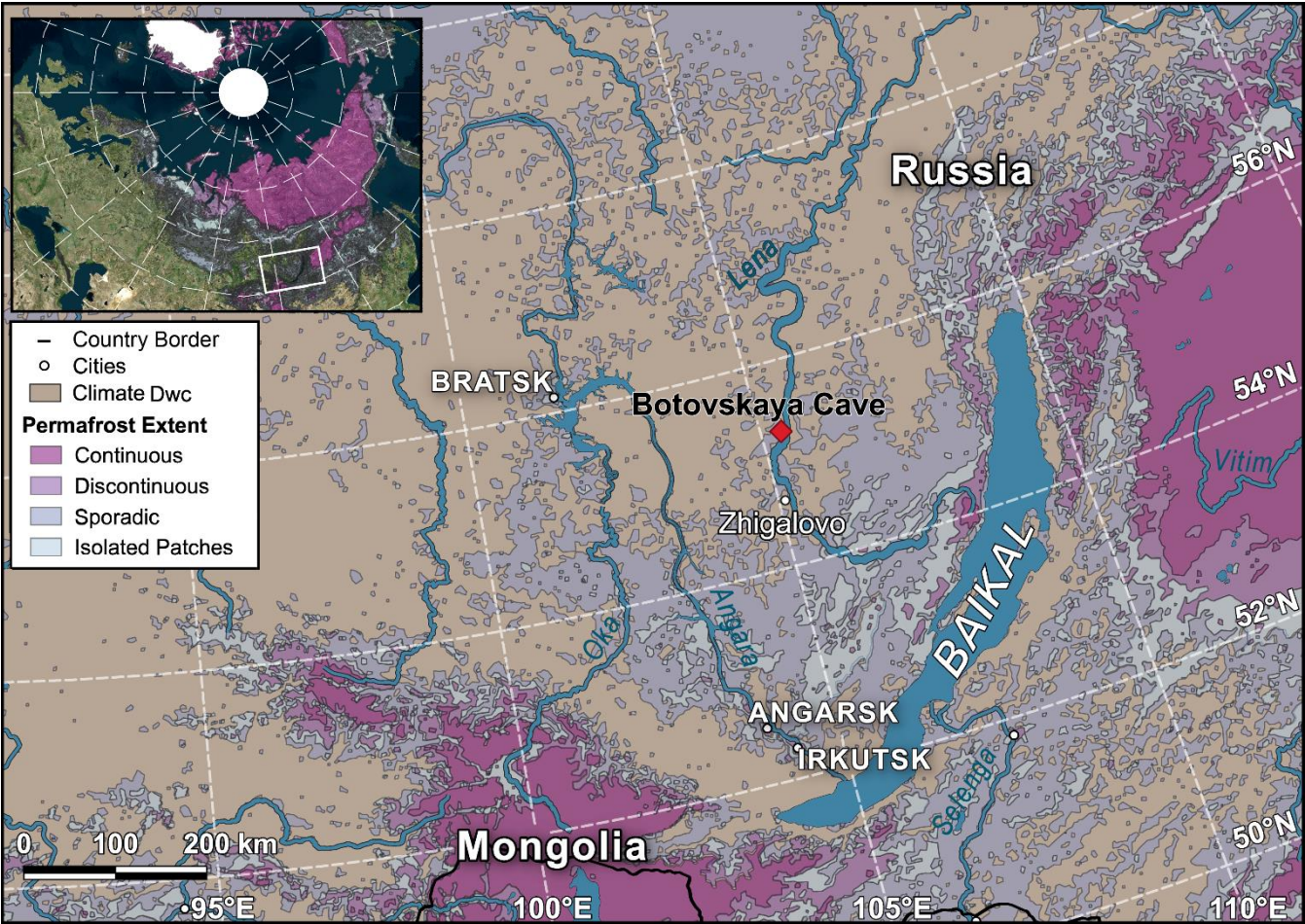
130 Figure 1: Location of Botovskaya cave in southern Siberia, Russia. Permafrost zones within our study area are derived from modelled permafrost probabilities (Obu et al., 2019). Botovskaya cave is within the zone of sporadic permafrost. Base aerial data: Microsoft Bing Maps.
