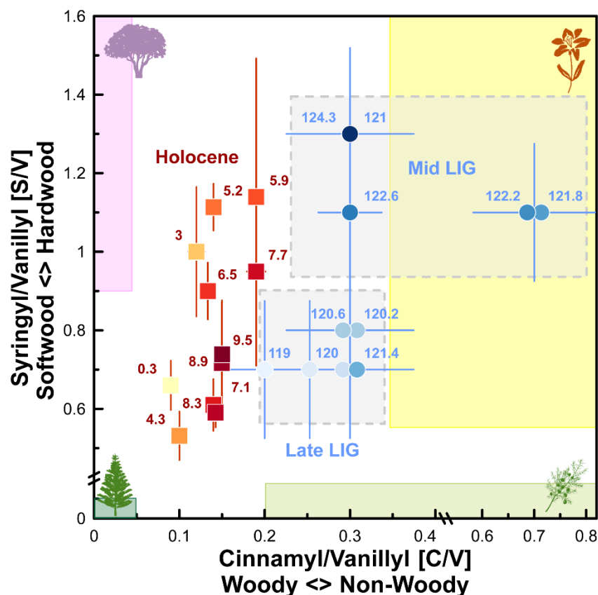
Figure 4: Stalagmite-based S/V vs. C/V ratios reflect changes in vegetation composition during the last interglacial (LIG) and the Holocene. Samples are color-coded by age, with darker colours indicative of older samples. Red points are Holocene samples and the blue LIG samples. Overlapping samples were adjusted left/right for clarity (e.g., 122.2 – 121.8 ka). The shaded boxes denote experimentally determined LOP ratios of predominant species (Hedges and Mann, 1979); dark green is dominated by softwood woody plants, light-green by softwood non-woody plants, pink denotes hardwood woody plants, and yellow indicates hardwood non-woody plants. Regions generally characterised by the mid-LIG and late LIG are highlighted by grey-shaded boxes. The Holocene is characterised by more woody vegetation compared to the LIG. Icons (pine tree, juniper bush, flower, and deciduous tree) are all sourced from www.freepick.com .
