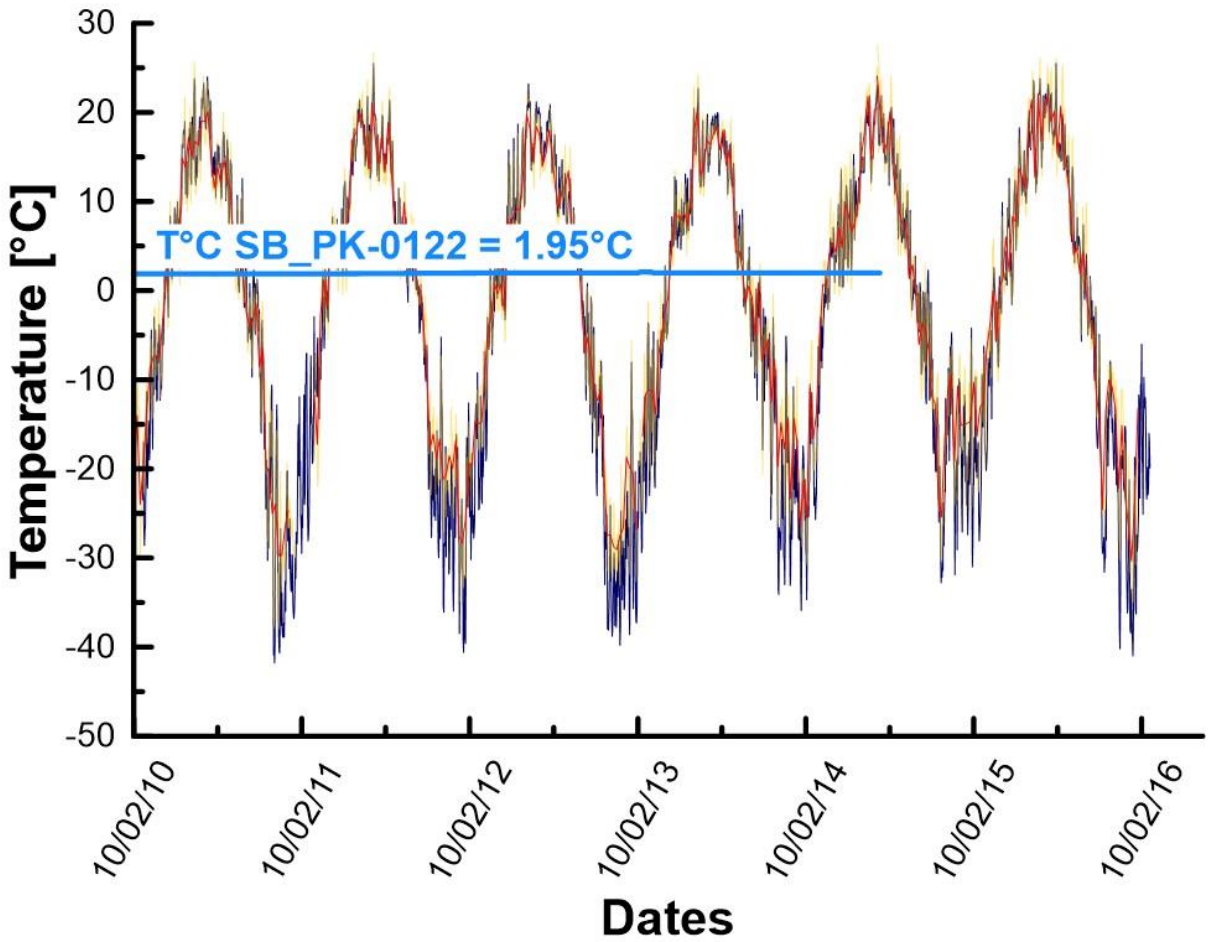
785 Fig. B: Temperatures recorded inside (light blue line) and outside (yellow and red lines) Botovskaya cave over a period of 6 years. Trends of both daily (yellow line) and weekly average (red line) temperatures outside the cave are increasing since 2013, whereas inside mean cave temperatures remain stable. Average daily temperatures for Zhigalovo meteorology station (55 km south of Botovskaya – see Fig. 1) are recorded by the navy-blue line (Klein Tank et al., 2002).
