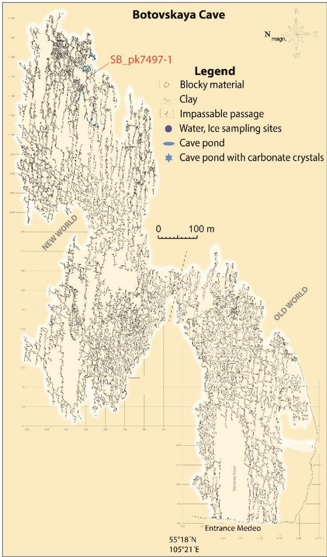
Fig. A: Mapped areas of Botovskaya cave with locations of specimen. Old and New world regions are joined in the area crossed with a grey dashed line. The location of sample SB_pk7497-1 is highlighted in the northeastern part of the New World. Key features are listed within the figure.
