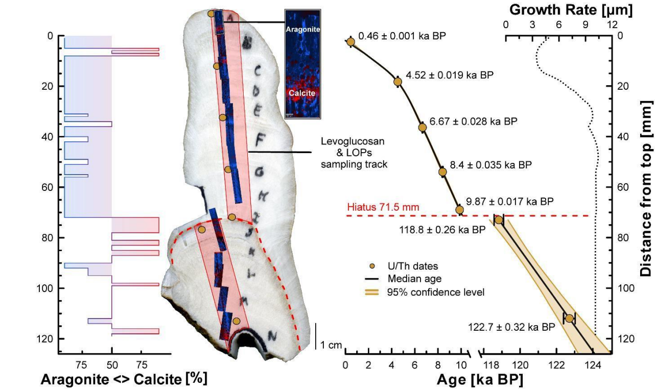
Figure 2: Distribution of U-Th dates and age uncertainties along stalagmite SB_pk7497-1. The COPRA median age model (black line) is constrained by 7 U-series dates (gold circles with 2s error bars). The hiatus is shown as dashed red line. The golden lines and shading highlight the 95% confidence bounds of the age-depth model. Growth rate varies from ca. 9.8 \mu\text{m/a} during the LIG and early Holocene to ca. 3.4 \mu\text{m/a} in the late Holocene (black dotted line). The red shaded area shows the sampling area for levoglucosan
