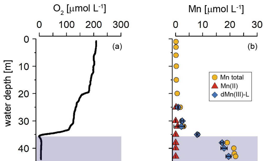
245 Figure 2. A) Water column O 2 and B) total dissolved Mn and dissolved Mn(II) and dMn(III)-L (error bars represent standard deviation; n=3) in the Scharendijke basin as observed in September 2020. The shaded area indicates the anoxic part of the water column.
