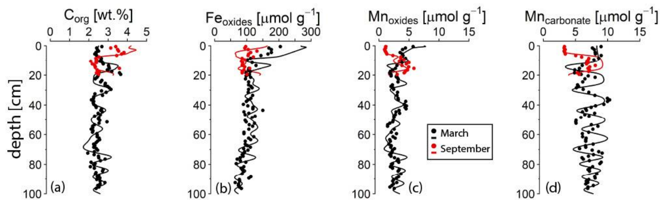
285 Figure 4. Solid phase profiles of key components in March (black) and September (red) 2020. The dots represent measured values, the lines indicate the results of the reactive transport model. Fe oxides refer to the sum of the Fe extracted in the ascorbic acid, CDB and ammonium oxalate extraction steps. Mn oxides refer to the Mn that is extracted in the ascorbic acid step. The profiles for all extraction steps are shown in Fig. S8 and S9.
