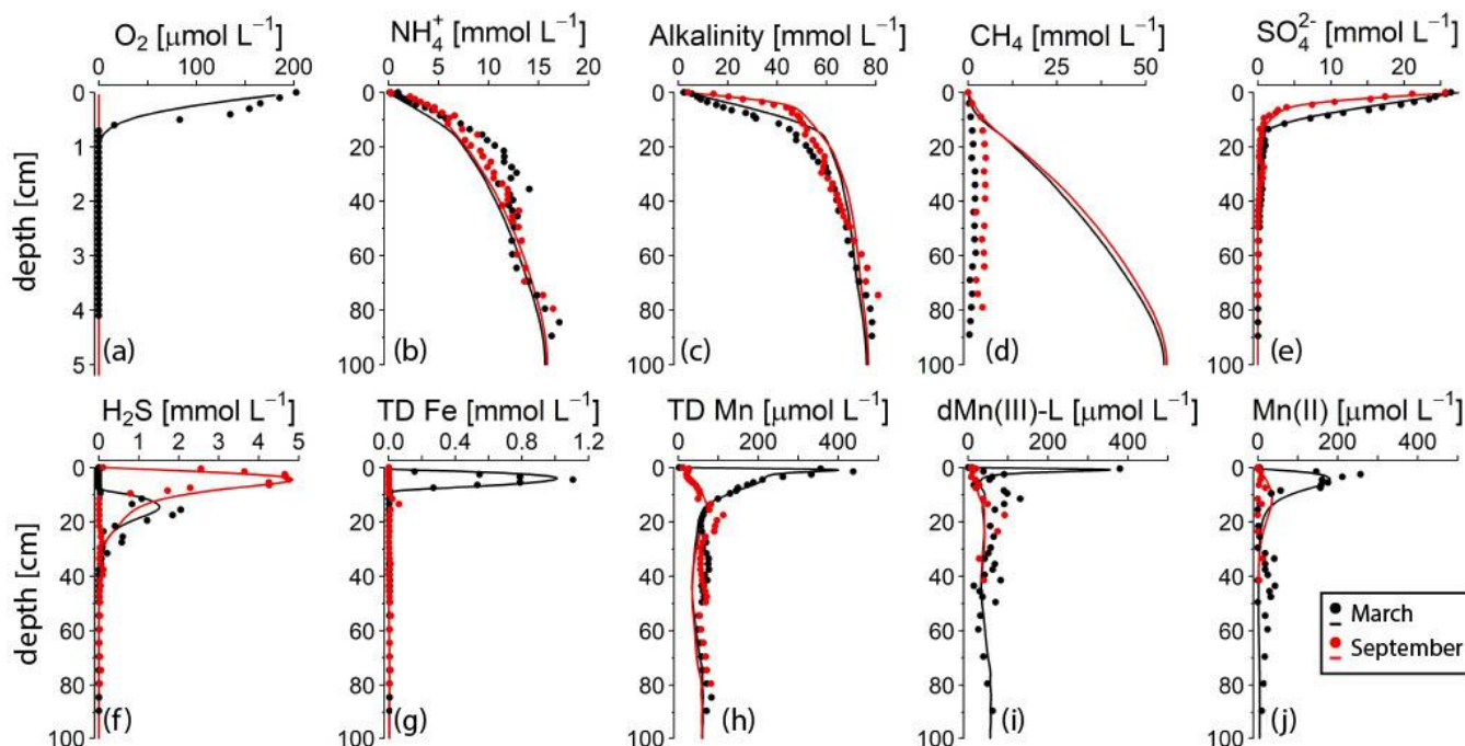
255 Figure 3. Pore water profiles of key components in March (black) and September (red) 2020. The dots represent measured concentrations, the lines indicate the results of the reactive transport model. Note the different depth scale on the y-axis for O 2 . TD Fe and TD Mn refer to total dissolved Fe and total dissolved Mn. Profiles of Mn(II) and dMn(III)-L with standard deviation error bars (n =3) and the contribution to TD Mn (in %) can be found in Fig. S5, S6. No O 2 was detected in the sediment in September 2020. A zoom of the top 20 cm of the profiles is presented in Fig. S7.
