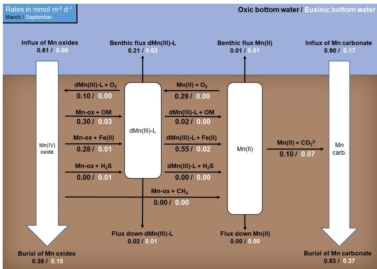
305 Figure 5. Rates of Mn cycling in March (black) and September (white) 2020 as calculated with the reactive transport model. Numbers represent depth integrated reaction rates in mmol m -2 d -1 . Note that the rates are not balanced because the system is not at steady state. The depth profiles of the reaction rates can be found in Fig. S10.
