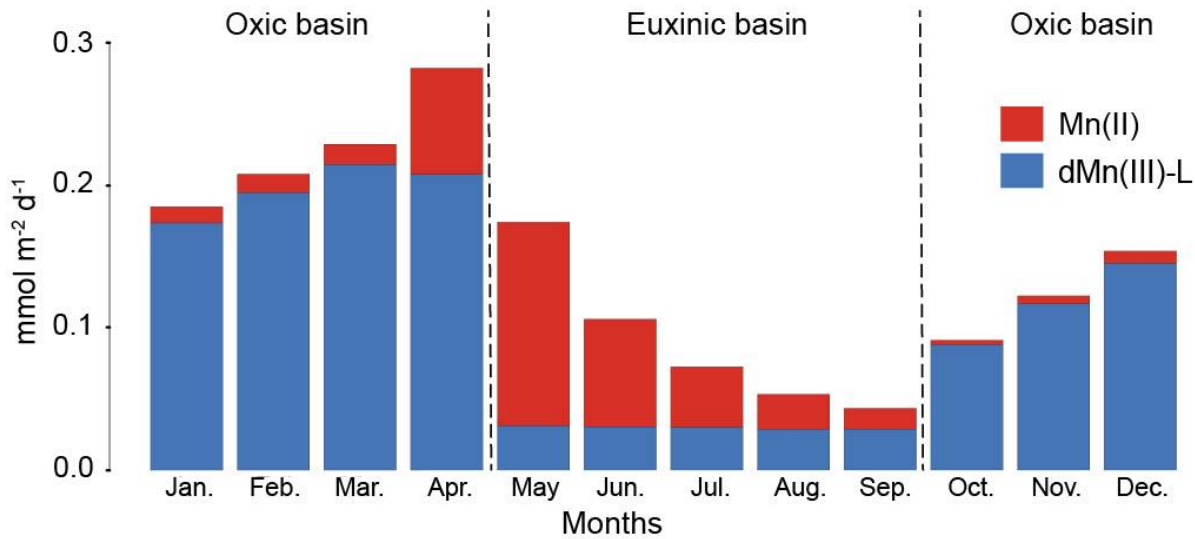
335 Figure 7. Sediment-water exchange of dissolved Mn (mmol m -2 d -1 ) calculated per month in 2020. The total dissolved Mn flux consists of dissolved Mn(II) and dMn(III)-L. Positive numbers indicate a flux from the sediment to the overlying water.
