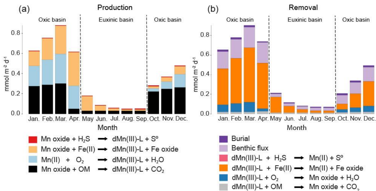
320 Figure 6. Depth integrated reaction rates for the sediment processes that (a) produce dMn(III)-L and (b) that remove dMn(III)-L as calculated with the model. The rates are calculated for each month of one year (2020) and are given in mmol m -2 d -1 .
