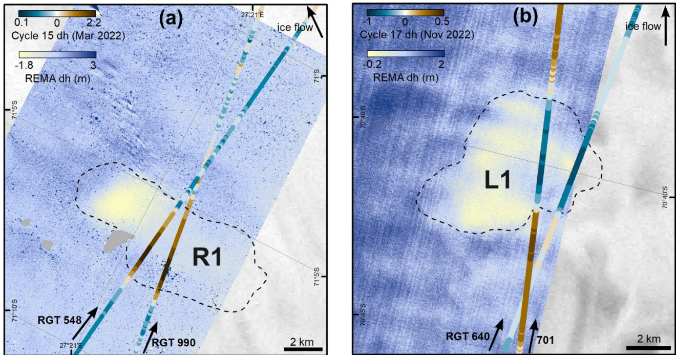
Supplementary Fig. 2: Ice surface elevation change from REMA strip differencing for Lakes R1 (a) and L1 (b). Regions of ice surface subsidence (yellow shading) between time-stamped REMA strip pairs (7 th December 2016 – 21 st December 2017 and 12 th September 2015 – 10 th December 2016) are delineated by the dashed lines. Each example highlights the spatial cooccurrence between localised ice surface subsidence and surface elevation anomalies along the intersecting ICESat-2 tracks, suggesting Lakes R1 and L1 were draining during the period bounded by the REMA strip pairs.
