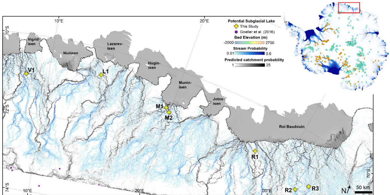
Supplementary Figure 6: Probability of subglacial drainage basin boundaries over the ensemble of 50 stochastic simulations derived from water routing analysis. The dashed black line is the MEASUREs grounding line (Rignot et al., 2016) and ice-shelf imagery is from the MODIS mosaic (Haran et al., 2021). Subglacial lake locations depicted in the inset map are from Livingstone et al. (2022), where active lakes are represented by orange dots and stable lakes by green dots.
