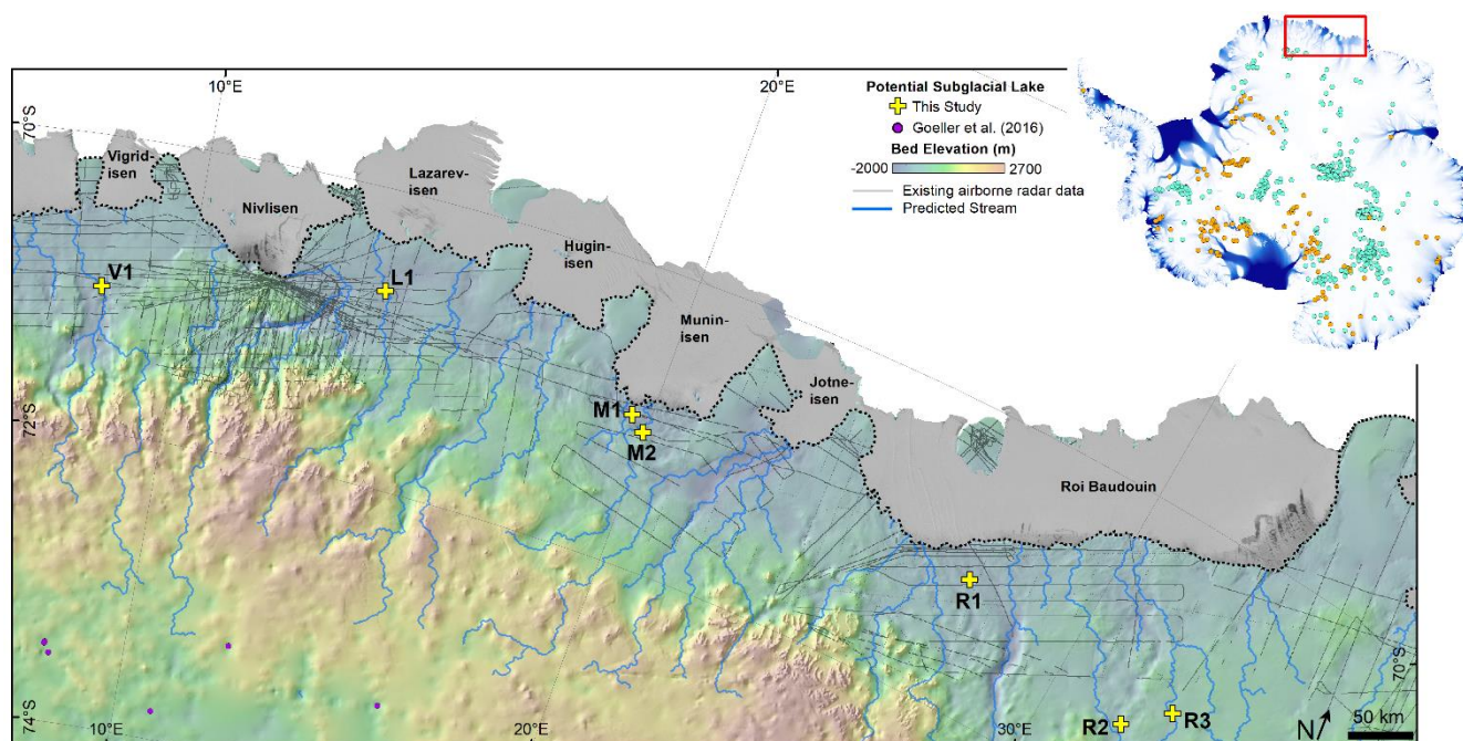
Supplementary Figure 5: Example of predicted streams from water routing analysis for one of 50 stochastic simulations. Newly-identified active lakes in this study are shown in yellow and previously-identified subglacial lakes from Goeller et al. (2016) are shown in purple. The dashed black line is the MEaSUREs grounding line (Rignot et al., 2016) and the bed elevations are from BedMachine (Morlighem et al., 2022). Ice-shelf imagery is from the MODIS mosaic (Haran et al., 2021). Subglacial lake locations depicted in the inset map are from Livingstone et al. (2022), where active lakes are represented by orange dots and stable lakes by green dots.
