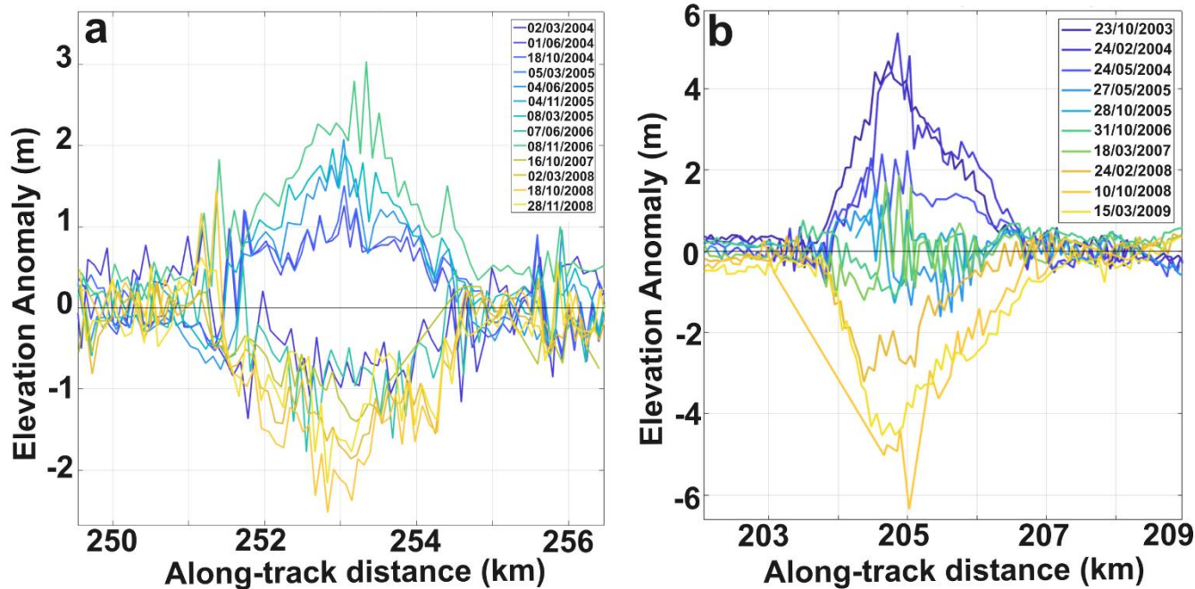
Supplementary Figure 4: Ice surface elevation displacement anomalies from two ICESat tracks over and Lake L1 (a, Track 134) and Lake R1 (b, Track 21). Elevation anomalies are calculated with respect to surface plane fits representing averaged surface elevation.
