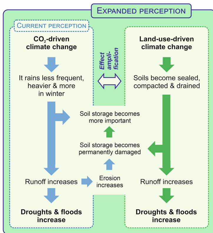
Figure 4: Current perception of the influence of CO 2 -driven climate change on rain and subsequent droughts and floods (left panel) and expanded perception, including land-use-driven climate change (right panel) and their interaction.
