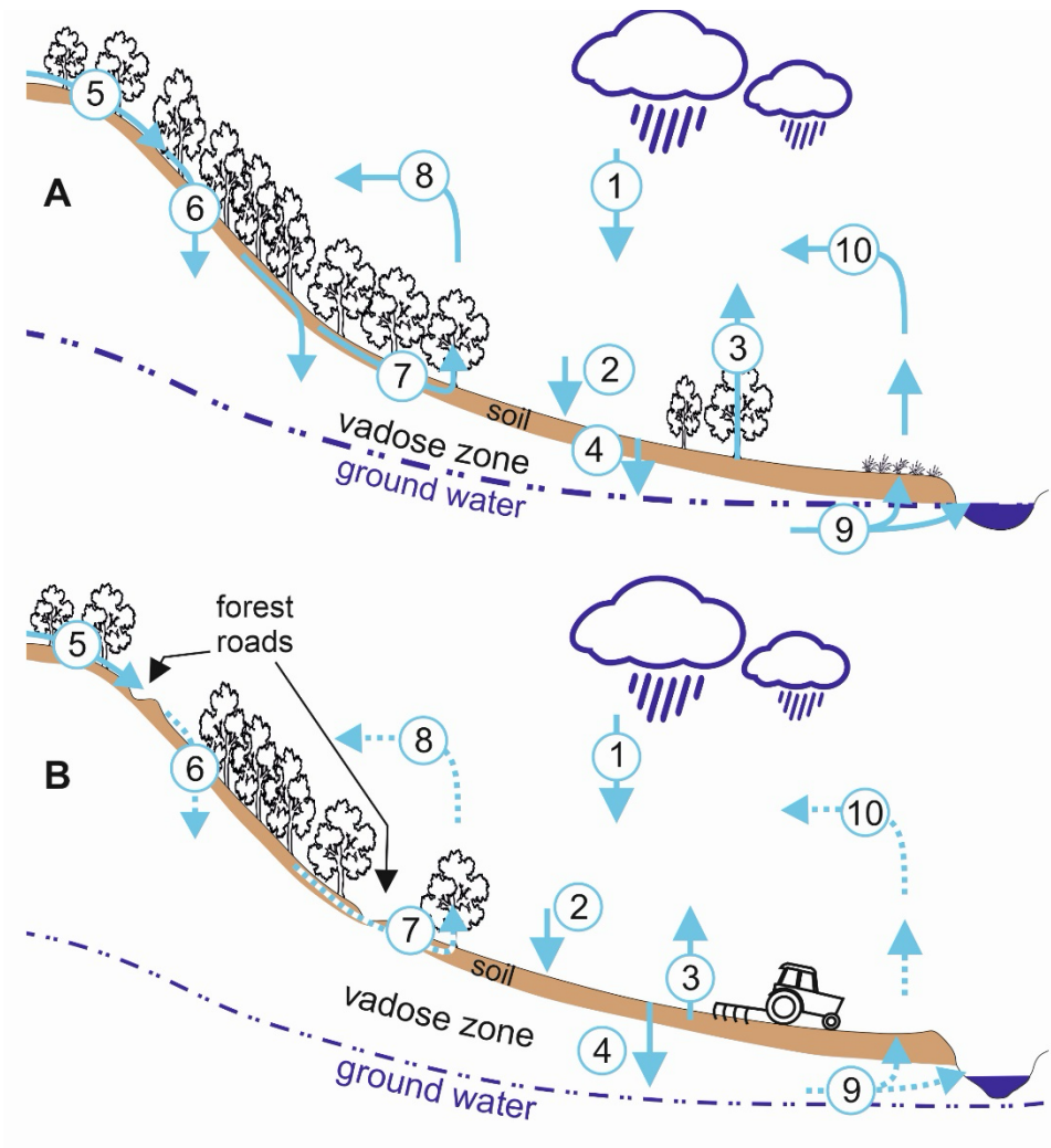
Figure 5: Schematic representation of (A) intact landscape hydrology and (B) under contemporary conditions where lateral water flows have been strongly disturbed (dashed lines) by infrastructure and other interventions and where the groundwater was lowered (1 precipitation, 2 infiltration, 3 evapotranspiration, 4 groundwater recharge, 5 surface runoff, 6 run-on infiltration, 7 interflow, 8 air-moisture transport, 9 groundwater flow, 10 groundwater-born evapotranspiration and air-moisture transport).
