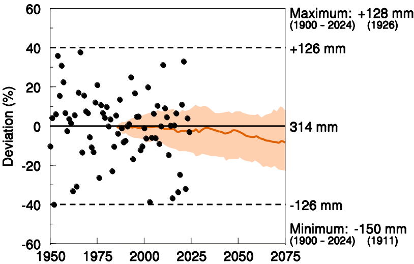
125 Figure 2: Deviations of summer rainfall (June, July, August) in Bavaria (approx. area 71,000 km 2 ) from the average 1971 to 2000 (being equal to the average 1900 to 2024); black circles and black curve show measurements, orange shaded area and orange curve show the bandwidth and the median of projections for RCP 8.5 (Data redrawn from BySMUV, 2021, and complemented with years 2020 to 2024 taken from DWD, 2025, which was also used by BySMUV, 2021).
