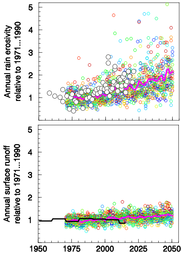
135 Figure 3: Change in annual rain erosivity (top panel) and surface runoff (bottom panel) relative to the mean from 1971 to 1990. Colored symbols (taken from Auerswald et al., 2019c) were calculated from an ensemble of ten projections approved by the German Weather Service following RCP 8.5. Each colour indicates one of the ten climate projections. See the Appendix for the climate projections, methods, and covered area. The magenta line is a 3-year moving average of 10 projections (thus equivalent to a 30-year normal period). The black symbols (top panel) show the measured erosivities taken from (Auerswald et al., 2019a and Winterrath, 2023). The black line (bottom panel) shows the 10-year means of a full hydrologic model based on measured meteorological data (taken from Baumeister et al., 2017; for other hydrologic parameters resulting from this model, see Fig. 1).
