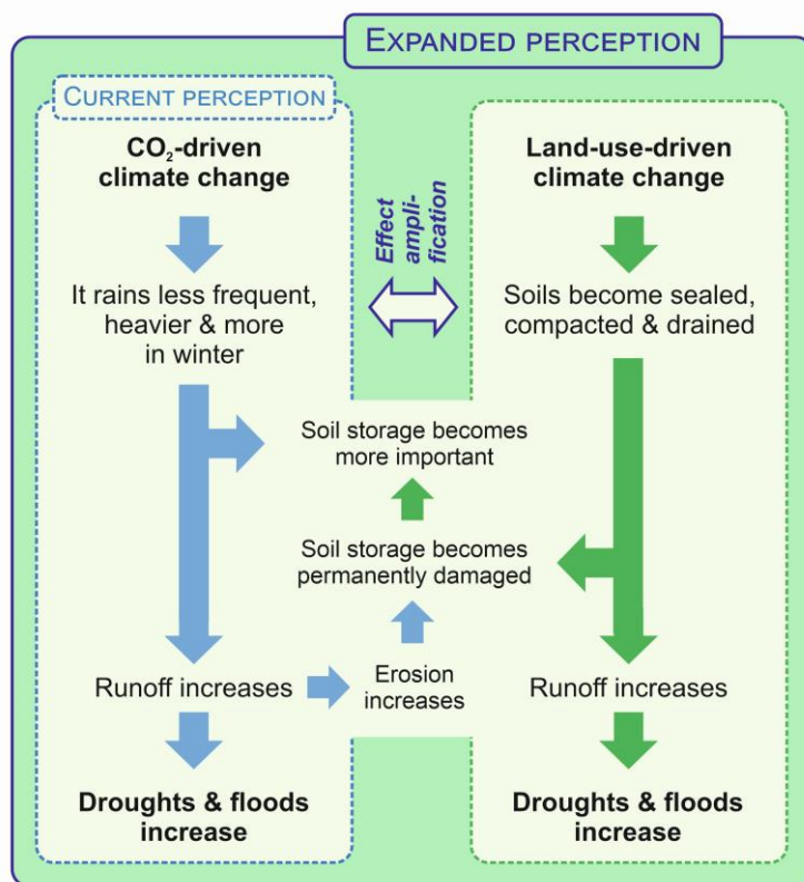
170 Figure 4: Current perception of the influence of CO 2 -driven climate change on rain and subsequent droughts and floods (left panel) and expanded perception, including land-use-driven climate change (right panel) and their interaction.
