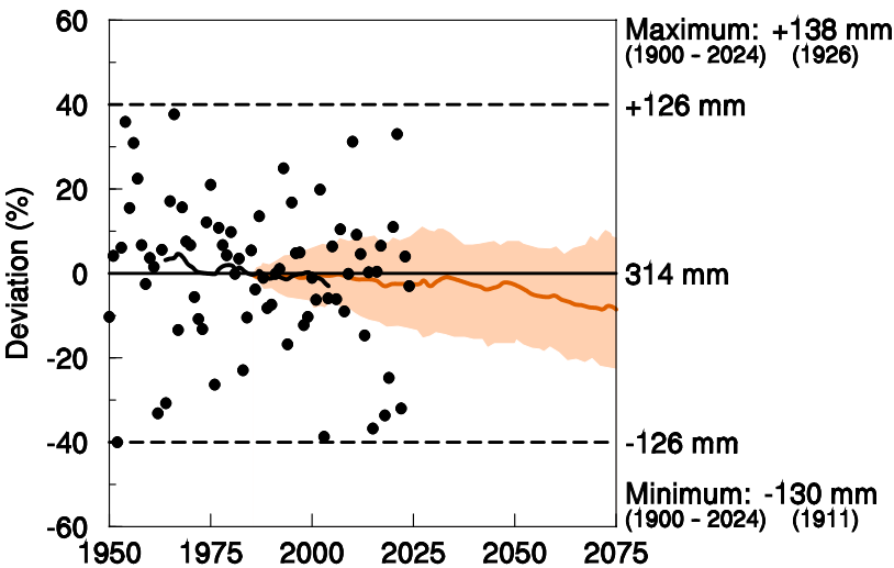
Figure 2: Deviations of summer rainfall (June, July, August) in Bavaria (approx. area 71,000 km 2 ) from the average 1971 to 2000 (being equal to the average 1900 to 2024); black circles and black curve show measurements, orange shaded area and orange curve show the bandwidth and the median of projections for RCP 8.5 (Data redrawn from BySMUV, 2021, and complemented with years 2020 to 2024).
