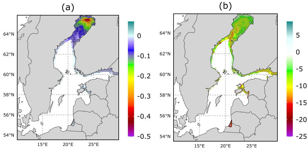
Figure 12. Linear trend for (a) ice thickness (in cm/year) (b) ice thickness (in %) for mean of Nov–May ice thickness from 1993/94 to 2020/21. Black dots mark the areas with 95 % significance level
