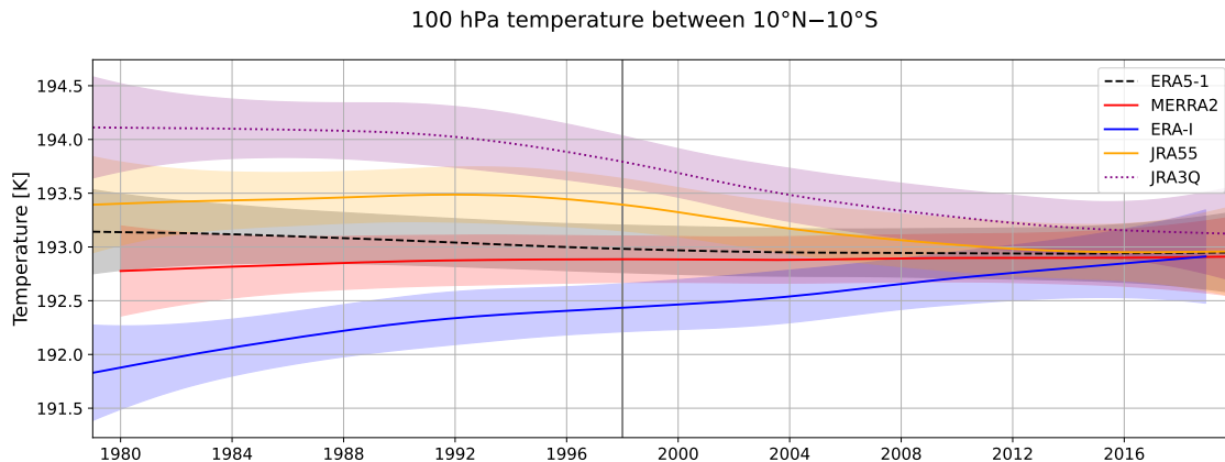
Figure 4. DLM trend state for the average tropical (10°N–10°S) temperature at 100 hPa in ERA5 (black, dashed line), MERRA-2 (red, solid), ERA-Interim (blue, solid), JRA-55 (orange, solid) and JRA3Q (purple, dotted) for the time period 1979–2019. Shading denotes the range of 2 standard deviations. The ERA-Interim time series ends in 2018, MERRA-2 begins in 1980.
