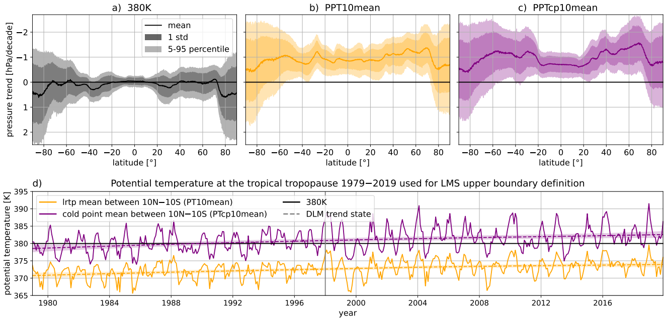
Figure 9. Zonal mean pressure trends of the LMS upper boundaries in ERA5 as estimated by the DLM for the time period 1998–2019 (upper panels) together with the potential temperature evolution at the tropical tropopause (lower panel). The potential temperature at the tropical ( 10^{\circ}\text{N} – 10^{\circ}\text{S} ) lapse rate tropopause (PT10mean, orange) and the cold point (PTcp10mean, purple) define the isentropes that serve as dynamical upper LMS boundaries (PPT10mean and PPTcp10mean). The upper LMS boundary can also be approximated with the 380 K isentrope, which is presented in addition (black). In the upper panels, the pressure trends of the respective boundaries are presented, showing the the mean trend (solid line) together with the associated standard deviation (dark shading) and the 5–95 percentile (light shading). Note that the pressure trend axis is inverted because decreasing pressure is associated with an upward trend in the pressure coordinate system. The lower panel shows the potential temperature time series (solid line) between 1979–2019 together with the DLM trend state time series (dashed lines) and the range of two standard deviations (shading). The grey vertical line marks the beginning of the year 1998.
