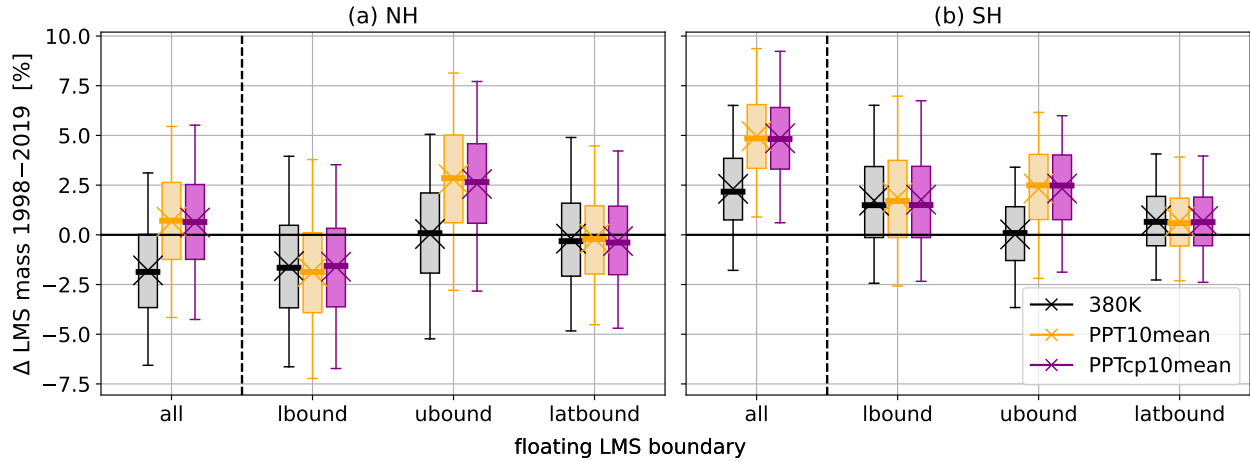
Figure 13. Similar to Fig. 12 but for hemispheric LMS mass difference if only one LMS boundary is allowed to evolve in time ("floating") while the other two are fixed, i.e. the year 1979 repeated. The respective boundaries are the lower boundary (lbound, here: the lapse rate tropopause), the upper boundary (ubound, either 380 K (black), PPT10mean (orange) or PPTcp10mean (purple)) and the lateral boundary (latbound). For comparison, the LMS mass change between 1998–2019 for all boundary surfaces evolving in time is presented to the left of the dashed vertical line (same as in Fig. 12a and c).
