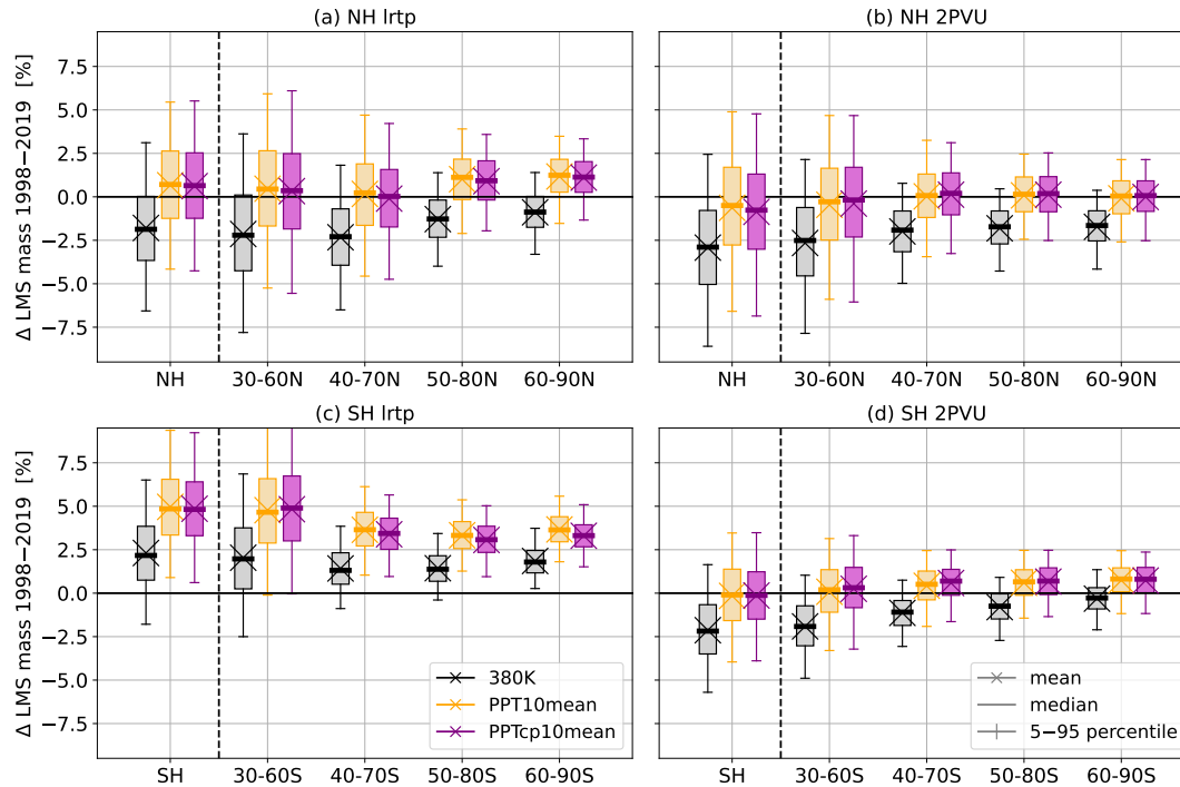
ERA5 LMS mass difference 1998–2019 according to DLM results
