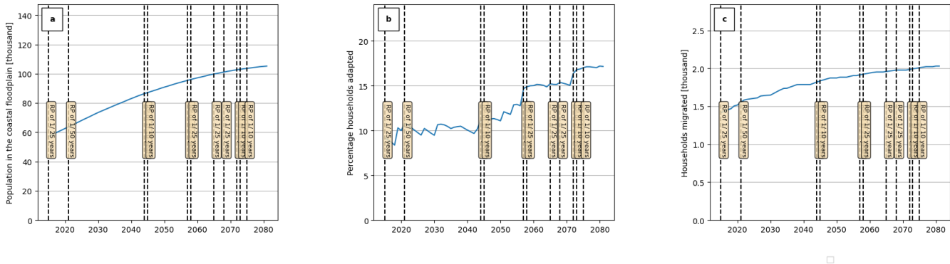
Figure 7 a: Population exposed to the risk of flooding and salt intrusion in the floodplain, b: percentage of households adapted, c: households migrated. This simulation is made for the coastal province of Sofala under RCP4.5-SSP2 and full behaviour setting.
