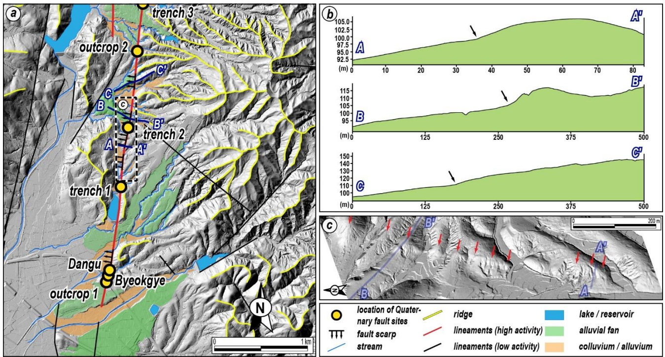
660 Figure A2: (a) A detailed topographic map of the southern region. (b) Topographic profiles along the main lineament (blue line in (a)) crossing the fault scarps. Black arrows mark knickpoints identified as fault scarps. (c) A 3D hillshade image. The red arrows highlight the fault scarp, which is clearly visible to the unaided eye (modified from Ha et al., 2022).
