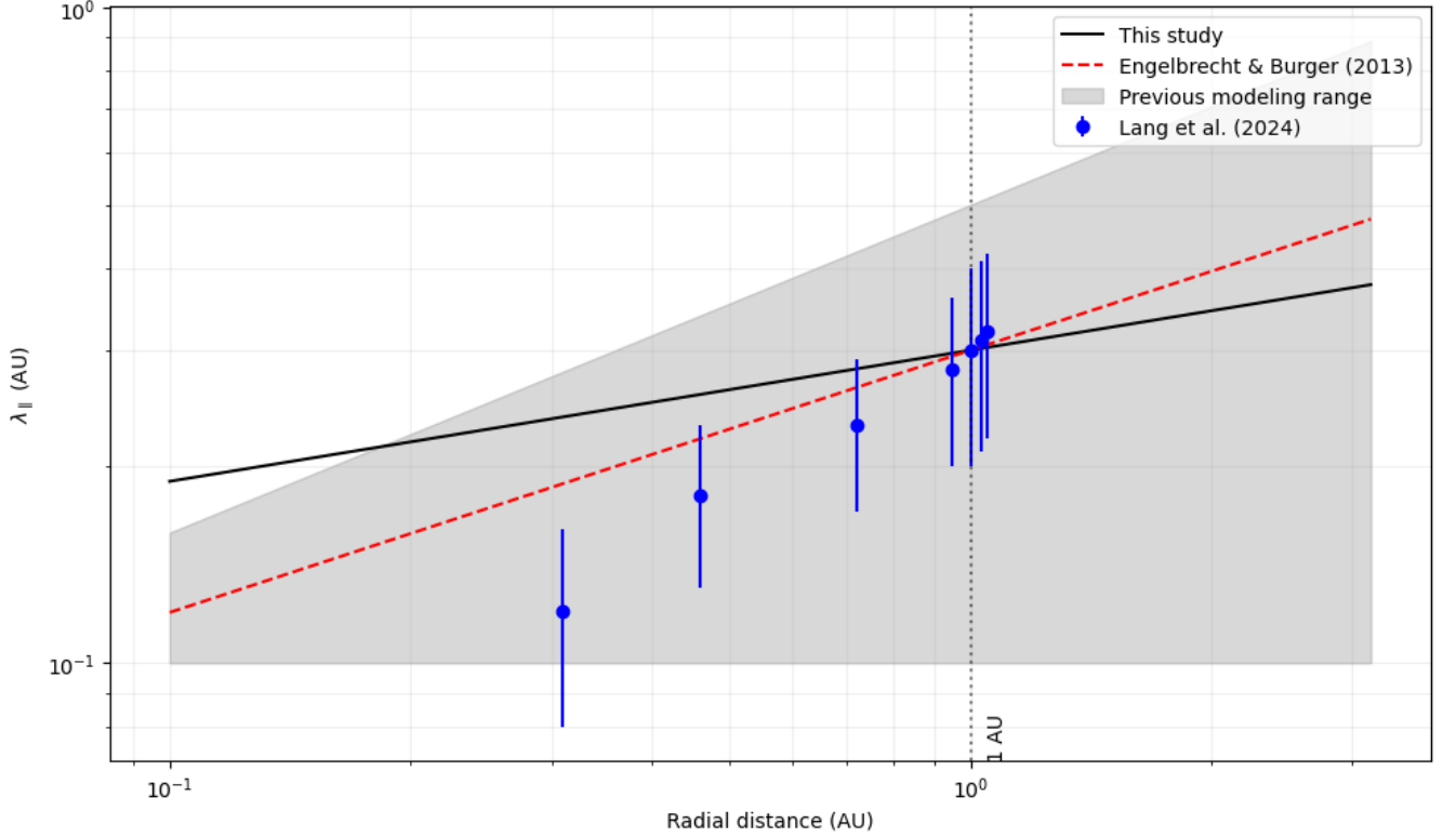
Figure 10. Radial dependence of the parallel mean free path ( \lambda_{||} ) for GeV protons. The solid black line represents our model ( \lambda_{||} = 0.3(r/1 \text{ AU})^{0.2} \text{ AU} ). The red dashed line shows the theoretical prediction from Engelbrecht and Burger (2013). Blue dots with error bars represent observational data from Lang et al. (2024). The shaded gray area indicates the range of \lambda_{||} values used in previous modeling efforts based on (Dröge et al., 2010; He et al., 2011). The vertical dotted line marks 1 AU for reference.
