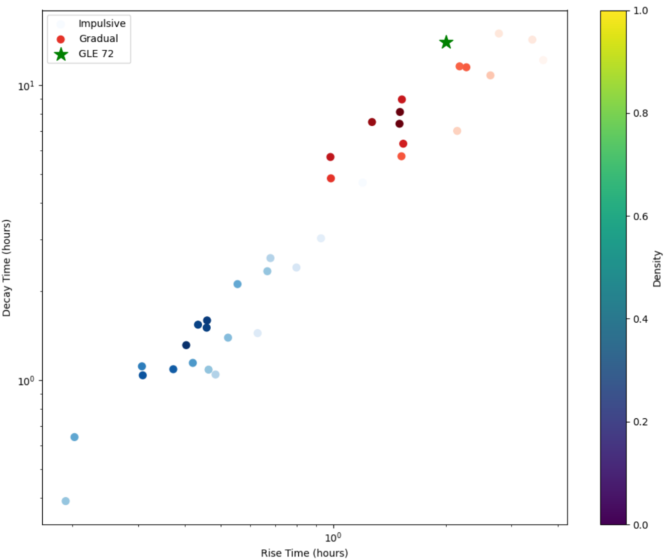
Figure 1. Distribution of Rise and Decay Times for GLEs.
