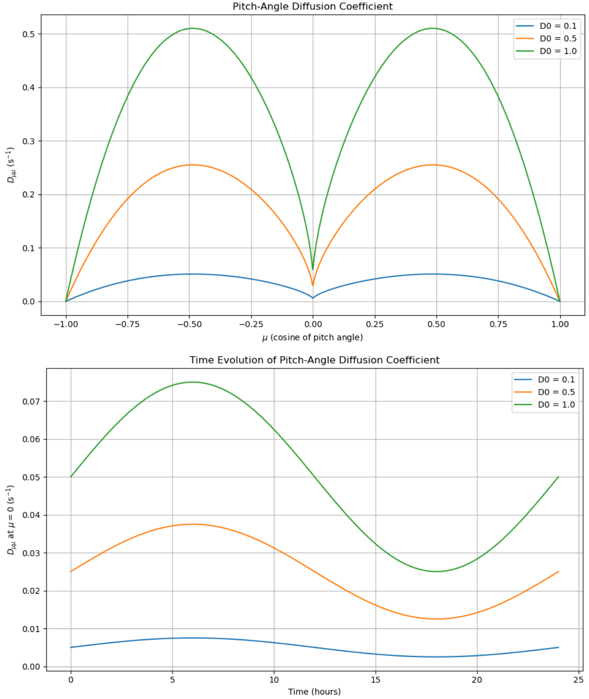
Figure 8. Pitch-angle diffusion coefficient ( D_{\mu\mu} ) characteristics. (Top panel) D_{\mu\mu} as a function of \mu (cosine of pitch angle) for different D_0 values. (Bottom panel) Time evolution of D_{\mu\mu} at \mu = 0 over 24 hours, simulating passage through a stream interaction region. The model uses D_{\mu\mu}(\mu, t) = D_0(t)(1 - \mu^2)(|\mu|^{5/3-1} + 0.05) , where D_0(t) = D_0(1 + 0.5\sin(2\pi t/24)) represents time-dependent scattering conditions.
