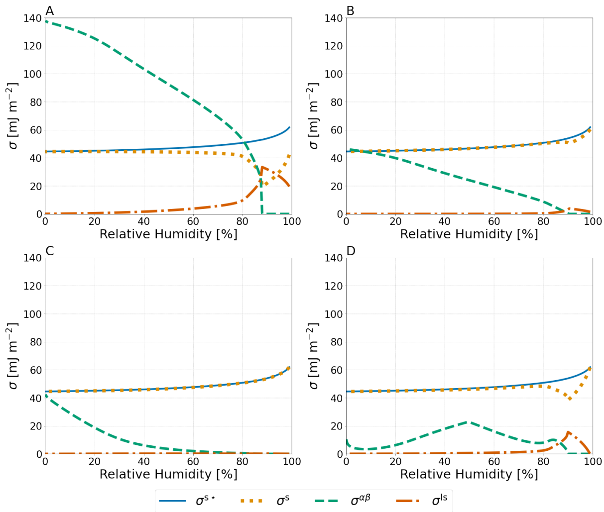
Figure 3. Predicted values of \sigma^{S^*} , which represent the measurable effect of expanding a finite depth surface phase as defined in Eq. (23); \sigma^S ; \sigma^{\alpha\beta} ; and \sigma^{ls} (see legend) for a particle of 1000 nm dry diameter composed of water-PEG-400-ammonium-sulfate at T = 298 K. \sigma^{\alpha\beta} and \sigma^{ls} were calculated using (A) Antonov's rule (Eq. 1), (B) the Girifalco-Good equation (Eq. 2), (C) the Butler equation with geometric mean activity coefficients (Eq. 14), and (D) the weighted mean interfacial composition approach (Eq. 18).
