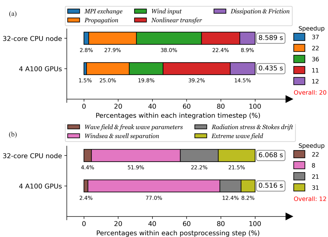
Figure 6. GPU runtime analysis within the integration (a) and postprocessing (b) time steps for a global 0.1^{circ} wave hindcast case.
