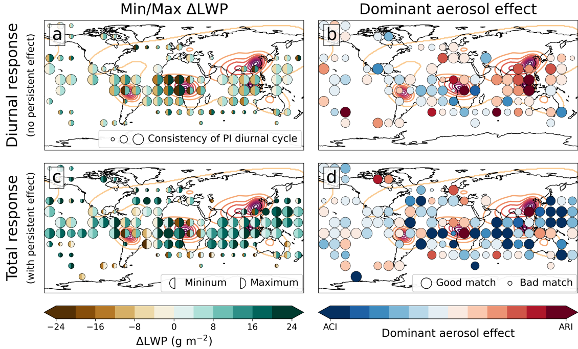
Figure 6. Contributions to \Delta LWP from the short-term diurnal component (a and b) and with the addition of the long-term persistent component (c and d). Panels (a) and (c) show the minimum (left hemisphere) and maximum (right hemisphere) absolute response during the diurnal cycle with larger circles representing an increasingly consistent LWP diurnal cycle throughout the PI simulation. Panels (b) and (d) show the dominating process (ARI/ACI) driving \Delta LWP, with larger circles representing a better match between the PD_{ARI} or PD_{ACI} and PD .
