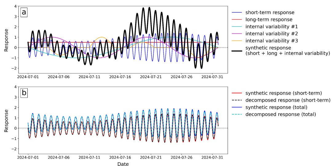
Figure R2. Figure demonstrating the capability of the decomposition method. A synthetic response in (a) includes a short-term diurnal component with a time-dependent amplitude, a long-term persistent time-independent component, and internal variability from multiple sources. The aim of the decomposition method is to sufficiently isolate any underlying short-term response along with a persistent response. The result of the decomposition method from the manuscript applied to the synthetic response (short-term + long-term + internal variability [1-3]) is shown in (b).
