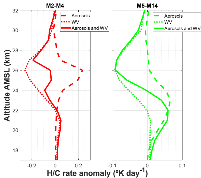
410 Figure 7: Mean profiles of aerosols only, water vapor only, and aerosol and water vapor daily heating/cooling rate anomaly averaged over the short-term period (M2 – M4) and the mid-term period (M5 – M14), all excluding week 1 and 2 after the eruption.
