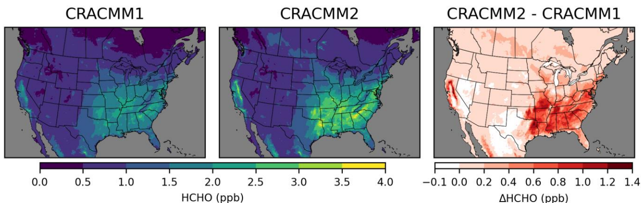
Figure 2. Surface layer 11 am–3 pm local time June–August 2019 average HCHO concentrations simulated with CRACMM1 (left) and CRACMM2 (middle) and the change in CRACMM2 compared to CRACMM1 (right). Analogous results for other seasons are provided in Fig. S9.
