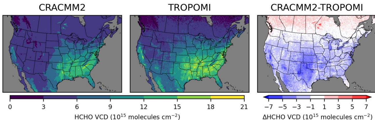
Figure 4. June–August 2019 average tropospheric vertical column densities from CMAQ with CRACMM2 (left) and from TROPOMI (middle) and the difference between CRACMM2 and TROPOMI (right). Similar comparisons for other seasons are provided in Fig. S11.
