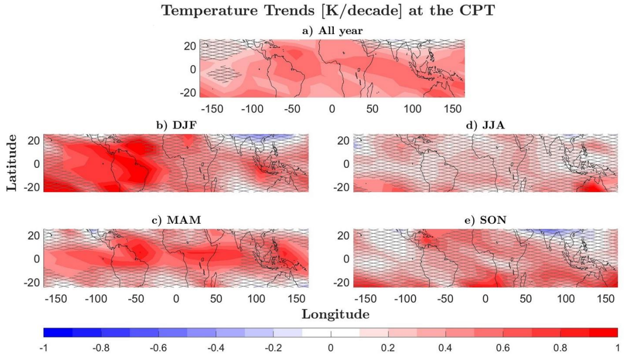
205 Figure 2. Long-term (2002-2022) temperature trends [K/decade] of the cold point tropopause (CPT) temperature based on the GNSS-RO dataset for the monthly mean (a) and seasonal mean time series (b-e). Trends not significant at the 95% confidence level are marked with grey crosses.
