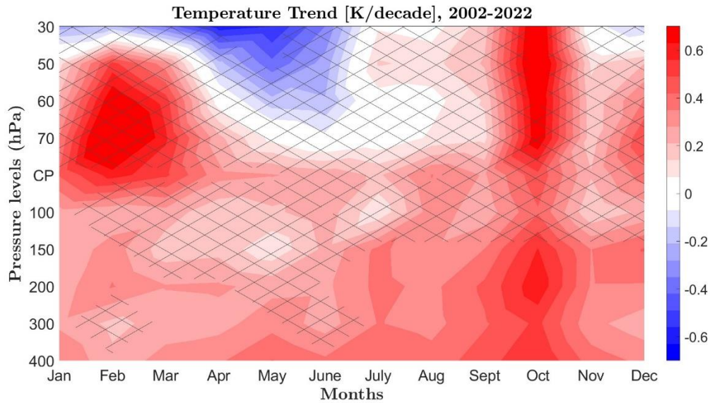
Figure 4. The seasonal cycle of temperature trends [K/decade] for 2002-2022 at the cold point (CP) and different pressure levels based on GNSS-RO data (20°S-20°N). Trends not significant at the 95% confidence level are marked with crosses.
