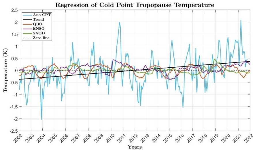
Figure 1. Tropical mean (20°S-20°N) deseasonalized cold point tropopause (CPT) temperature anomalies (Ano CPT), regression terms (QBO, ENSO, SAOD), and linear trend based on GNSS-RO data.
