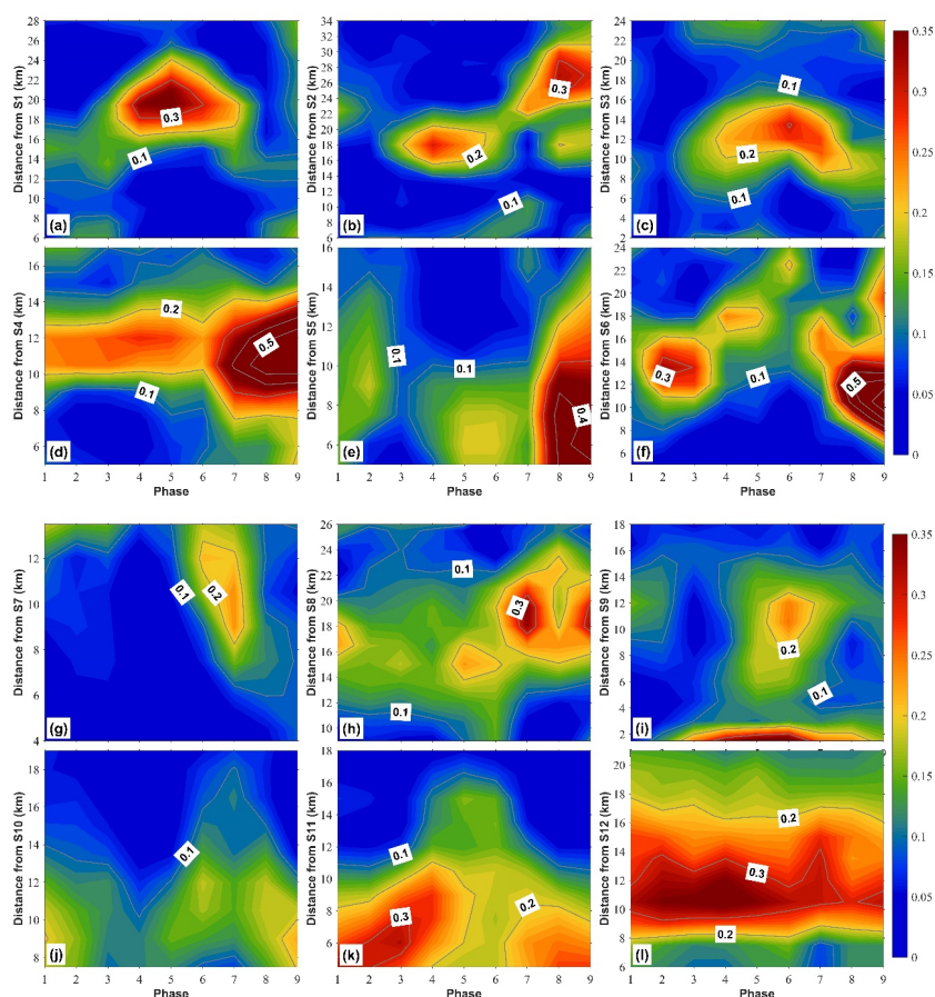
Figure 9. Intra-tidal variations of the gradient magnitude ( T_C ) of the SST along the pink lines across each front in Figures 7 and 8. S1-S12 in the y-axis labels means the start point of each pink line (black dot in Figures 7 and 8).
