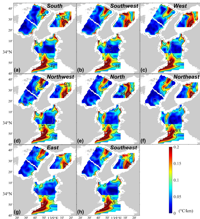
Figure 12. Average SST (contours) corresponding to the wind data in the same direction over the fronts F6-F10, F12 areas 350 in the eastern part of the SIS and its gradient magnitude ( T_G ) (colors) for eight directions of the wind. The thick black line indicates a gradient magnitude ( T_G ) contour of 0.1 \text{ } ^\circ\text{C}/\text{km} .
