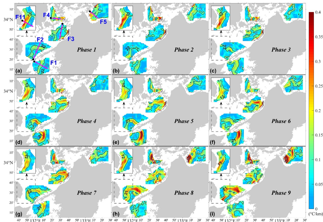
Figure 7. Averaged SST (contours) over the front F1-F5, F11 areas in the western part of the SIS and its gradient magnitude ( T_G ) (colors) for the nine tide phases (numbers 1-9 in Figure S1). The pink line perpendicular to each front is used to quantify the variations of the front along it. The black dot indicates the start point of each pink line. The thick black line indicates a gradient magnitude ( T_G ) contour of 0.1 ^{\circ}\text{C}/\text{km} . The dashed box indicates the original location of the front F11 area.
