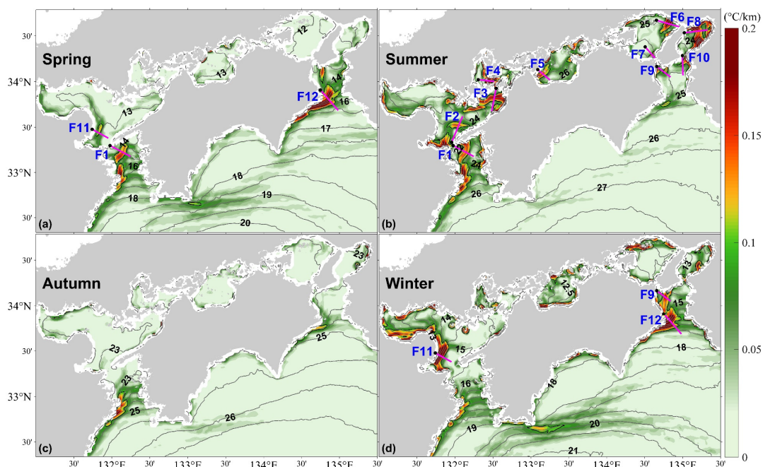
180 Figure 2. Seasonal mean SST (contours) and its gradient magnitude ( T_G ) (colors) from spring to winter. The thick black line indicates a gradient magnitude ( T_G ) contour of 0.1 °C/km.
