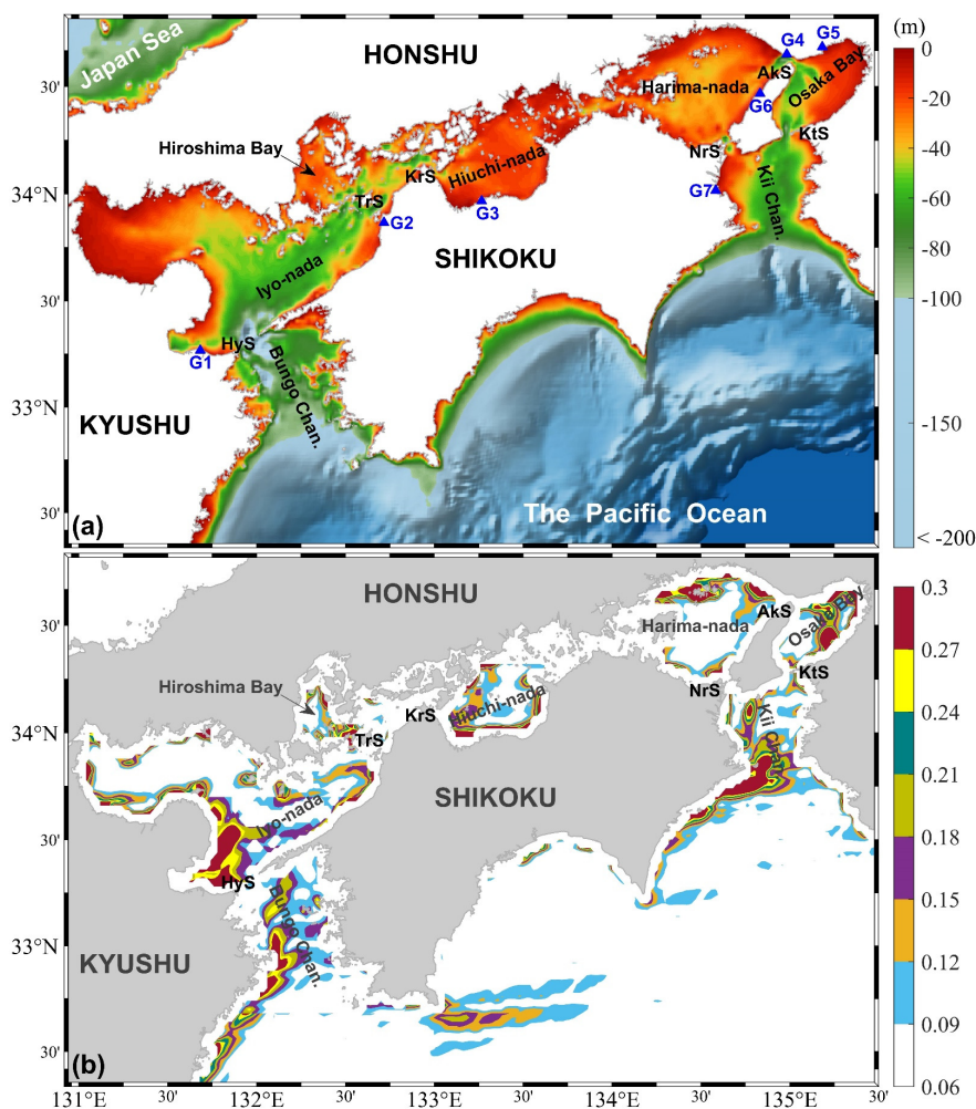
45 Figure 1. (a) Location and bathymetry of the SIS. The blue triangles indicate the gauge stations. ‘HyS,’ ‘TrS,’ ‘KrS,’ ‘AkS,’ ‘NrS,’ and ‘KtS’ denote Hayasui Strait, Tsurushima Strait, Kurushima Strait, Akashi Strait, Naruto Strait, and Kantan Strait, respectively. (b) The appearance frequency of the fronts in the SIS.
