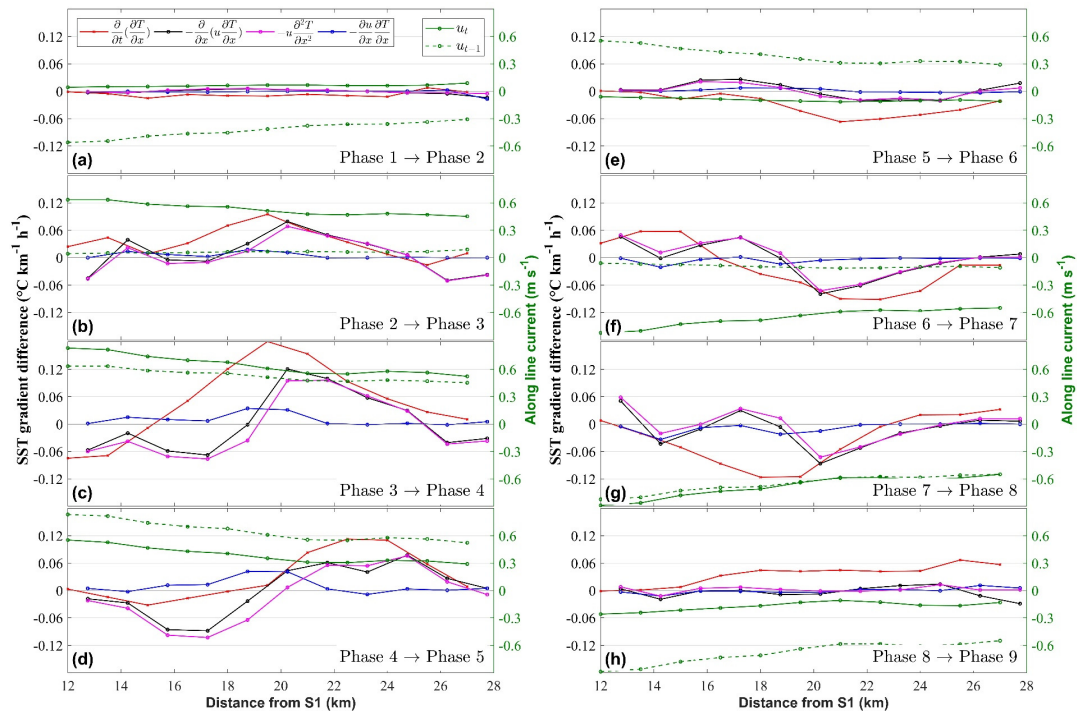
Figure 15. The left axis corresponds to the difference in front intensity between the two phases (red line), the transition term in Equation 5 ( -\frac{\partial}{\partial x} \left( u \frac{\partial T}{\partial x} \right) , black line), advection of an existing gradient ( -u \frac{\partial^2 T}{\partial x^2} , pink line), and intensification or weakening of the local gradient due to the convergence or divergence of the current ( \frac{\partial u}{\partial x} \frac{\partial T}{\partial x} , blue line) along the thick black line in Figure 13. The right axis corresponds to the tidal current along the thick black line in Figure 13 at the current phase (green solid line) and the previous phase (green dashed line).
