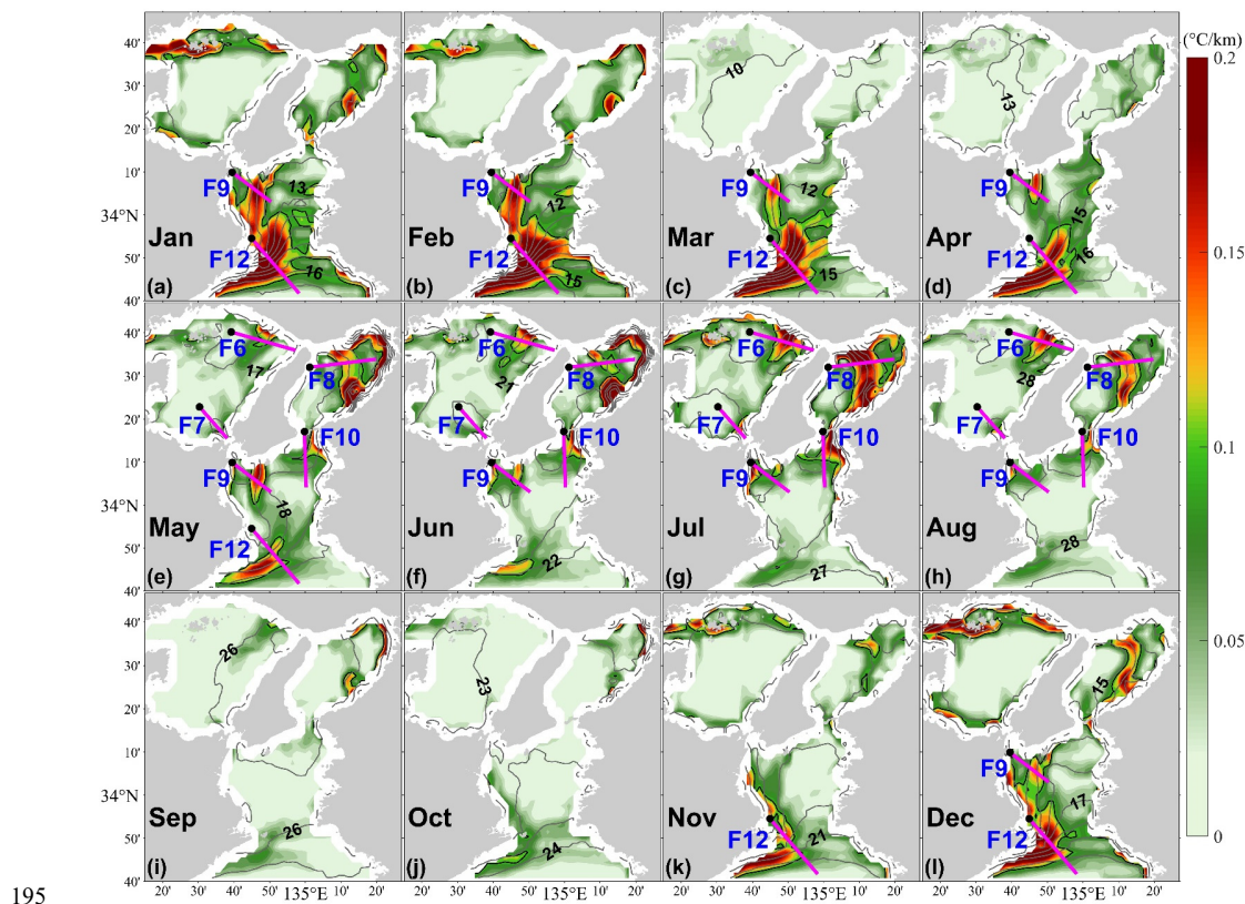
Figure 4. Monthly mean SST (contours) and its gradient magnitude ( T_G ) (colors) from January to December in the eastern part of the SIS. The pink line perpendicular to each front is used to quantify the variations of the front along it. The black dot indicates the start point of each pink line. The thick black line indicates a gradient magnitude ( T_G ) contour of 0.1\text{ }^{\circ}\text{C}/\text{km} .
