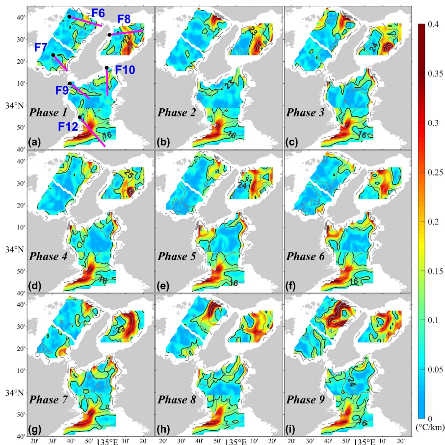
Figure 8. Averaged SST (contours) over the front F6-F10, F12 areas in the eastern part of the SIS and its gradient magnitude ( T_G ) (colors) for the nine tide phases (numbers 1-9 in Figure S1). The pink line perpendicular to each front is used to quantify the variations of the front along it. The black dot indicates the start point of each pink line. The thick black line indicates a gradient magnitude ( T_G ) contour of 0.1 °C/km.
