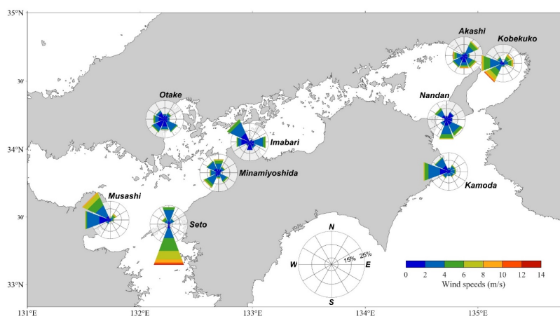
Figure 10. A succinct view of how the speed and direction of the wind data from 2016 to 2022 are typically distributed at nine observation stations. The wind data at Seto , Minamiyoshida , Otake , Imabari , Akashi , Kobekuko , and Nandan are for the summer, while the wind data at Musashi and Kamoda are for the winter. The frequency of winds is plotted by wind direction using a polar coordinate of gridding, and color bands show the wind speed ranges. The distribution of the wind is divided into eight directions.
