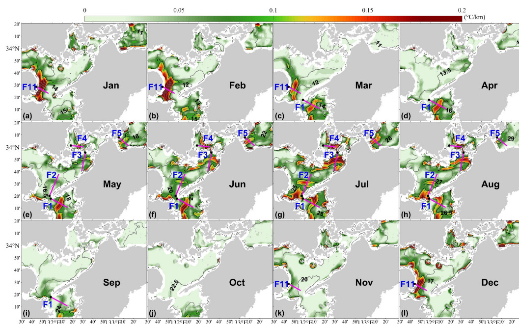
Figure 3. Monthly mean SST (contours) and its gradient magnitude ( T_G ) from January to December in the western part of the SIS. The pink line perpendicular to each front is used to quantify the variations of the front along it. The black dot indicates the start point of each pink line. The thick black line indicates a gradient magnitude ( T_G ) contour of 0.1 °C/km.
