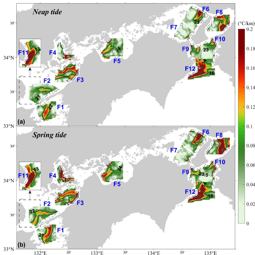
220 Figure 6. Average SST (contours) and its gradient magnitude ( T_G ) (colors) in the SIS during (a) neap tide and (b) spring tide. The thick black line indicates a gradient magnitude ( T_G ) contour of 0.1 °C/km. The dashed box indicates the original location of the front F11 area.
