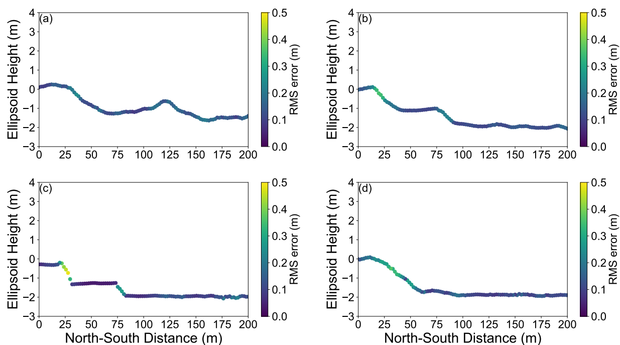
Figure A5. RMS error between our SlideRule-derived elevations and the source ATL03 photon information for ground track 2r for (a) 7 April 2019; (b) 4 January 2020; (c) 2 July 2021; (d) 31 December 2021
