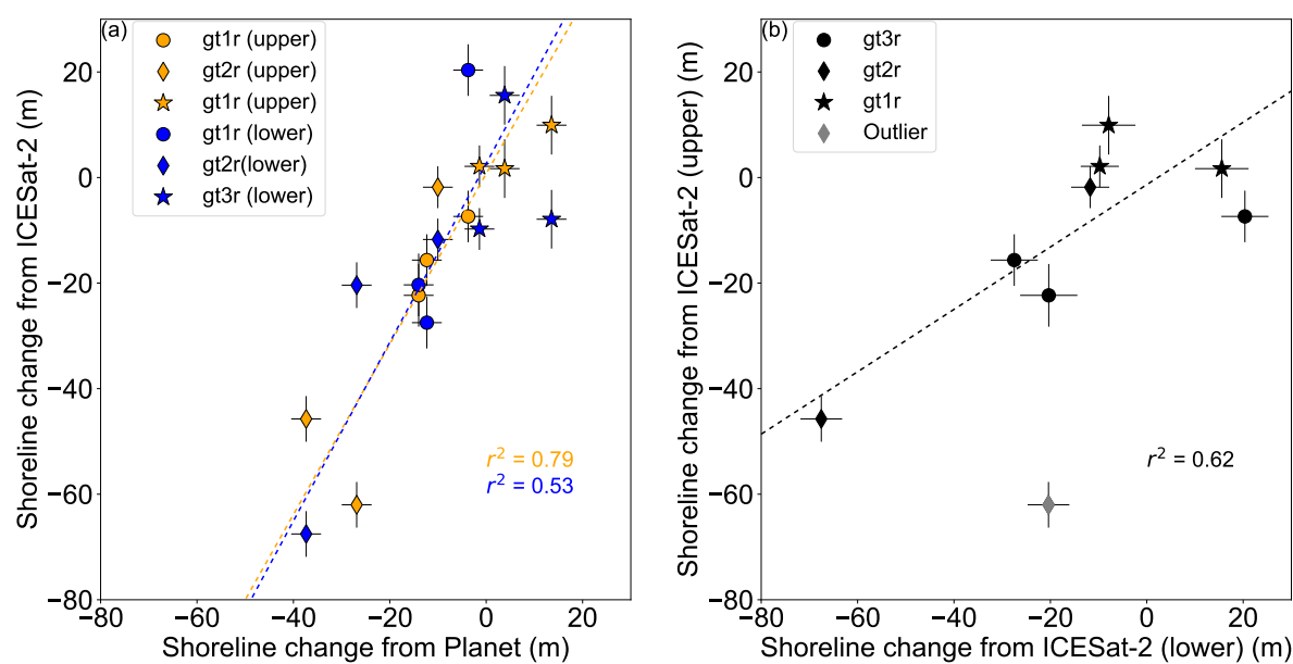
Figure 5. a) Comparison between shoreline change estimates from Planet and shoreline change estimates from the upper (orange) and lower (blue) boundaries derived from ICESat-2. b) Comparison between the measured change between each open water season across the upper and lower boundaries derived from ICESat-2. The coefficient of determination excluding the outlier drained lake measurement (grey) is reported. Linear fits were estimated using orthogonal distance regression.
