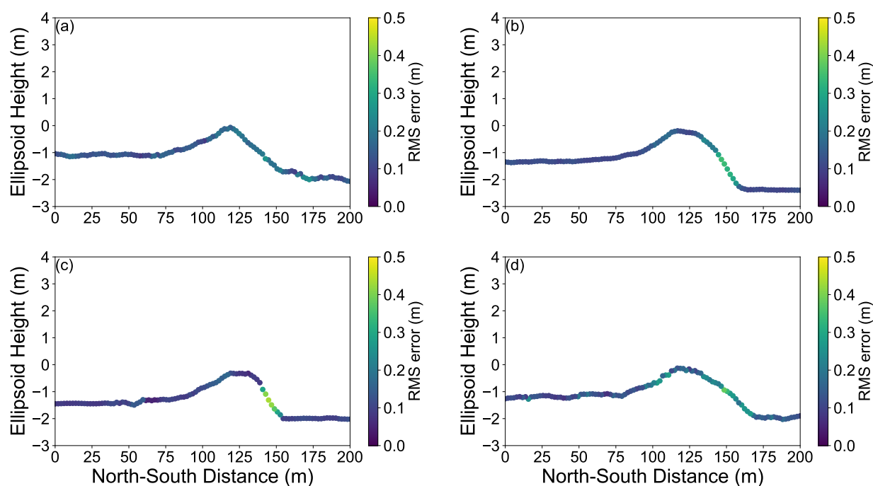
Figure A6. RMS error between our SlideRule-derived elevations and the source ATL03 photon information for ground track 1r for (a) 7 April 2019; (b) 4 January 2020; (c) 2 July 2021; (d) 31 December 2021
