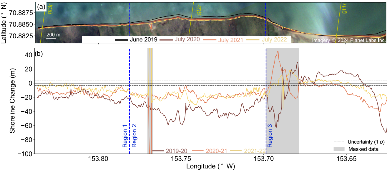
Figure 3. (a) Shorelines derived from Planet images, overlain on imagery from 07/25/2020. The locations of the three ICESat-2 ground track are also shown. (b) North-south shoreline change calculated between successive years. Areas where there was an ambiguous land/water boundary are masked out (shaded areas) and excluded from analysis. The boundaries of the three region shown in Fig. 1 are shown as dashed lines.
