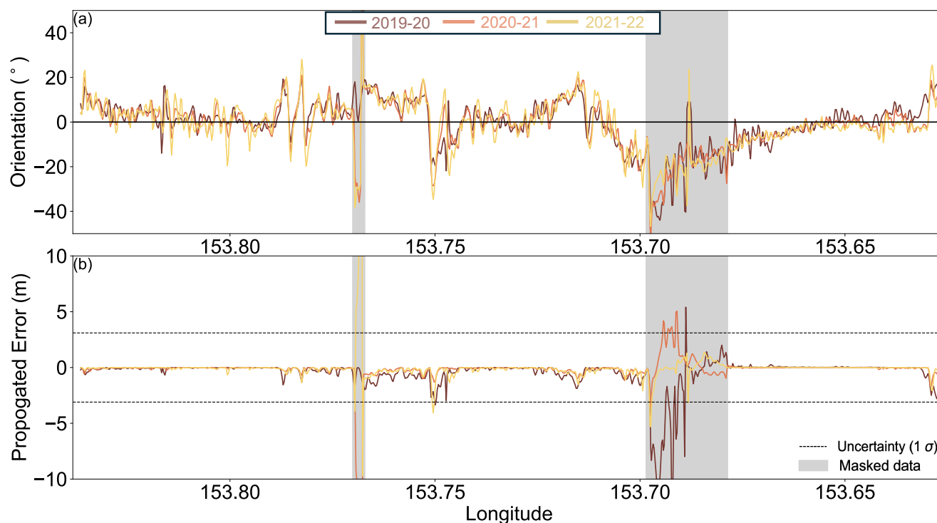
Figure A2. (a) Local orientation of the shoreline averaged between consecutive years, measured clockwise from north. (b) The relative error calculated from Equation 2 based on these orientations scaled by the measured shoreline change (Fig. 3b). The majority of this error falls well below our uncertainty threshold estimated in Section 2.3 (plotted as a dashed line).
