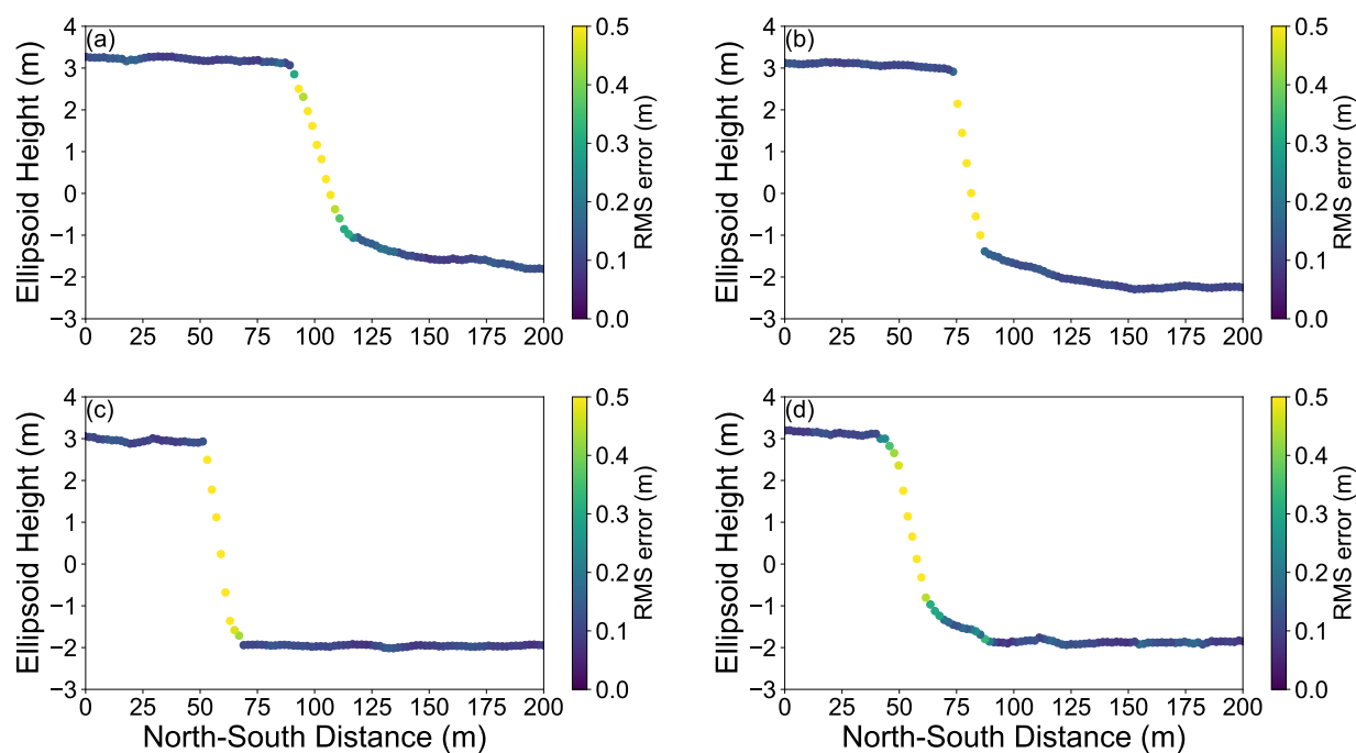
Figure A4. RMS error between our SlideRule-derived elevations and the source ATL03 photon information for ground track 3r for (a) 7 April 2019; (b) 4 January 2020; (c) 2 July 2021; (d) 31 December 2021
