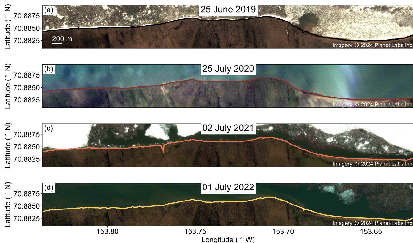
Figure 2. Planet Labs imagery (Planet Team, 2023) used to estimate shoreline positions. Shorelines delineated using Otsu thresholding are overlain and show good agreement with the visible land-water boundary.
