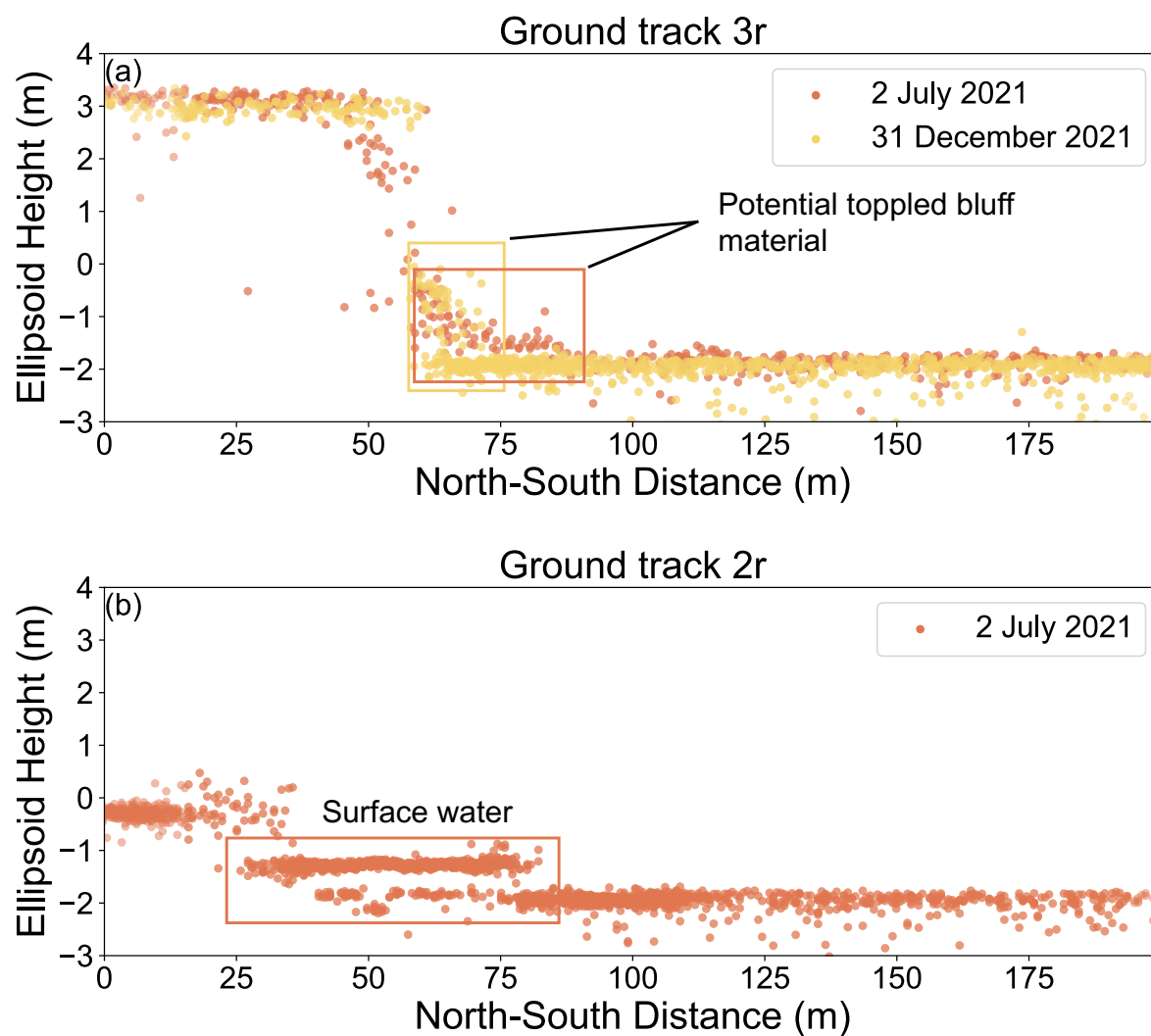
Figure 7. ICESat-2 ATL03 photon data show small-scale features, including (a) returns over what may be a toppled block material at the base of the bluff at ground track 3r and (b) Surface ponding in the drained lake basin at ground track 2r.
