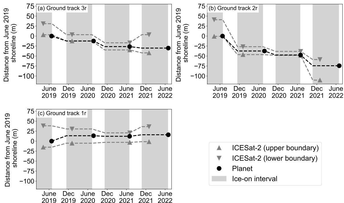
Figure 4. Time series of the position of upper and lower boundaries and coastal boundaries from ICESat-2 and the land-water boundary derived from Planet. Positions are given with respect to the location of Planet-derived shoreline from 25 June 2019. Ice-on intervals are shaded.
