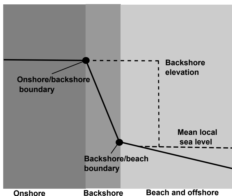
Figure A3. Illustration of the boundaries and elevation estimates described in Section 2.4
