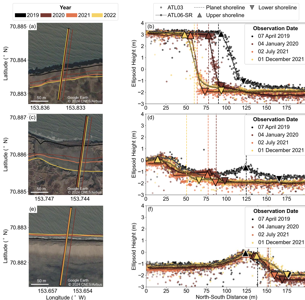
Figure 6. (a), (c), (e): Detailed view of the ICESat-2 sampling location from 2018 Google Earth Imagery for (a) ground track 3r; (c) ground track 2r and (e) ground track 1r. The location of the Planet shoreline and corresponding ICESat-2 pass for each year is shown. (b), (d), (f): ATL03 photon clouds from each ICESat-2 pass, with the SlideRule-derived (ATL06-SR) elevation profile overlain for (b) ground track 3r; (d) ground track 2r; and (f) ground track 1r. The estimated location of the upper and lower shoreline boundary for each date is marked, along with the north-south locations of the Planet-derived shorelines. The colors follow the same legend as (a), (c), and (e).
